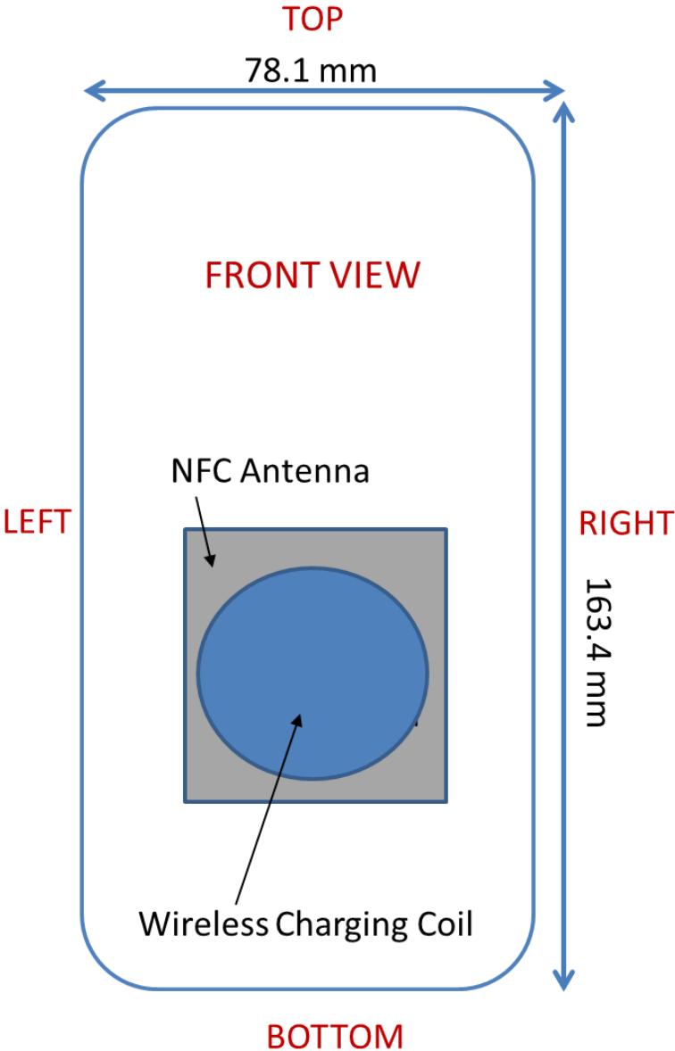
Figure H-2 NFC Antenna Locations
