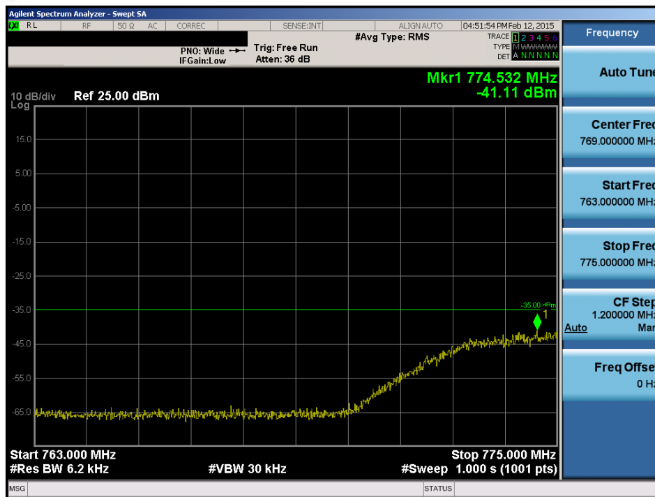
Plot 6-40. Lower Emission Mask Plot (Band 13 - 10.0MHz QPSK - RB Size 50)
