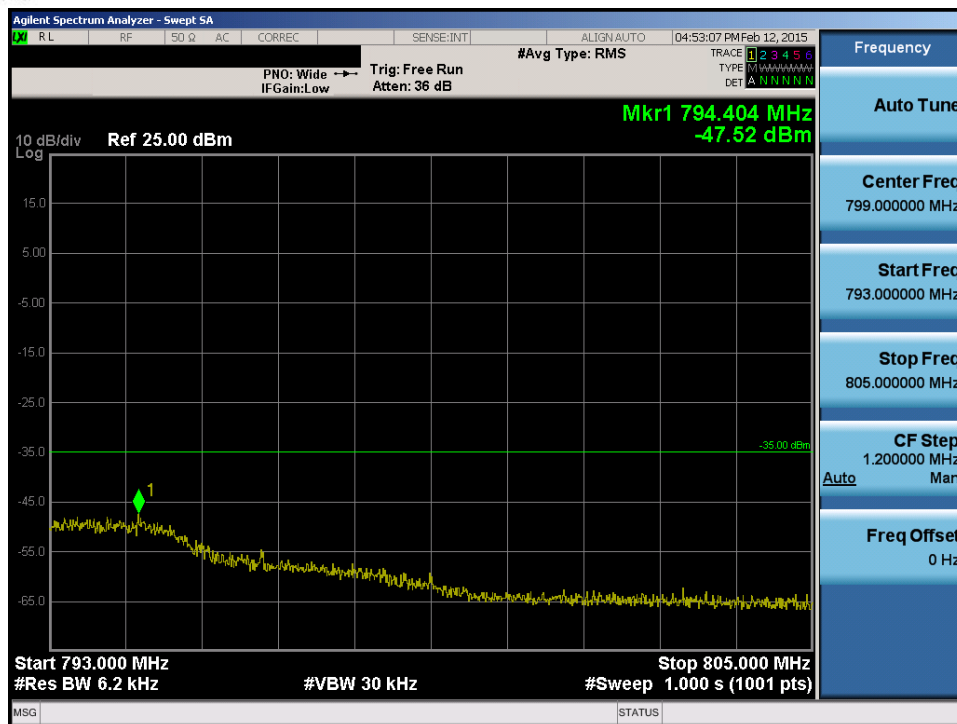
Plot 6-38. Upper Emission Mask Plot (Band 13 – 5.0MHz QPSK – RB Size 25)
