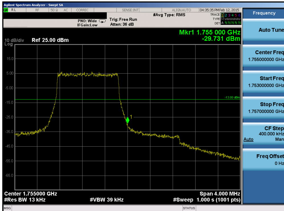
Plot 6-45. Upper Band Edge Plot (Band 4 – 1.4MHz QPSK – RB Size 6)
