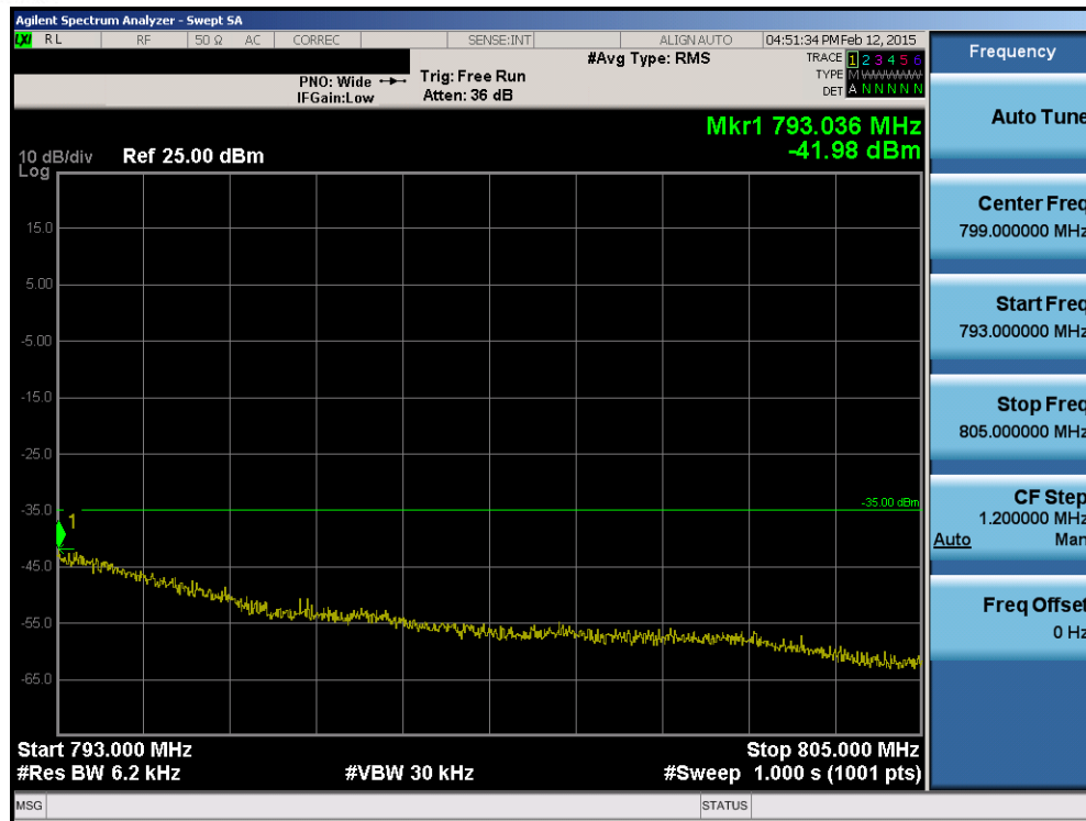
Plot 6-42. Upper Emission Mask Plot (Band 13 – 10.0MHz QPSK – RB Size 50)
