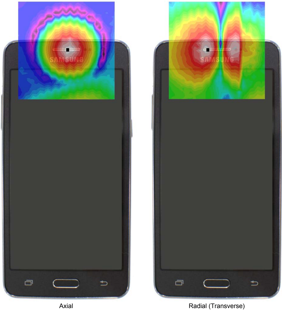
Figure 12-3 T-Coil Scan Overlay Magnetic Field Distributions
