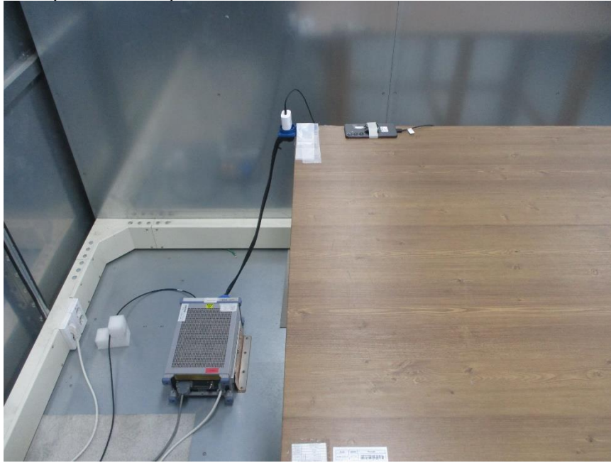
AC LINE CONDUCTED FRONT TEST PHOTO WPT(Test Case 5)
