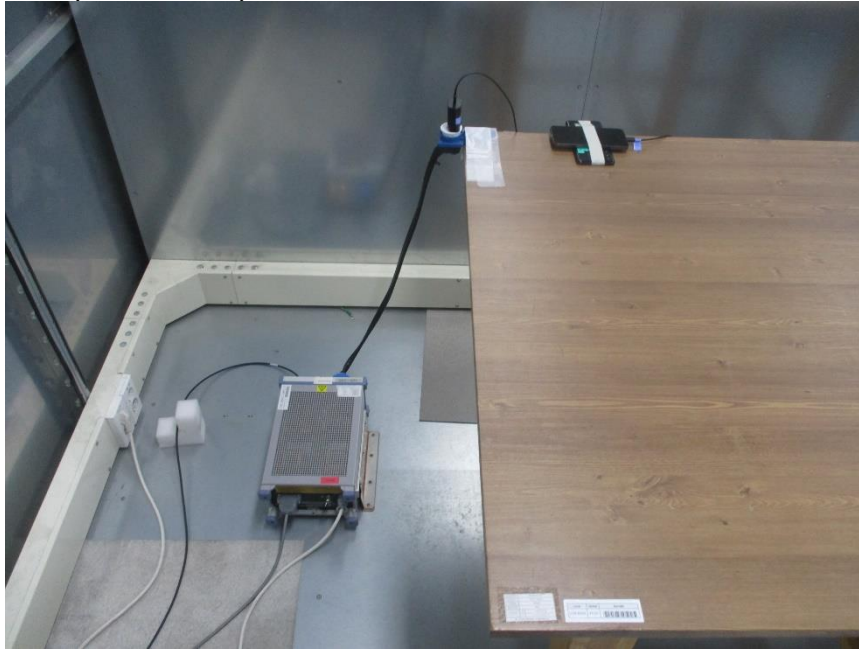
AC LINE CONDUCTED FRONT TEST PHOTO WPT(Test Case 4)
