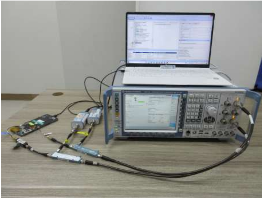
Test setup photo-3 (7-1(b) WLAN SAR1 vs SAR2 (DBS)/ WLAN Ant Switch)
