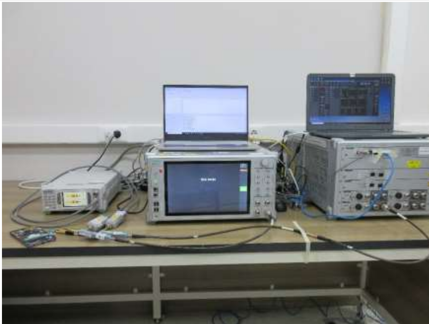
Test setup photo 10 - TC 14
