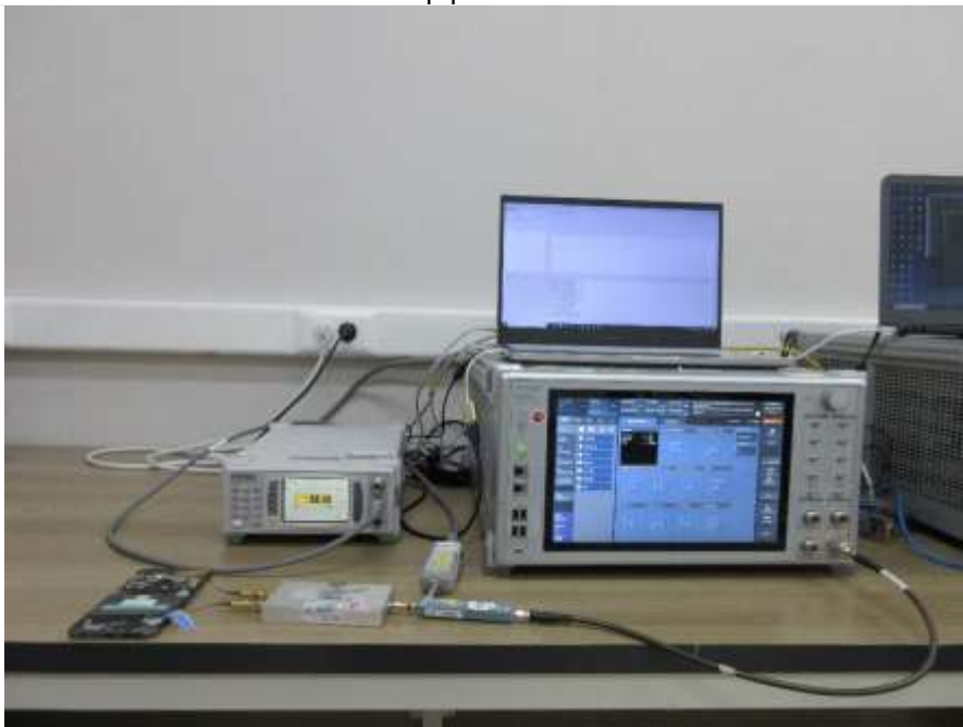
Test setup photo 08 - TC 12
