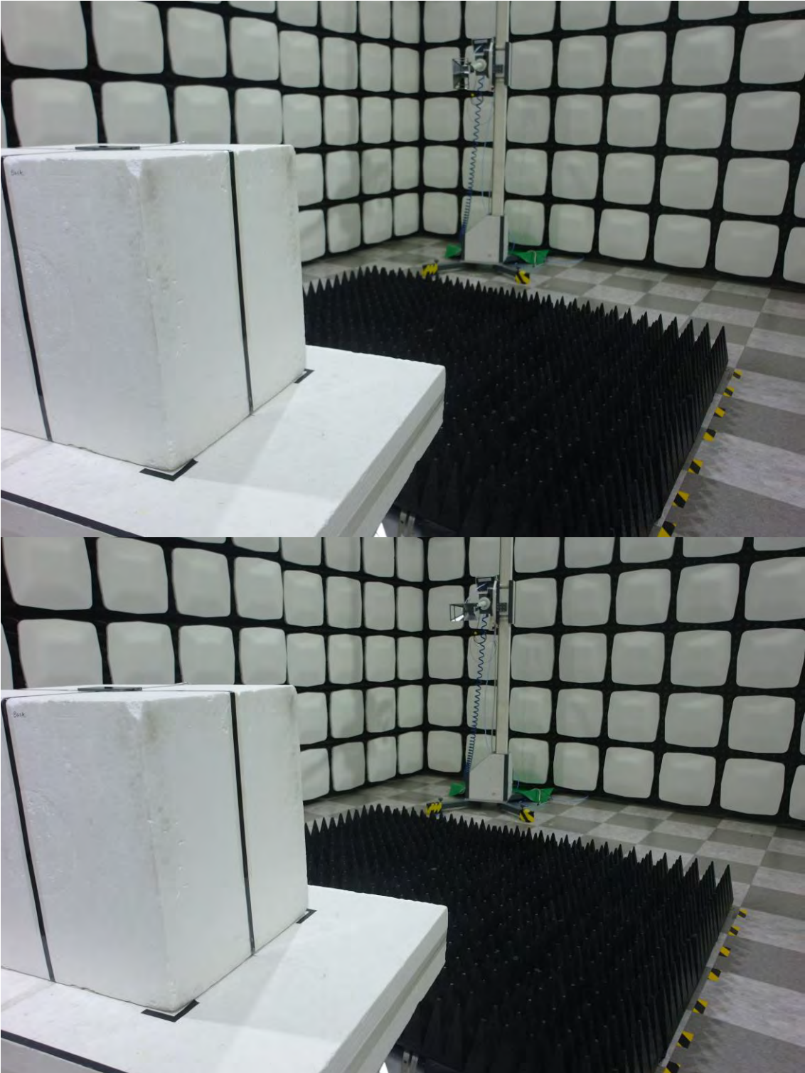
Radiated spurious emissions & Restricted Band Edge (Above 1 GHz)
