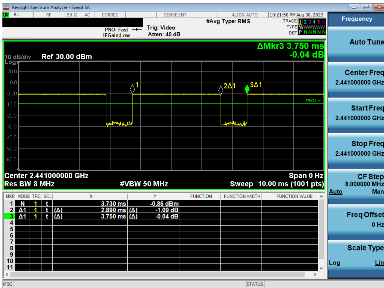
Figure 10-9 Bluetooth MIMO Transmission Plot
