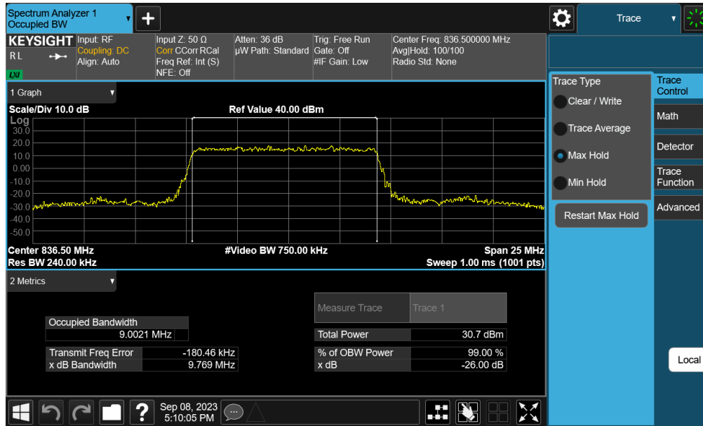
Plot 7-42. Occupied Bandwidth Plot (NR Band n5 - 10MHz \pi/2 BPSK - Full RB - Ant 6)
