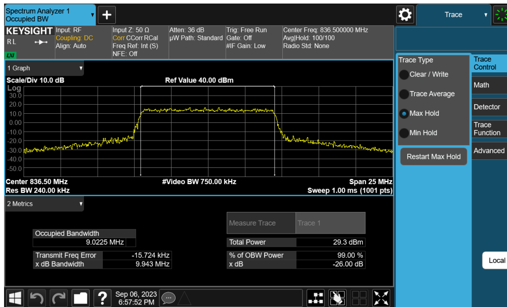
Plot 7-29. Occupied Bandwidth Plot (LTE Band 26/5 - 10MHz 16-QAM - Full RB - Ant 6)
