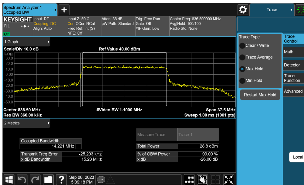
Plot 7-41. Occupied Bandwidth Plot (NR Band n5 - 15MHz 16-QAM - Full RB - Ant 6)
