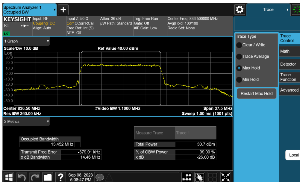
Plot 7-39. Occupied Bandwidth Plot (NR Band n5 - 15MHz \pi/2 BPSK - Full RB - Ant 6)
