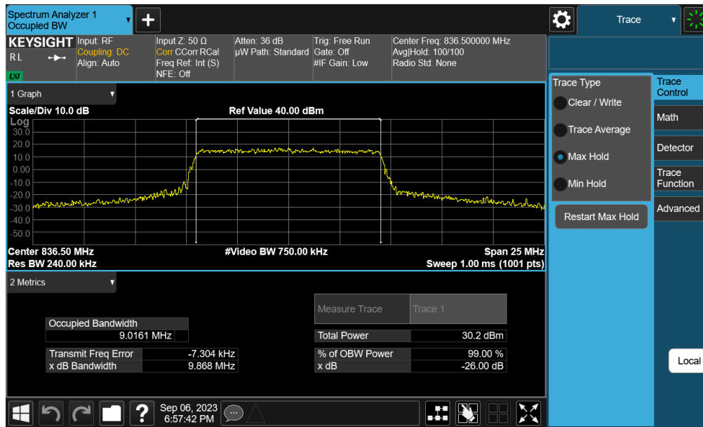
Plot 7-28. Occupied Bandwidth Plot (LTE Band 26/5 - 10MHz QPSK - Full RB - Ant 6)
