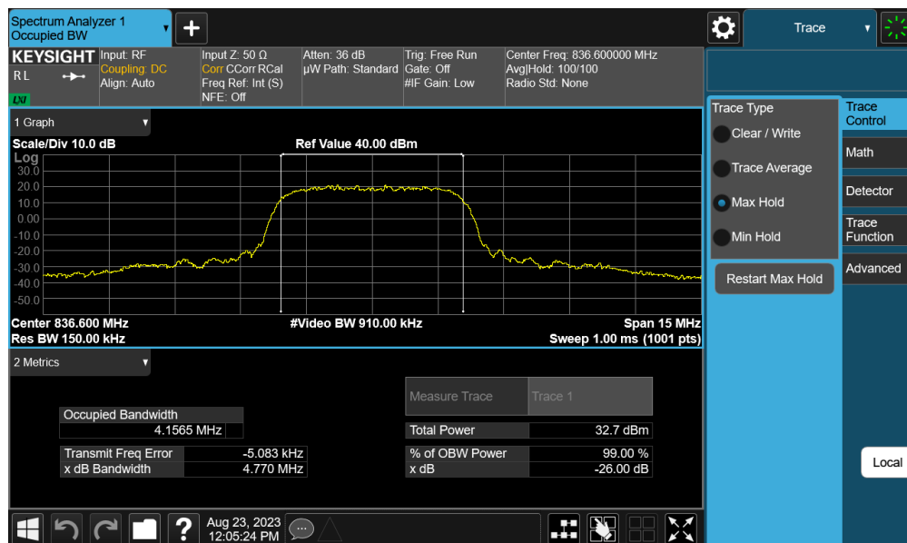
Plot 7-25. Occupied Bandwidth Plot (WCDMA, Ch. 4183 – Ant 0)
