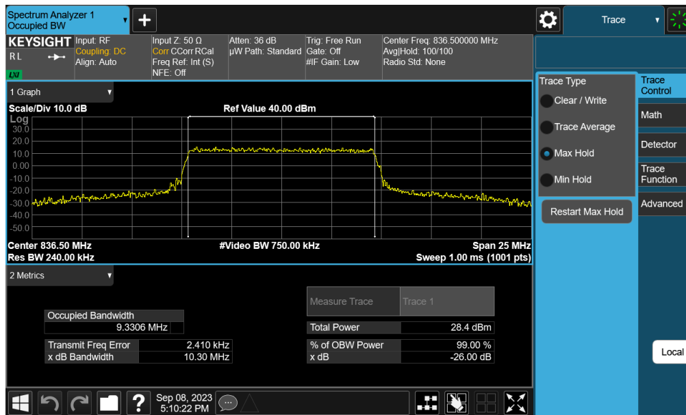
Plot 7-43. Occupied Bandwidth Plot (NR Band n5 - 10MHz QPSK - Full RB - Ant 6)
