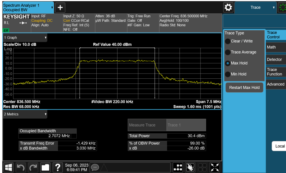
Plot 7-32. Occupied Bandwidth Plot (LTE Band 26/5 - 3MHz QPSK - Full RB - Ant 6)
