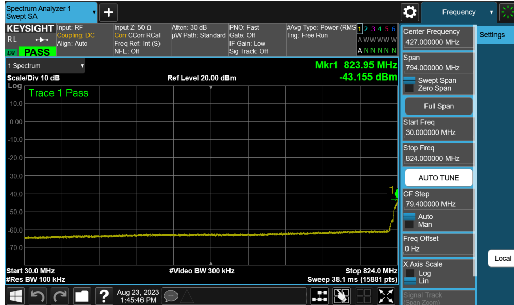
Plot 7-51. Conducted Spurious Plot (LTE Band 26/5 - 10MHz QPSK - 1 RB - Mid Channel – Ant 0)
