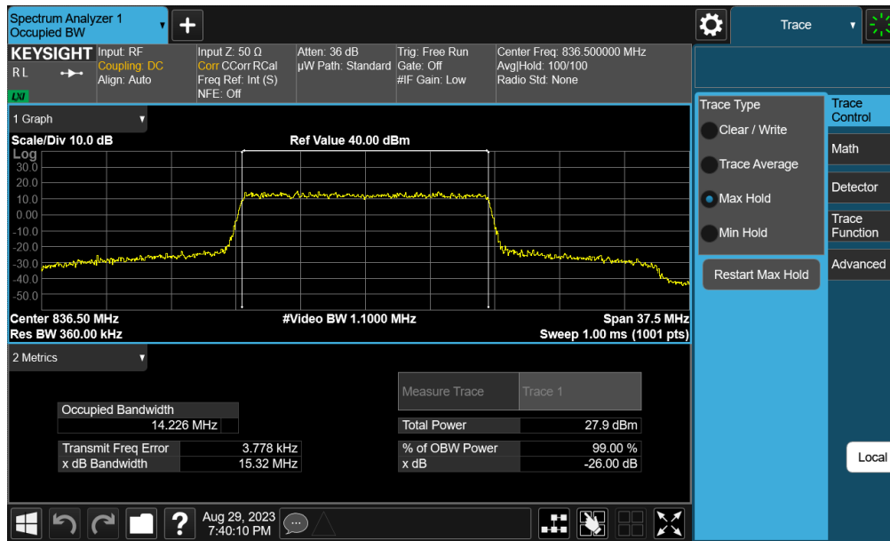
Plot 7-15. Occupied Bandwidth Plot (NR Band n5 - 15MHz QPSK - Full RB - Ant 0)
