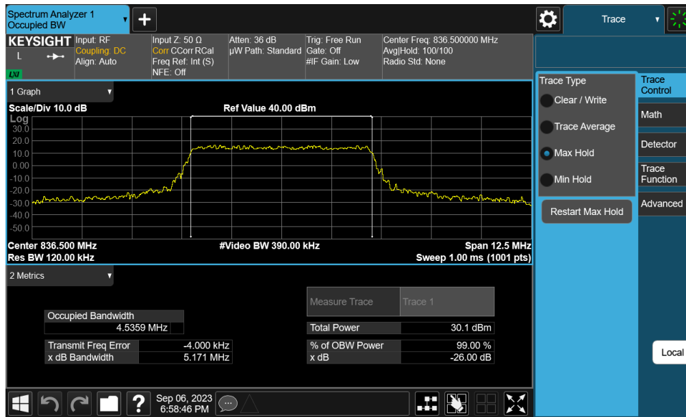
Plot 7-30. Occupied Bandwidth Plot (LTE Band 26/5 - 5MHz QPSK - Full RB - Ant 6)
