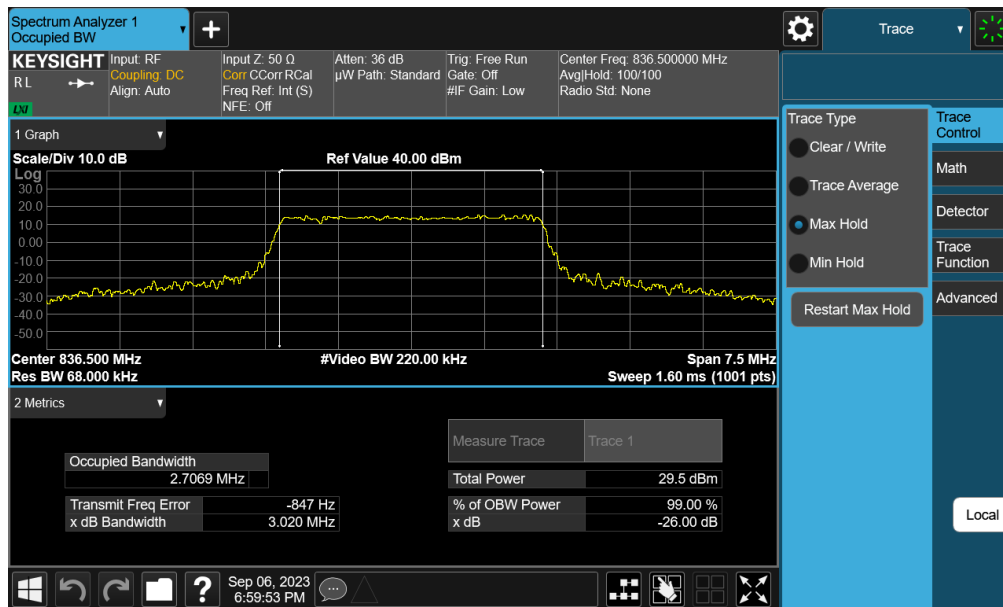
Plot 7-33. Occupied Bandwidth Plot (LTE Band 26/5 - 3MHz 16-QAM - Full RB - Ant 6)
