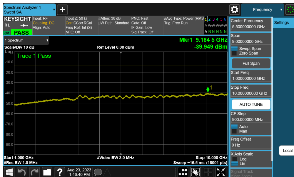
Plot 7-53. Conducted Spurious Plot (LTE Band 26/5 - 10MHz QPSK - 1 RB - Mid Channel – Ant 0)
