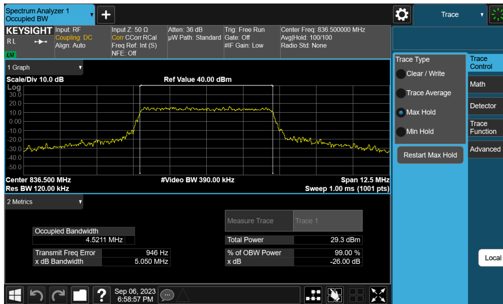
Plot 7-31. Occupied Bandwidth Plot (LTE Band 26/5 - 5MHz 16-QAM - Full RB - Ant 6)
