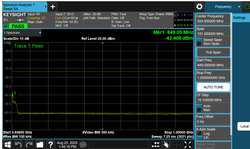
Plot 7-52. Conducted Spurious Plot (LTE Band 26/5 - 10MHz QPSK - 1 RB - Mid Channel – Ant 0)
