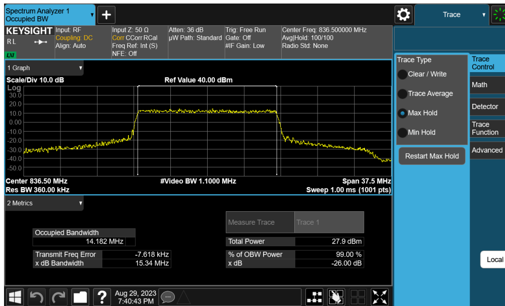
Plot 7-16. Occupied Bandwidth Plot (NR Band n5 - 15MHz 16-QAM - Full RB - Ant 0)
