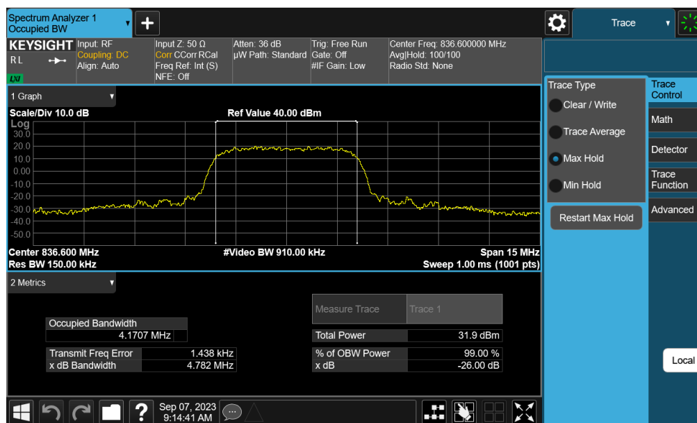
Plot 7-50. Occupied Bandwidth Plot (WCDMA, Ch. 4183 – Ant 6)
