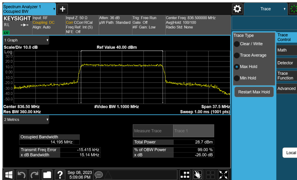
Plot 7-40. Occupied Bandwidth Plot (NR Band n5 - 15MHz QPSK - Full RB - Ant 6)
