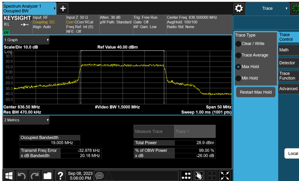
Plot 7-38. Occupied Bandwidth Plot (NR Band n5 - 20MHz 16-QAM - Full RB - Ant 6)
