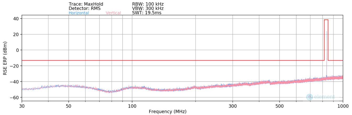
Plot 7-97. Radiated Spurious Plot Below 1GHz (NR Band n5 – Ant 0)
