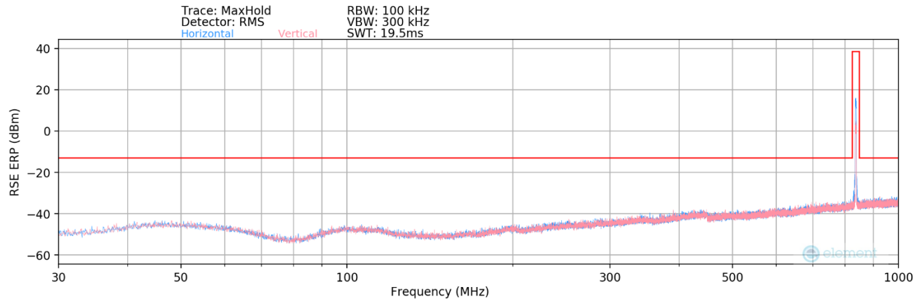
Plot 7-101. Radiated Spurious Plot Below 1GHz (WCDMA Cell – Ant 6)
