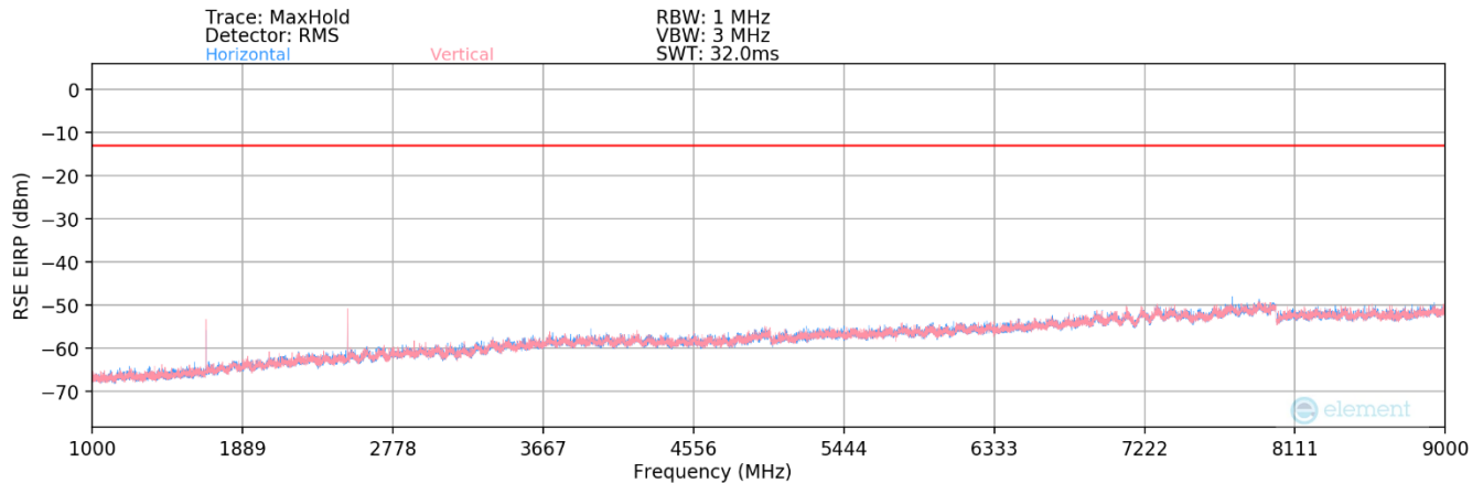
Plot 7-100. Radiated Spurious Plot Above 1GHz (GPRS Cell – Ant 6)
