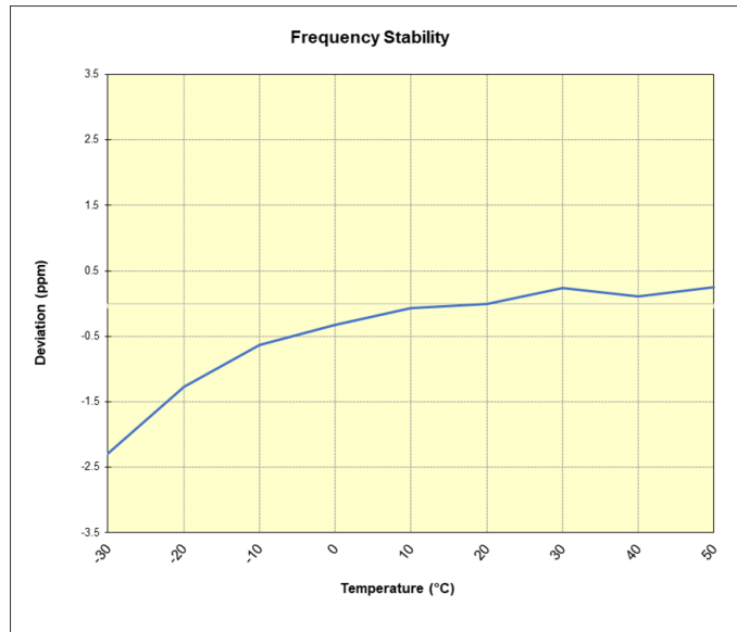
Plot 7-107. GSM/GPRS Cell Frequency Stability Chart
