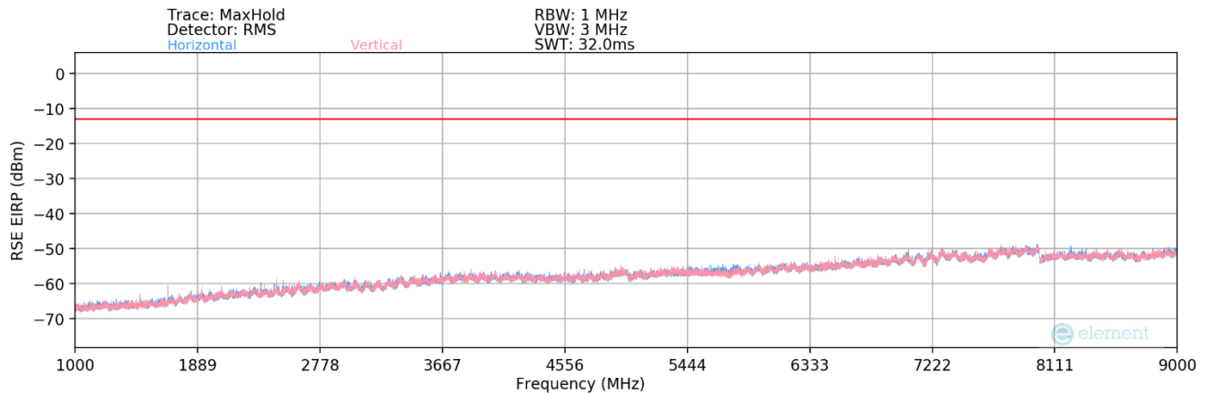
Plot 7-104. Radiated Spurious Plot Above 1GHz (LTE Band 26/5 – Ant 6)
