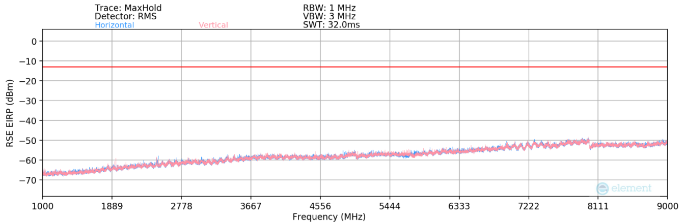
Plot 7-106. Radiated Spurious Plot Above 1GHz (NR Band n5 – Ant 6)
