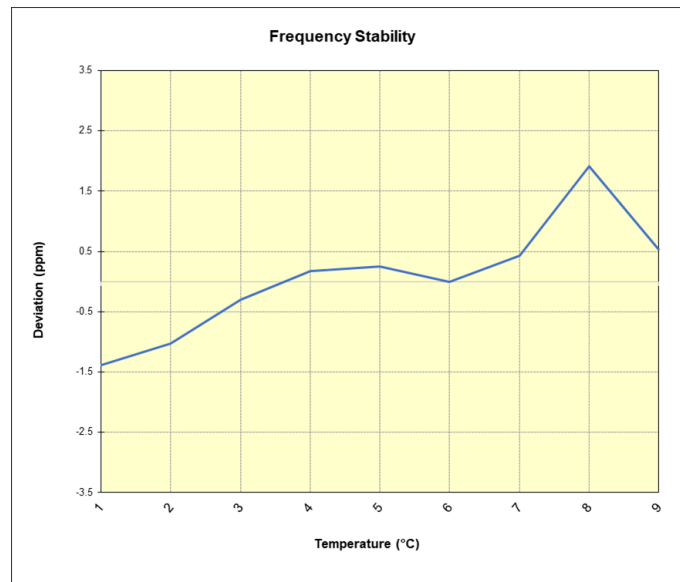
Plot 7-109. LTE Band 26/5 Frequency Stability Chart
