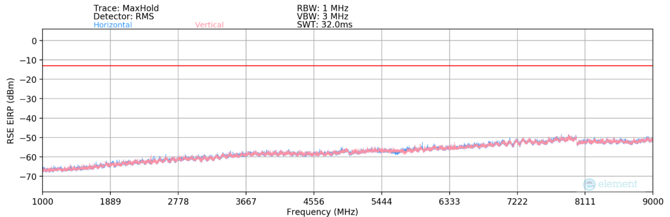
Plot 7-102. Radiated Spurious Plot Above 1GHz (WCDMA Cell – Ant 6)
