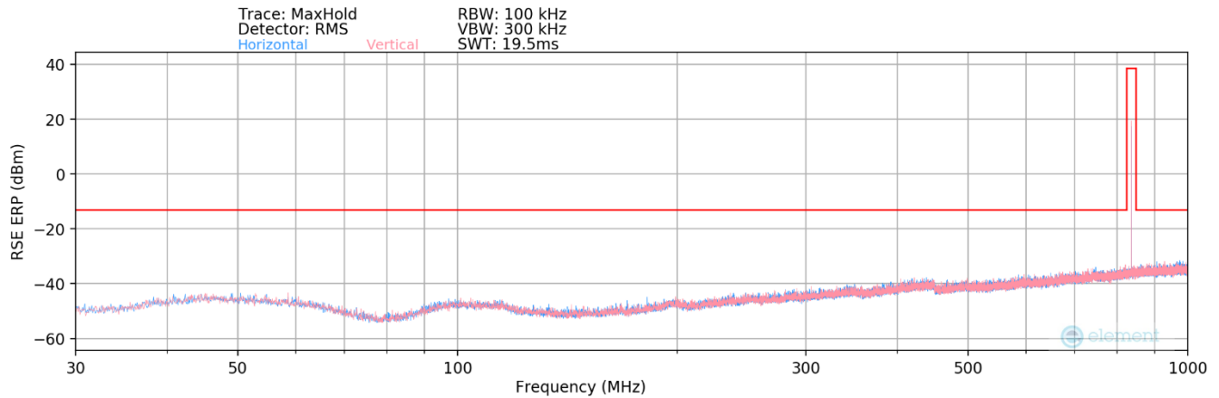
Plot 7-99. Radiated Spurious Plot Below 1GHz (GPRS Cell – Ant 6)
