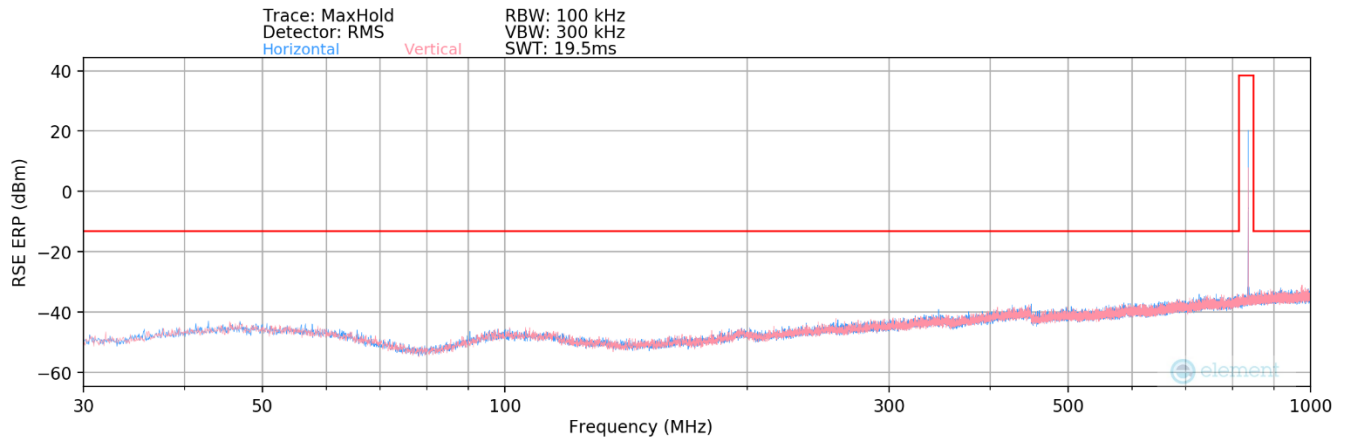
Plot 7-105. Radiated Spurious Plot Below 1GHz (NR Band n5 – Ant 6)
