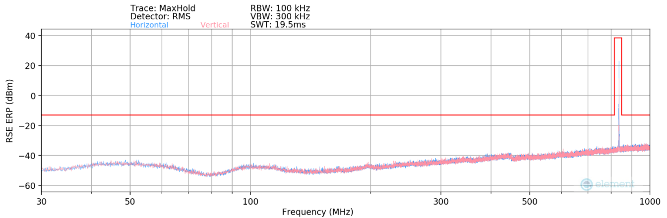
Plot 7-103. Radiated Spurious Plot Below 1GHz (LTE Band 26/5 – Ant 6)
