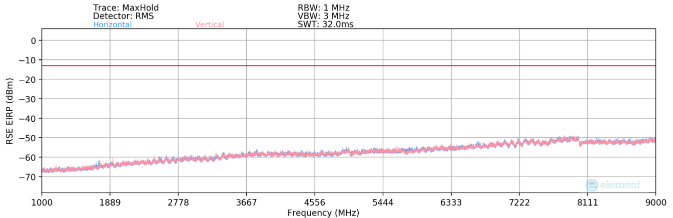
Plot 7-98. Radiated Spurious Plot Above 1GHz (NR Band n5 – Ant 0)
