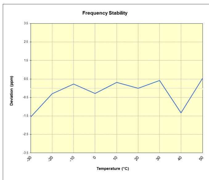
Plot 7-110. NR Band n5 Frequency Stability Chart
