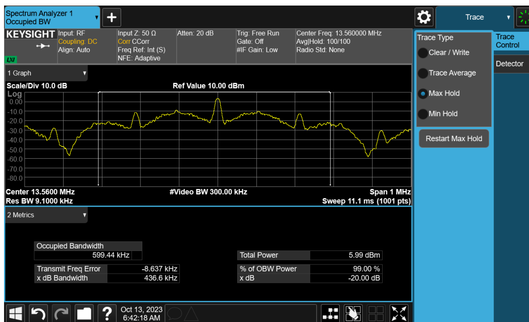
Figure 7-2. Occupied Bandwidth Plot
