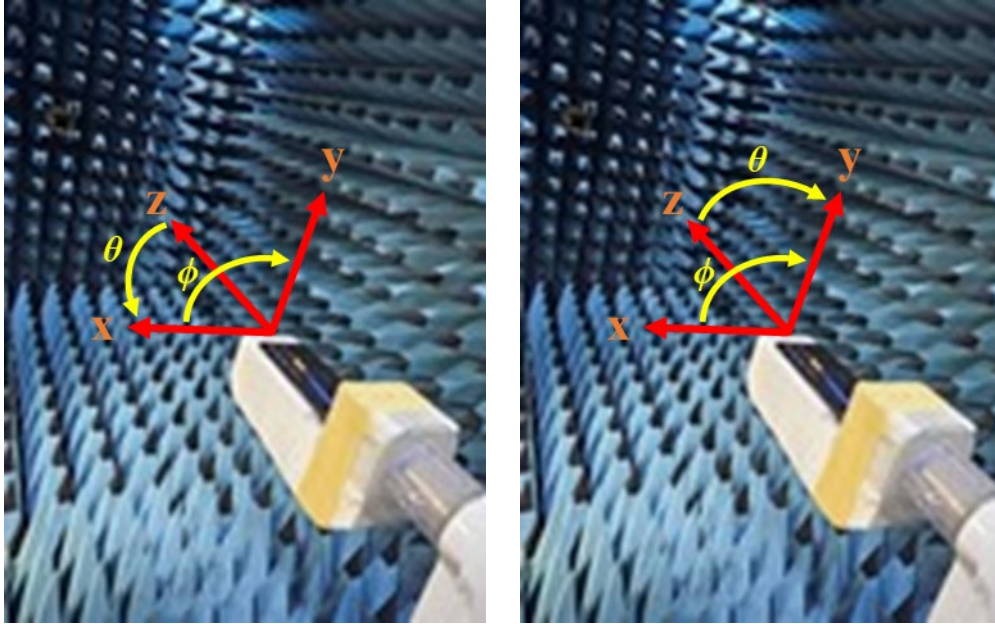
Figure 1: Geometry for SM-S928B for Radiation patterns.
