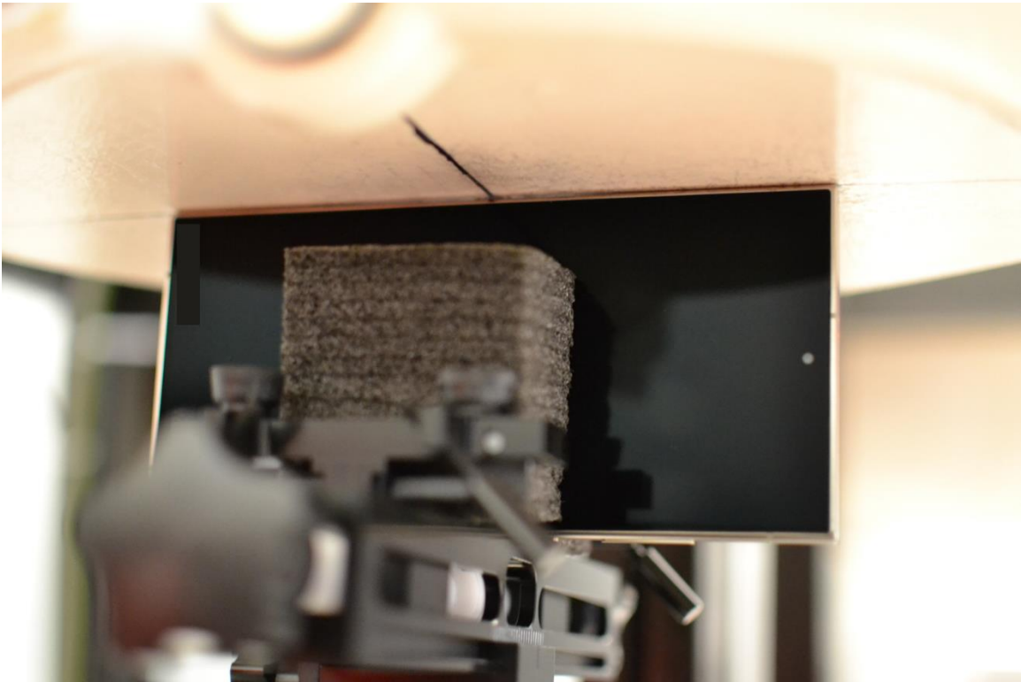
SAR Test Setup Photo 15 – Phablet, Left Edge at 0mm
