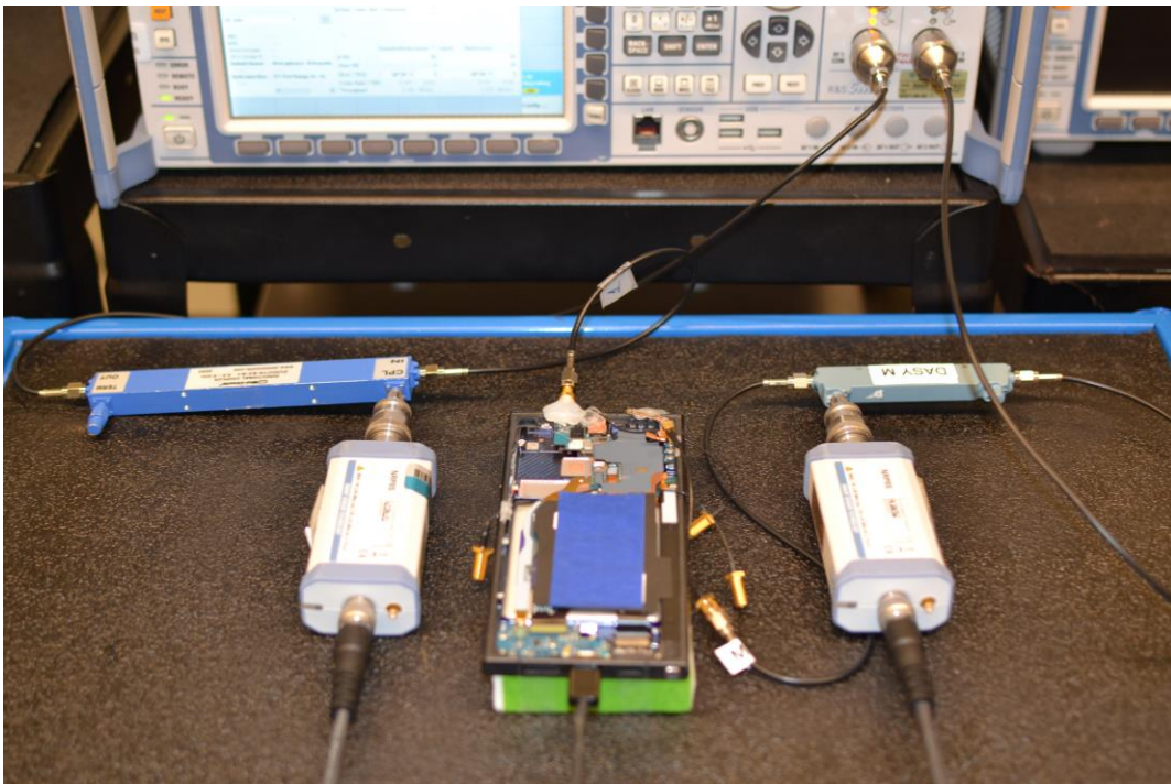
Test Setup Photo 8 – Radiated Power Test Setup (Figure 5-1f)
