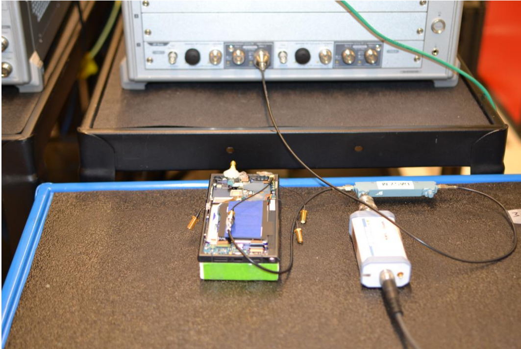
Test Setup Photo 3 – Conducted Test Setup (Figure 5-1a)
