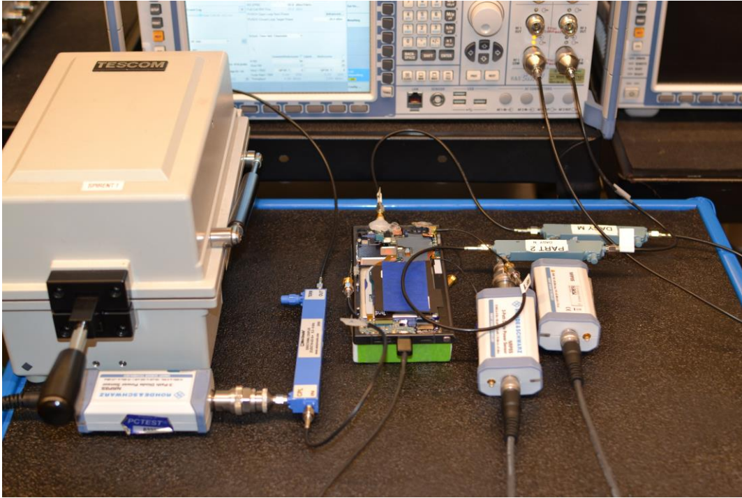
Test Setup Photo 7 – Conducted Test Setup (Figure 5-1e)
