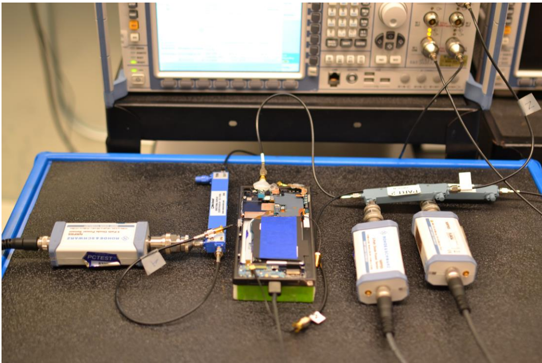
Test Setup Photo 6 – Conducted Test Setup (Figure 5-1d)
