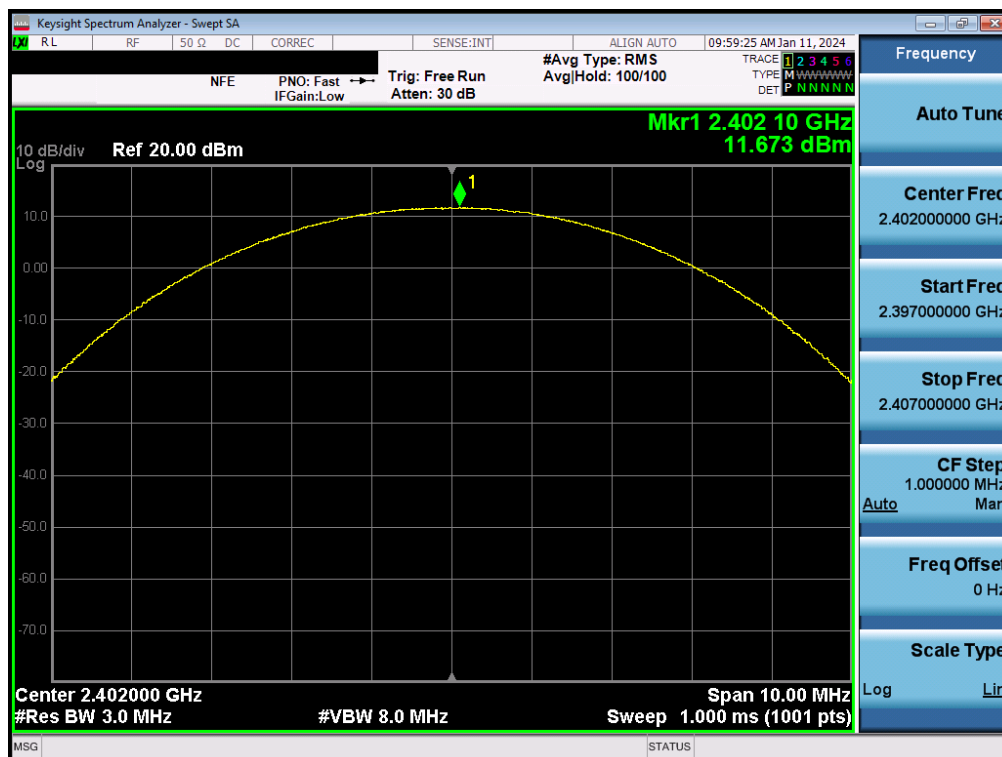
Plot 7-94. Peak Conducted Power (2Mbps – Ch. 0) – ANT2
