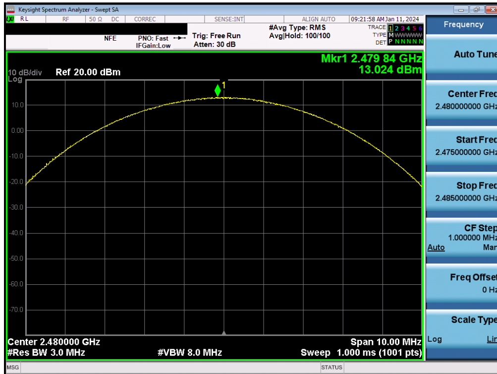
Plot 7-81. Peak Conducted Power (3Mbps – Ch. 78) – ANT1
