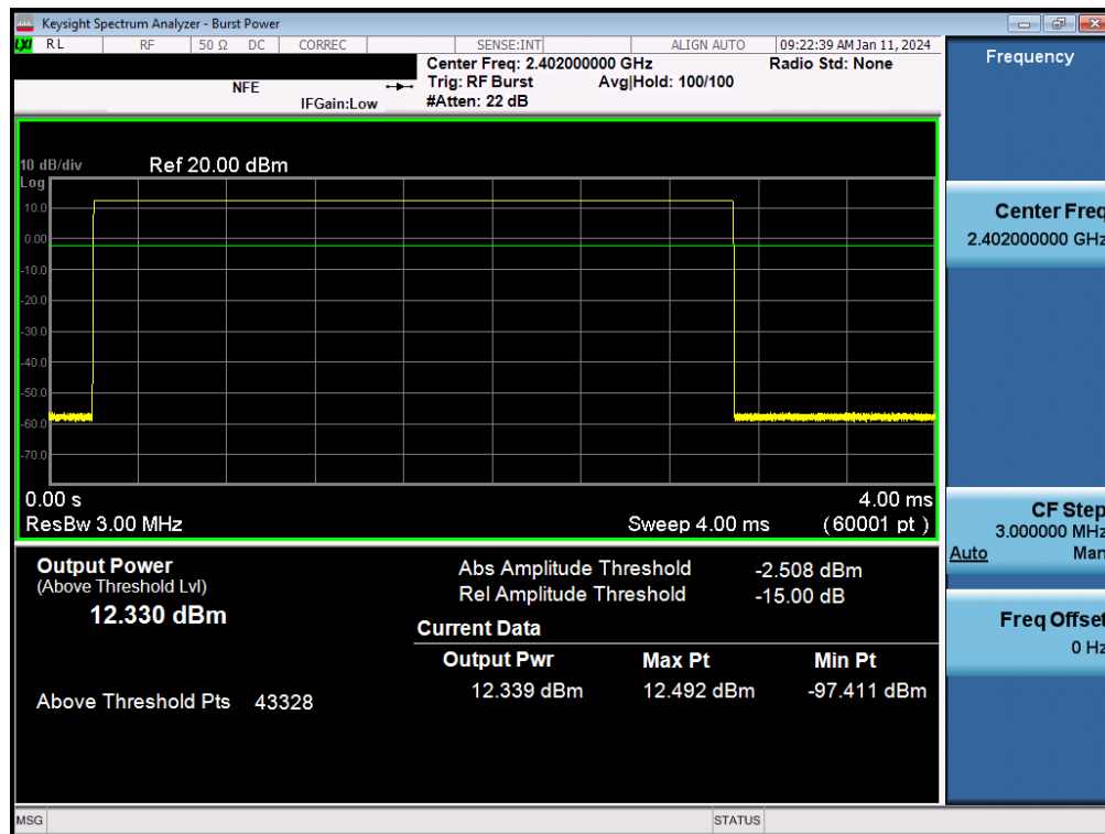
Plot 7-82. Average Conducted Power (1Mbps – Ch. 0) – ANT1
