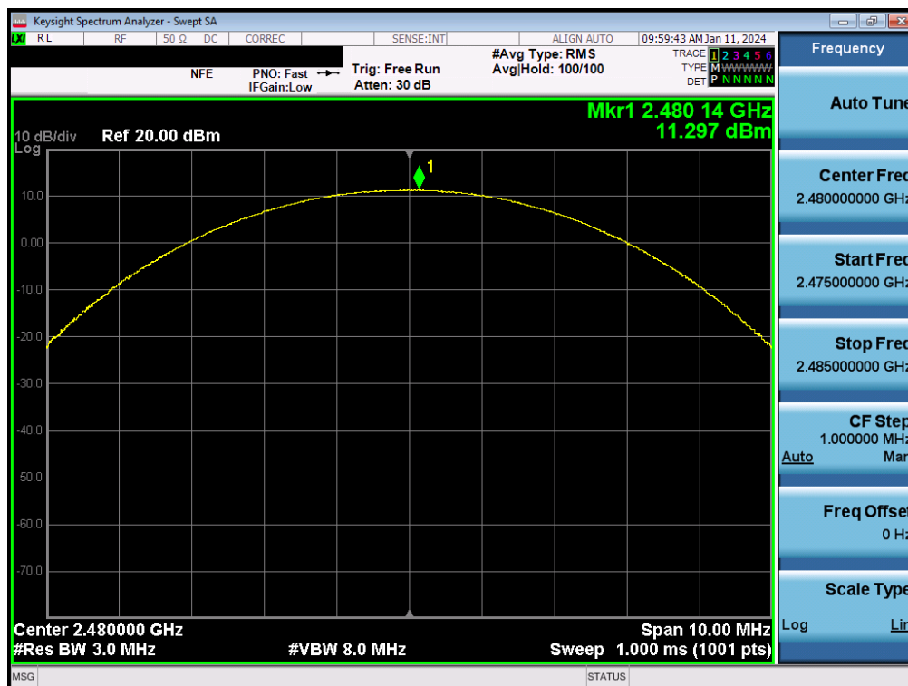
Plot 7-96. Peak Conducted Power (2Mbps – Ch. 78) – ANT2
