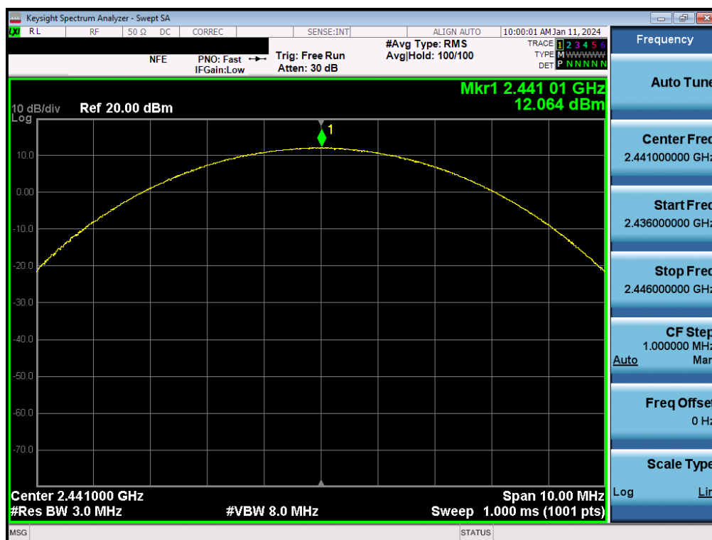
Plot 7-98. Peak Conducted Power (3Mbps – Ch. 39) – ANT2
