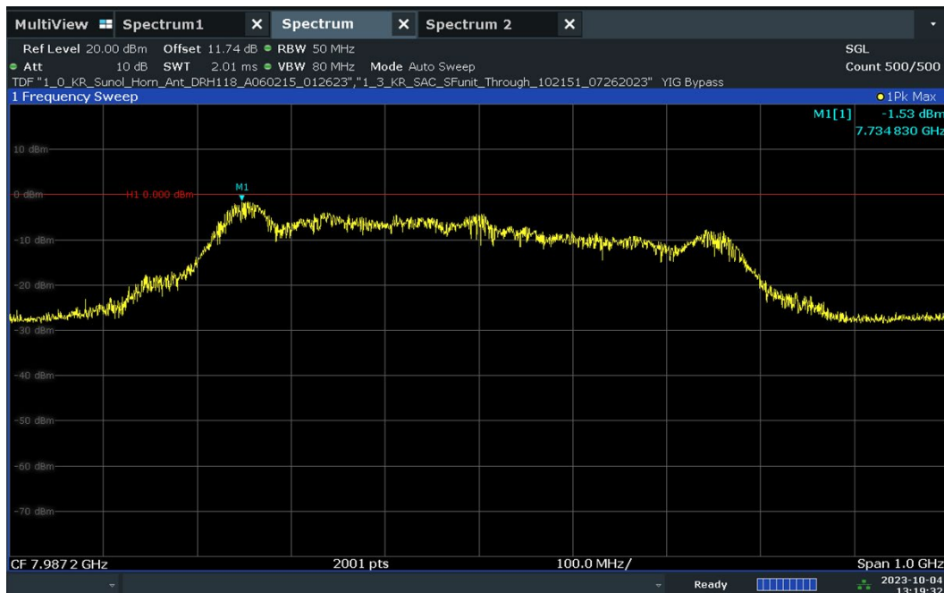
Plot 7-33. UWB Peak Power Measurement - CH.9 – BPRF
