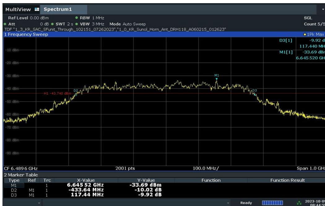
Plot 7-1. 10dBc Bandwidth – CH.5 - SP0 – Preamble 9
