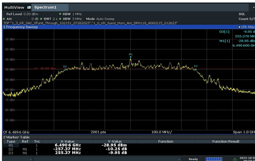
Plot 7-5. 10dBc Bandwidth – CH.5 – SP1 – Preamble 10
