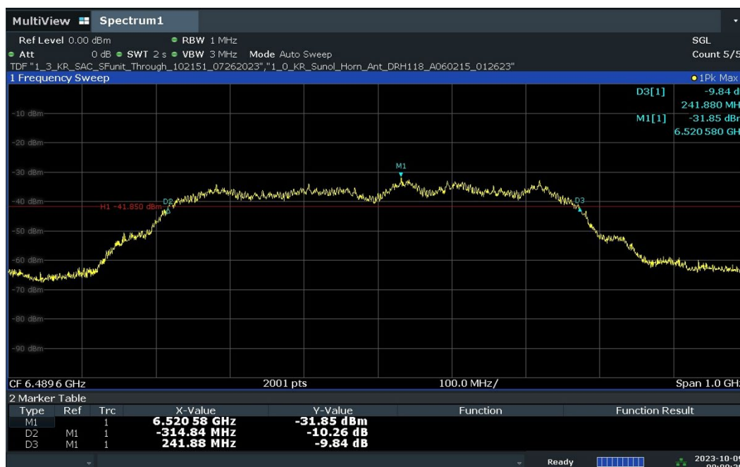
Plot 7-6. 10dBc Bandwidth – CH.5 – SP3 – Preamble 10
