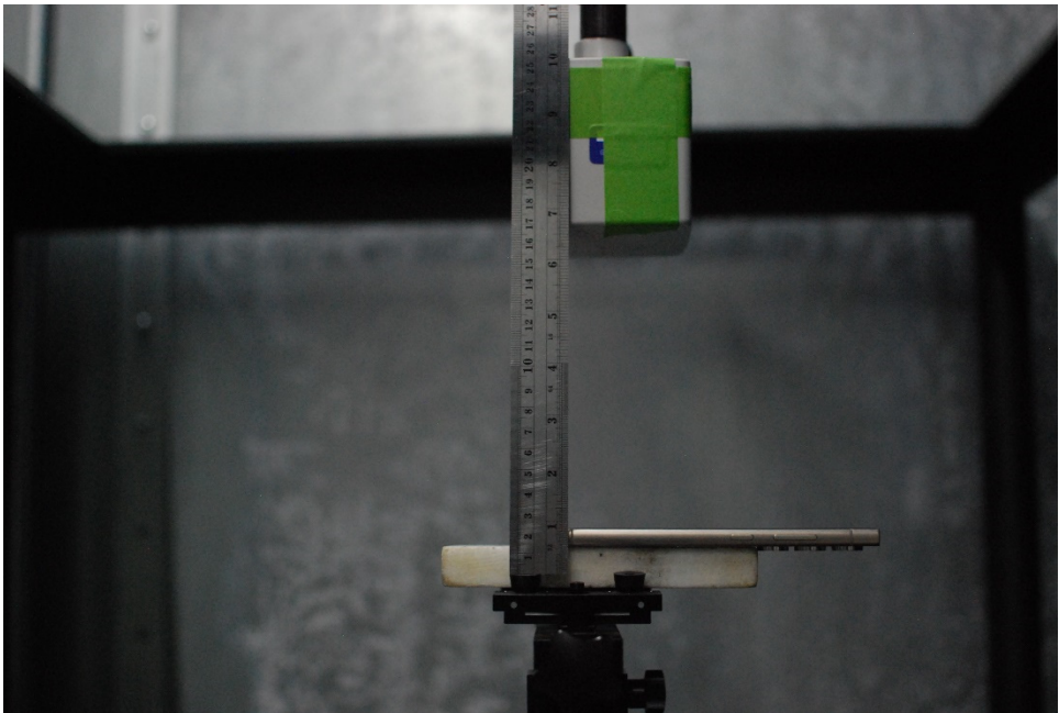
Test Setup Photo 3 H-field, Front side, 15cm
