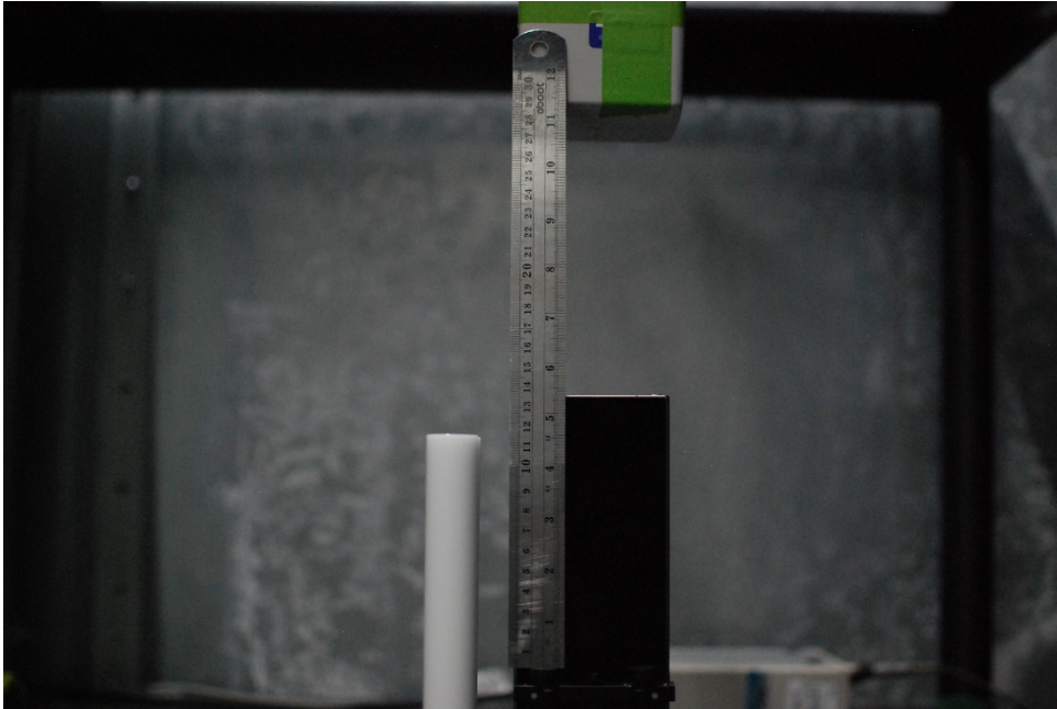
Test Setup Photo 5 H-field, Bottom edge, 15cm
