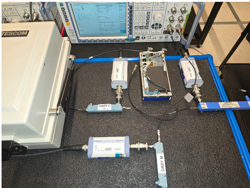
Test Setup Photo 10 – Conducted Test Setup (Figure 5-1g)
