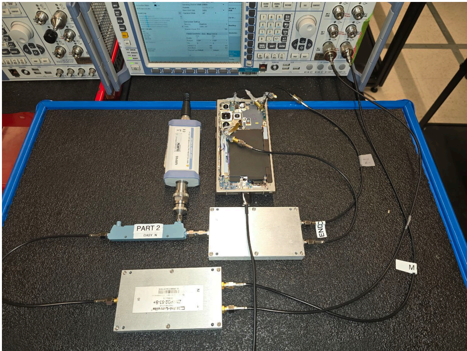
Test Setup Photo 7 – Conducted Test Setup (Figure 5-1f)
