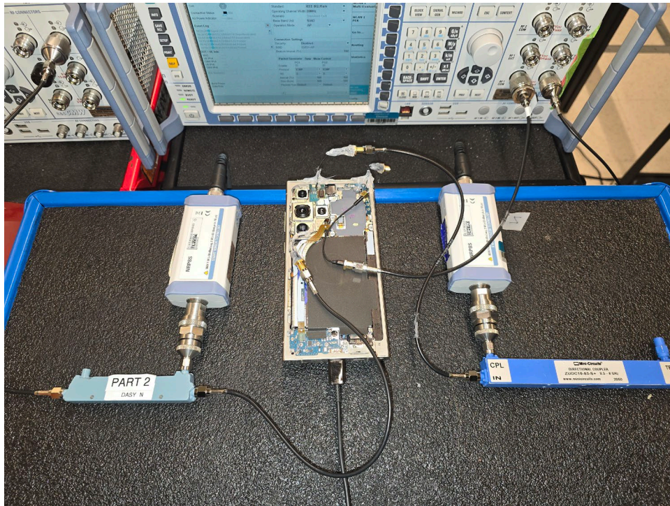
Test Setup Photo 9 – Conducted Test Setup (Figure 5-1e)
