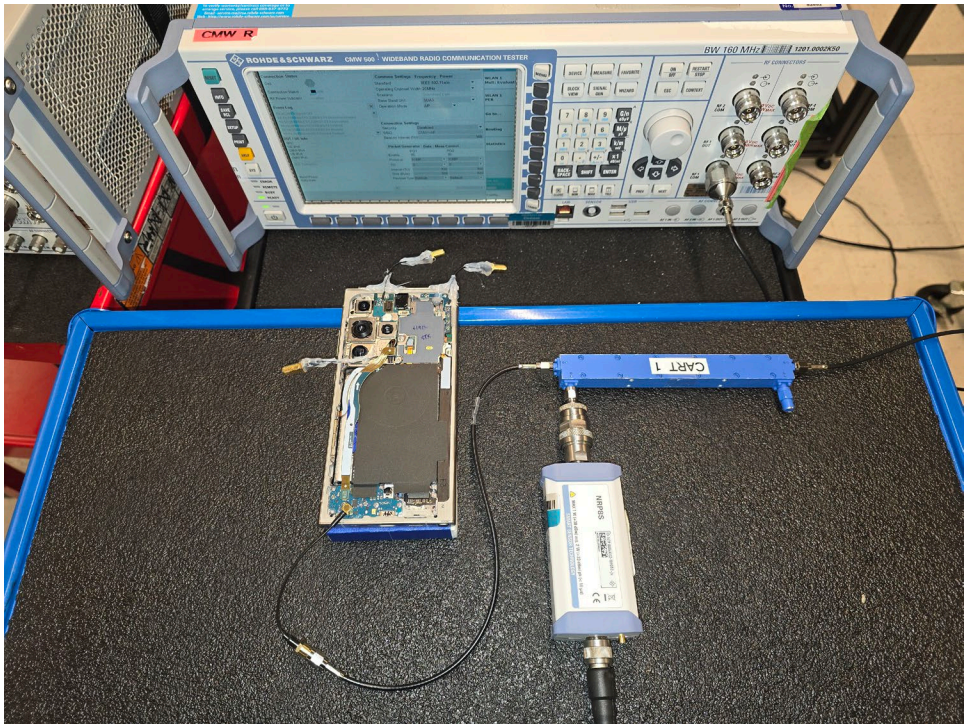
Test Setup Photo 1 – Conducted Test Setup (Figure 5-1a)
