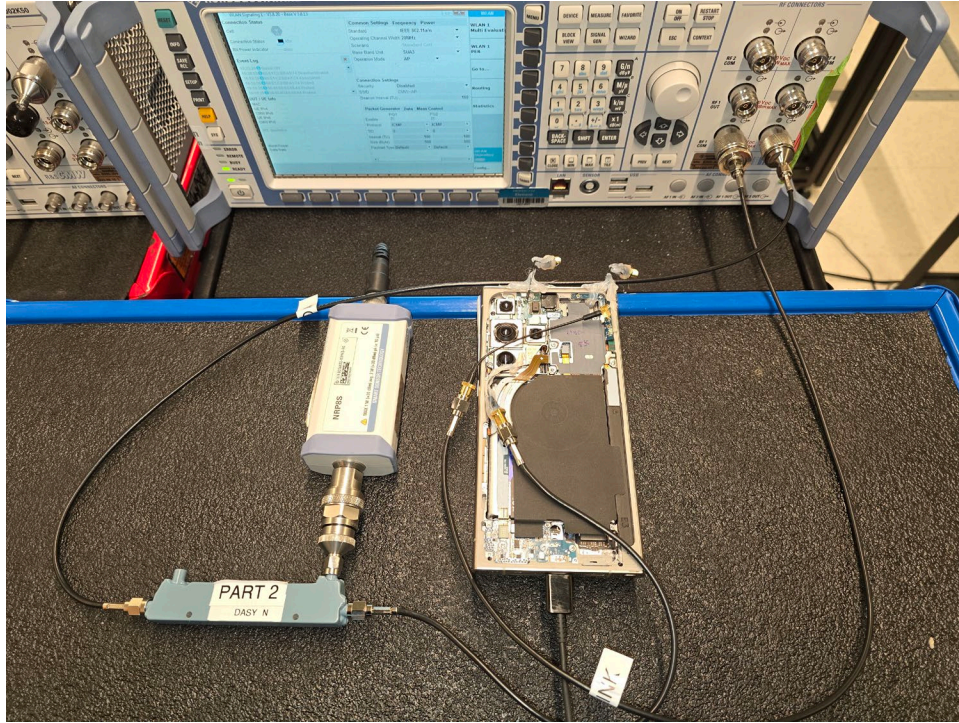
Test Setup Photo 5 – Conducted Test Setup (Figure 5-1d)
