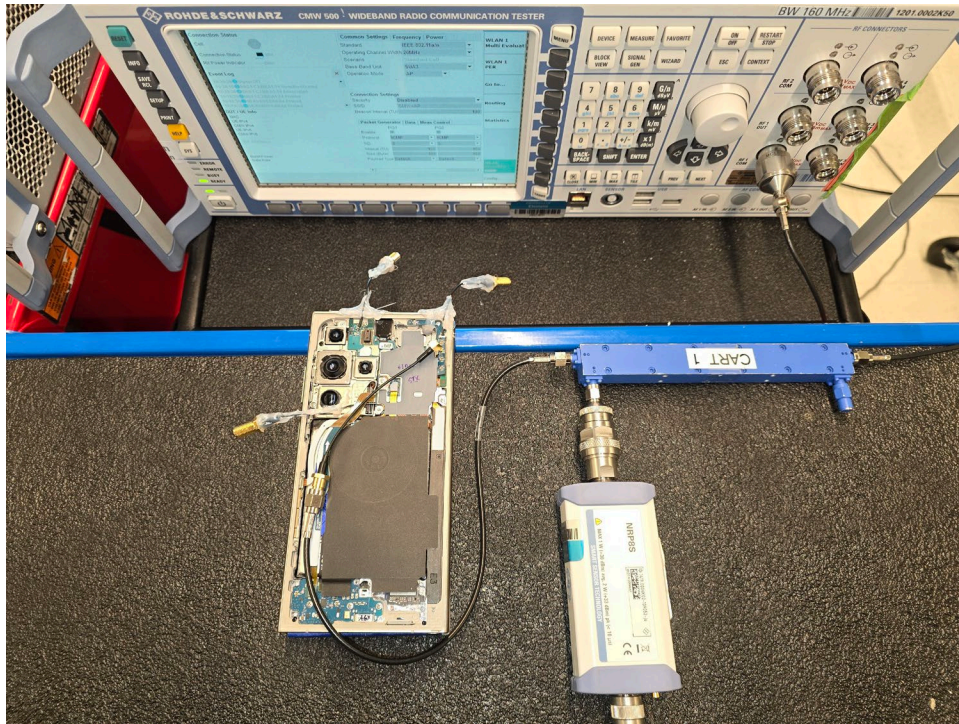
Test Setup Photo 3 – Conducted Test Setup (Figure 5-1a)
