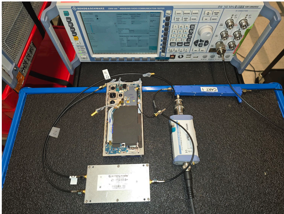
Test Setup Photo 6 – Conducted Test Setup (Figure 5-1b)
