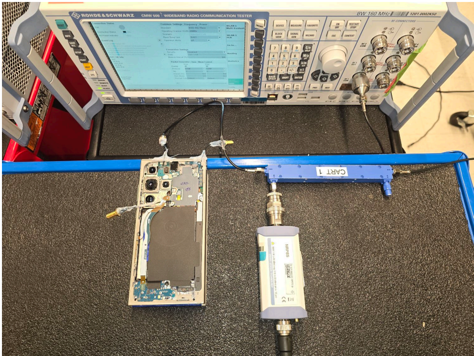
Test Setup Photo 2 – Conducted Test Setup (Figure 5-1a)
