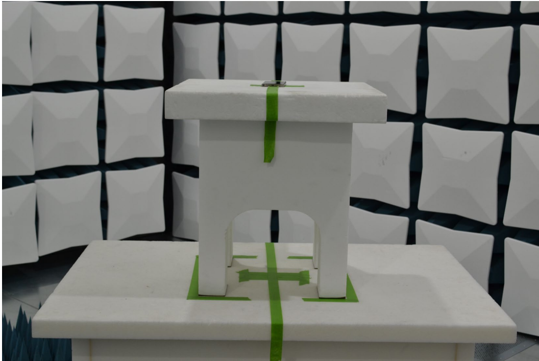
Figure 1. Test Setup – X Position – 1GHz-40GHz
