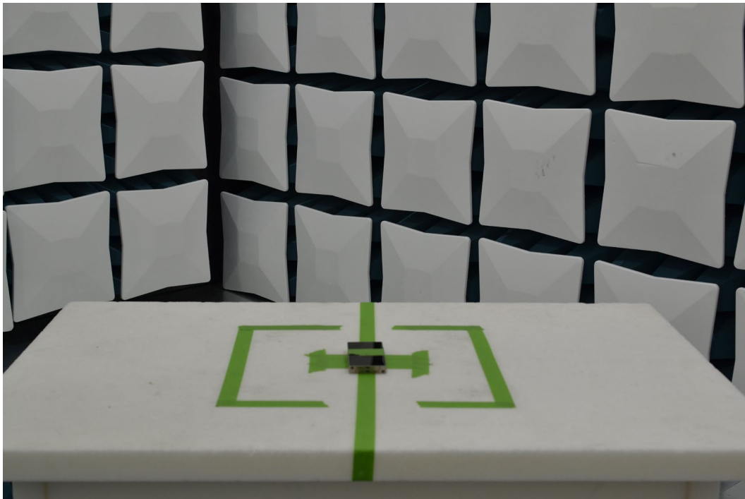
Figure 6. Test Setup – X Position – 30MHz-1GHz
