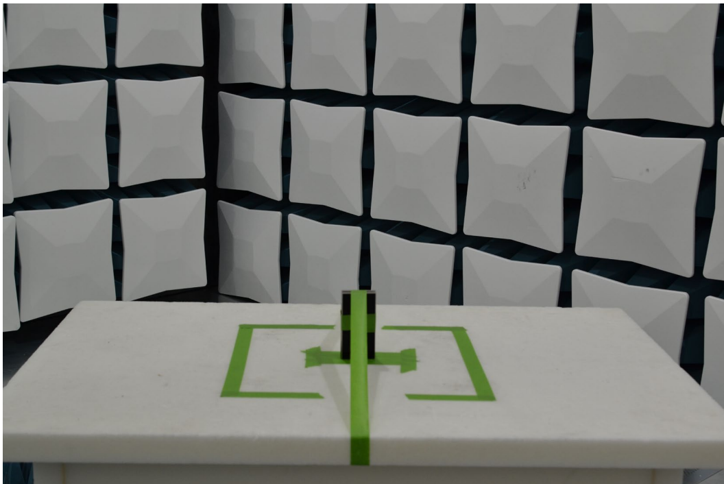
Figure 8. Test Setup – Z Position – 30MHz-1GHz
