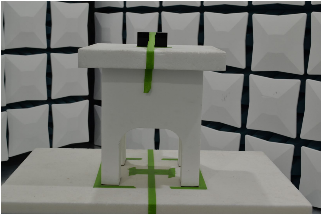
Figure 2. Test Setup – Y Position – 1GHz-40GHz
