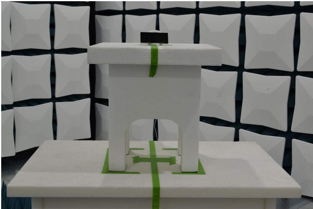
Figure 4. Test Setup – WCP Position – 1GHz-40GHz
