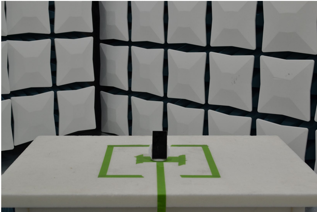
Figure 9. Test Setup – WCP Position – 30MHz-1GHz
