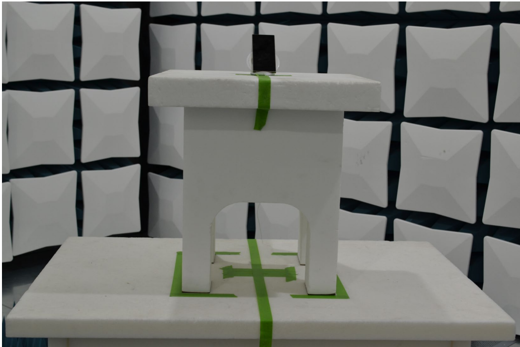
Figure 5. Test Setup – WCP Position – 1GHz-40GHz
