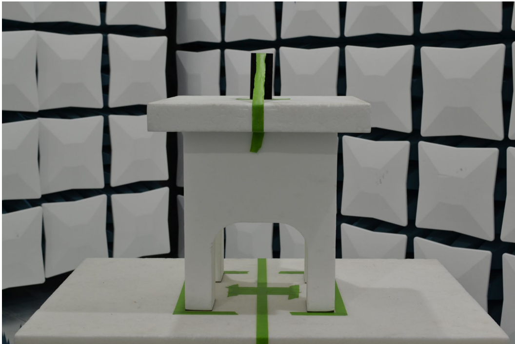
Figure 3. Test Setup – Z Position – 1GHz-40GHz
