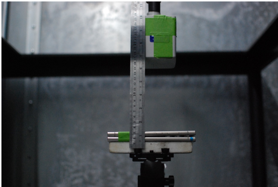
Test Setup Photo 7 H-field, Back side, 15cm
