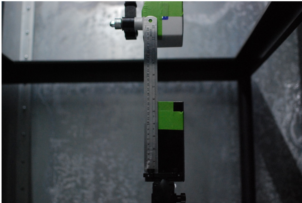
Test Setup Photo 4 E-field, Bottom edge, 15cm
