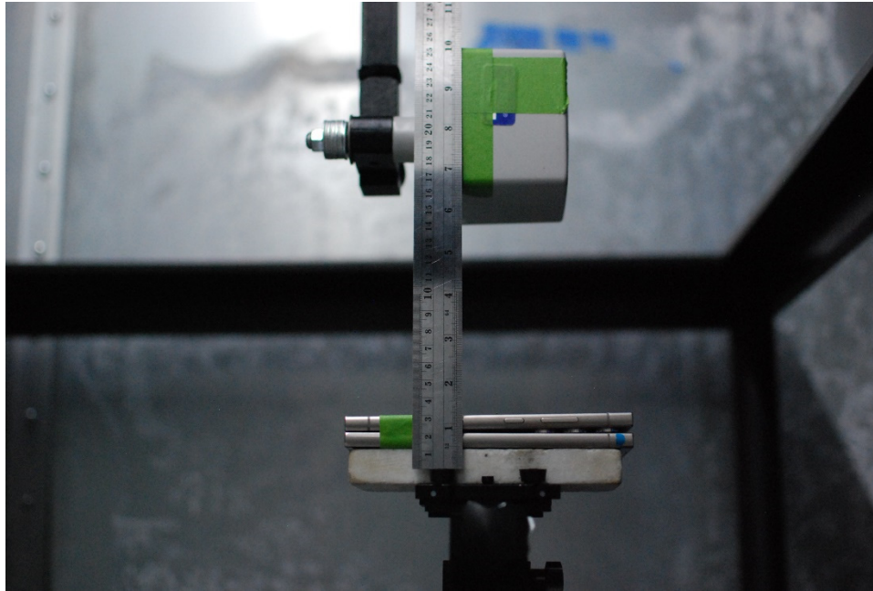
Test Setup Photo 1 E-field, Back side, 15cm
