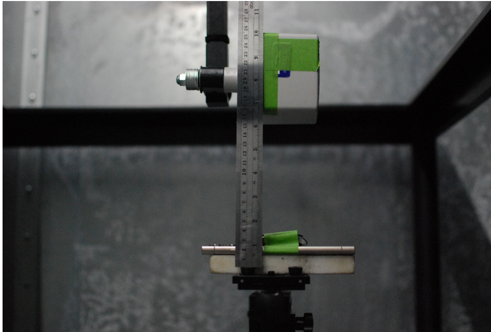
Test Setup Photo 13 E-field, Back side, 15cm
