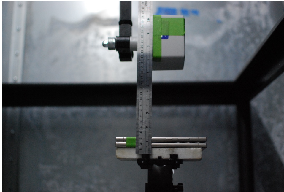
Test Setup Photo 2 E-field, Front side, 15cm
