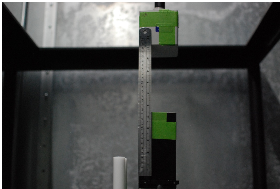
Test Setup Photo 10 H-field, Bottom edge, 15cm
