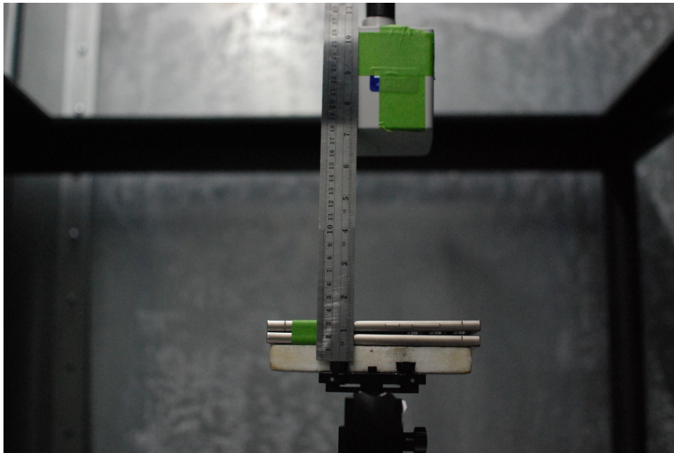
Test Setup Photo 8 H-field, Front side, 15cm
