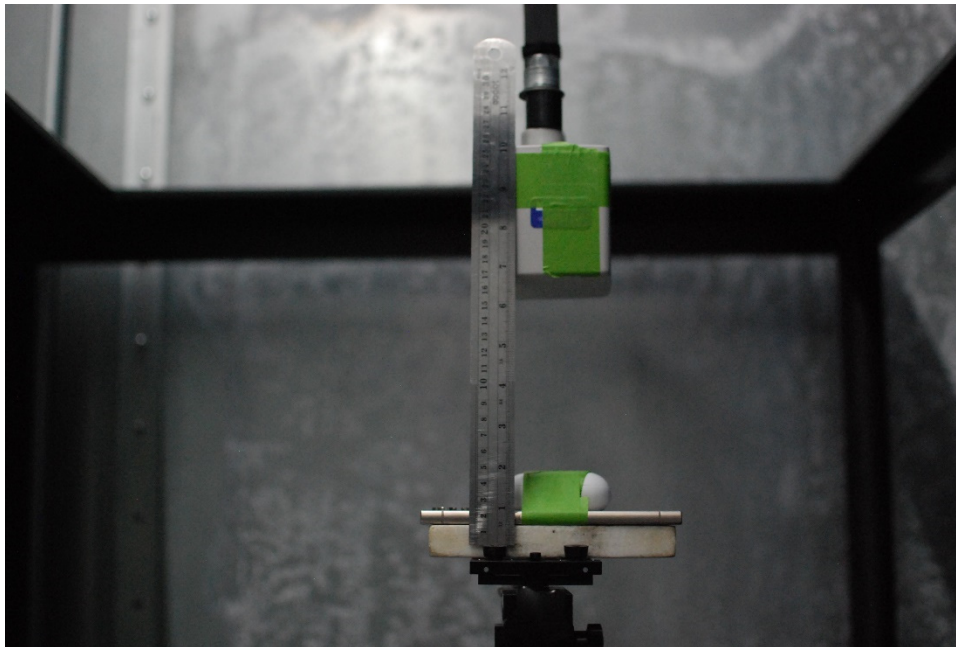
Test Setup Photo 16 H-field, Back side, 15cm
