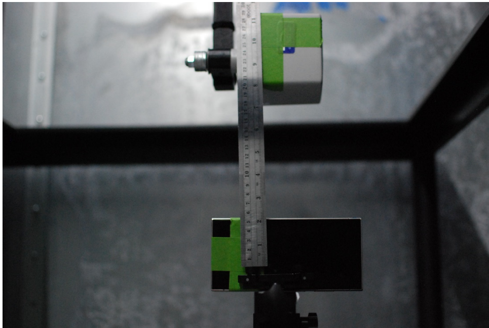
Test Setup Photo 6 E-field, Left edge, 15cm
