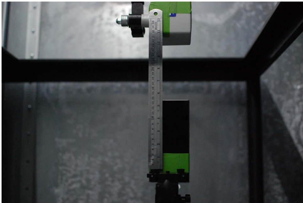
Test Setup Photo 3 E-field, Top edge, 15cm
