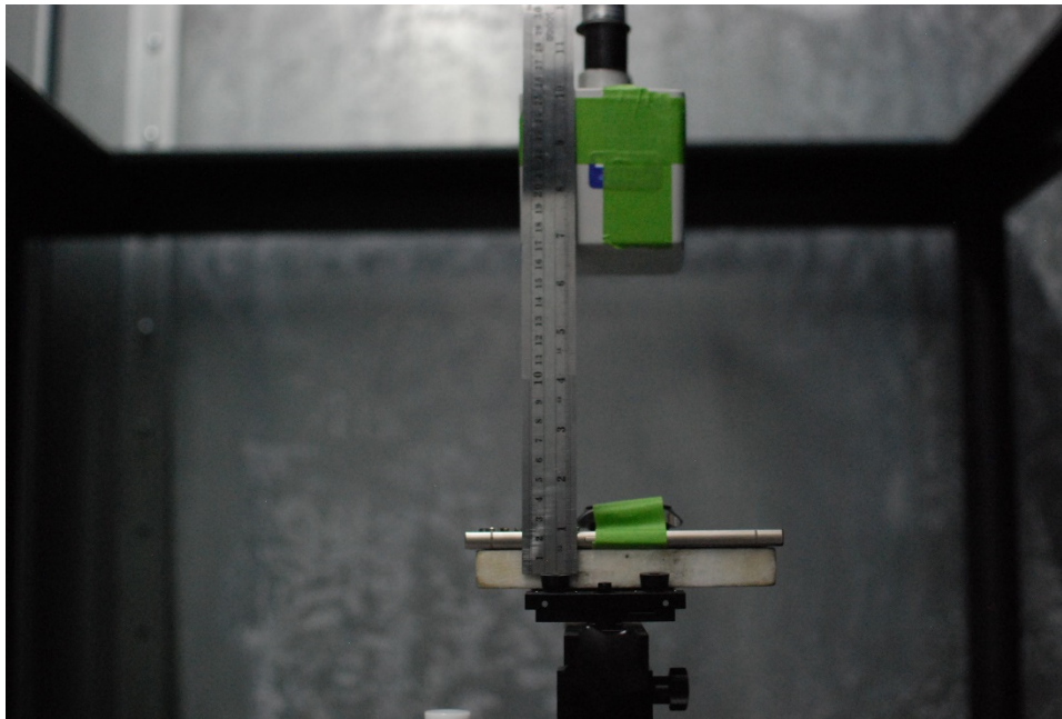
Test Setup Photo 14 H-field, Back side, 15cm
