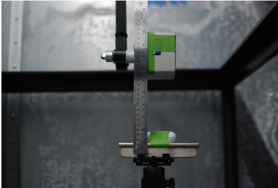
Test Setup Photo 15 E-field, Back side, 15cm
