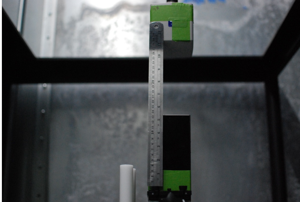
Test Setup Photo 9 H-field, Top edge, 15cm
