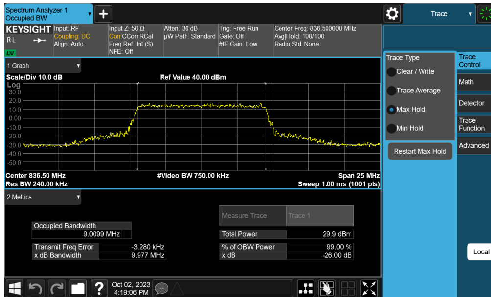
Plot 7-31. Occupied Bandwidth Plot (LTE Band 26/5 - 10MHz QPSK - Full RB Configuration – Ant E)
