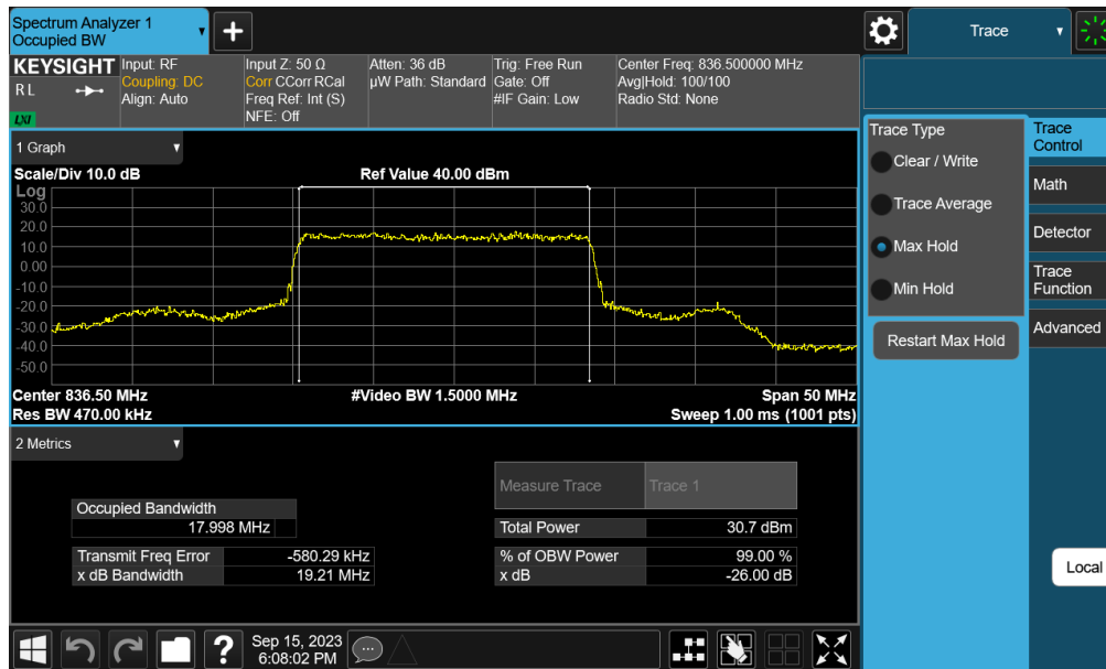
Plot 7-14. Occupied Bandwidth Plot (NR Band n26/5 - 20MHz \pi/2 BPSK - Full RB Configuration – Ant A)
