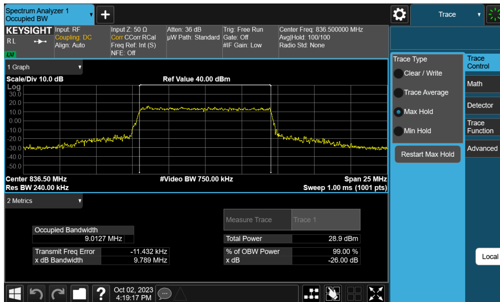
Plot 7-32. Occupied Bandwidth Plot (LTE Band 26/5 - 10MHz 16-QAM - Full RB Configuration – Ant E)
