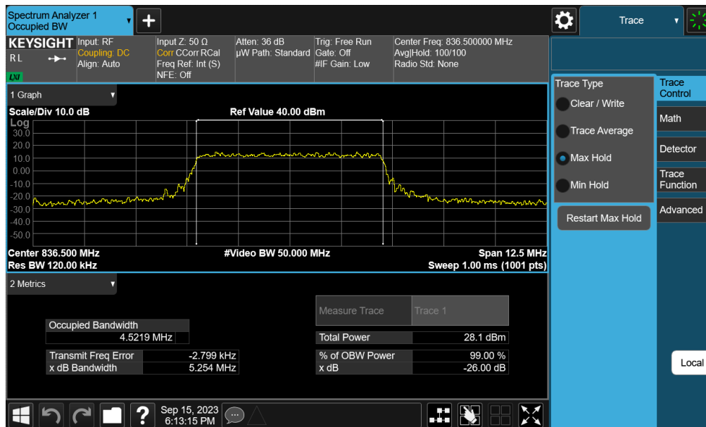
Plot 7-25. Occupied Bandwidth Plot (NR Band n26/5 - 5MHz 16-QAM - Full RB Configuration – Ant A)
