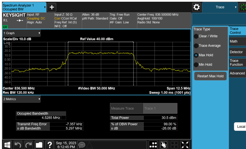
Plot 7-23. Occupied Bandwidth Plot (NR Band n26/5 - 5MHz \pi/2 BPSK - Full RB Configuration – Ant A)
