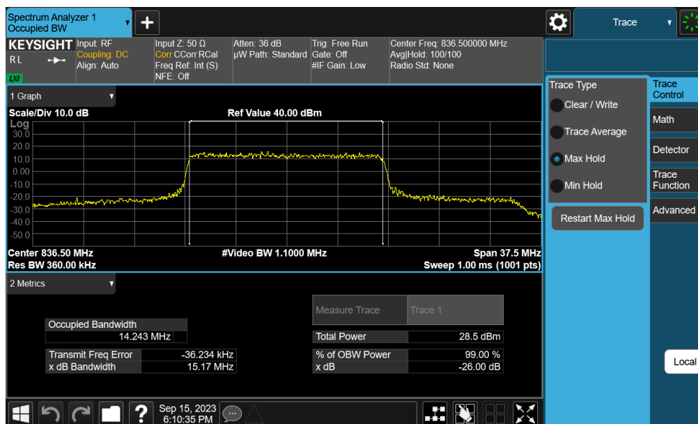
Plot 7-19. Occupied Bandwidth Plot (NR Band n26/5 - 15MHz 16-QAM - Full RB Configuration – Ant A)
