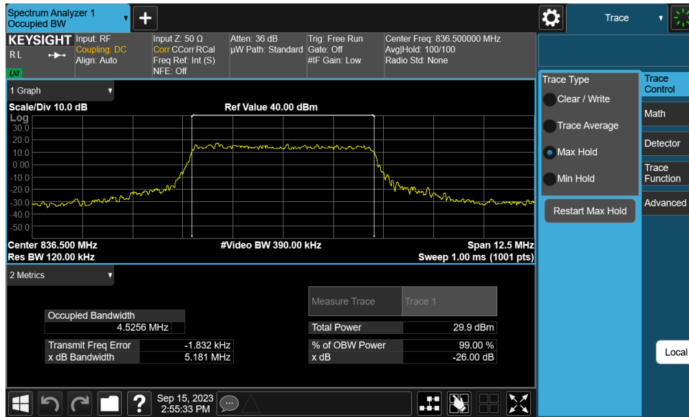
Plot 7-8. Occupied Bandwidth Plot (LTE Band 26/5 - 5MHz QPSK - Full RB Configuration – Ant A)
