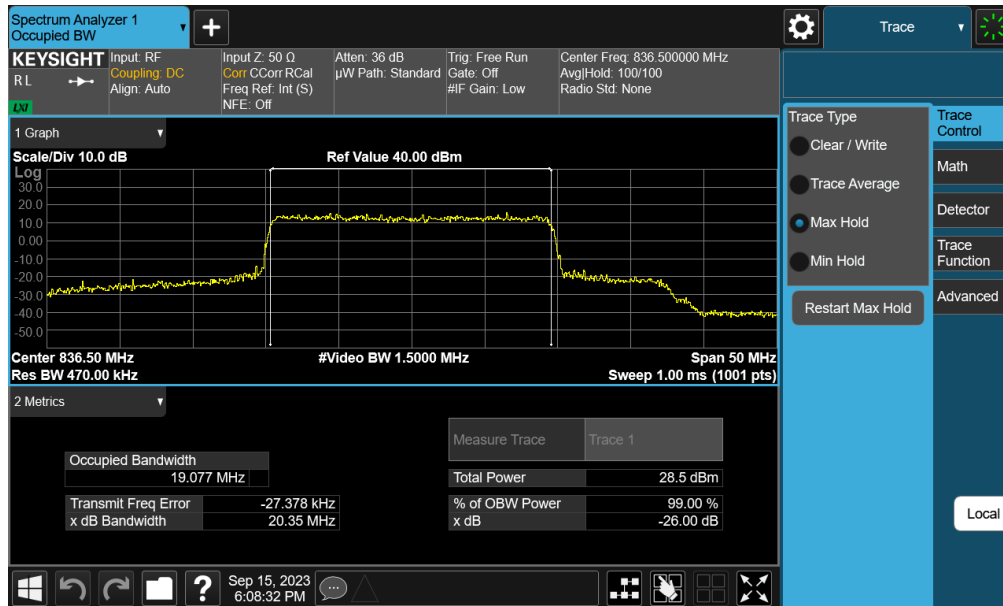
Plot 7-15. Occupied Bandwidth Plot (NR Band n26/5 - 20MHz QPSK - Full RB Configuration – Ant A)
