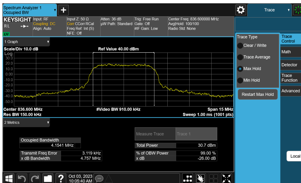
Plot 7-28. Occupied Bandwidth Plot (WCDMA, Ch. 4183 – Ant E)
