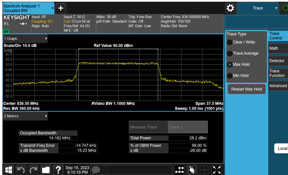
Plot 7-18. Occupied Bandwidth Plot (NR Band n26/5 - 15MHz QPSK - Full RB Configuration – Ant A)
