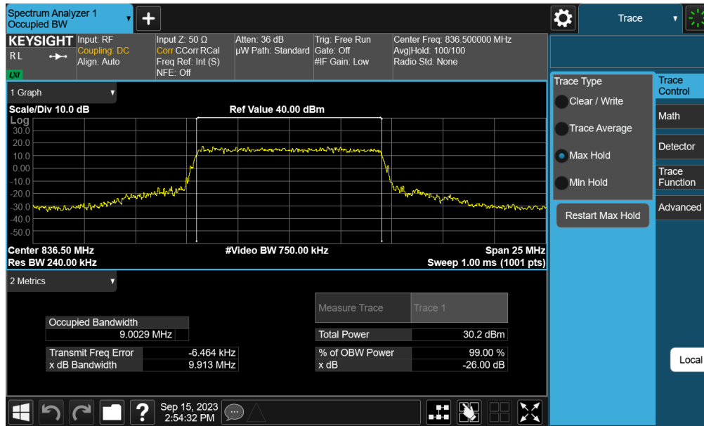
Plot 7-6. Occupied Bandwidth Plot (LTE Band 26/5 - 10MHz QPSK - Full RB Configuration – Ant A)
