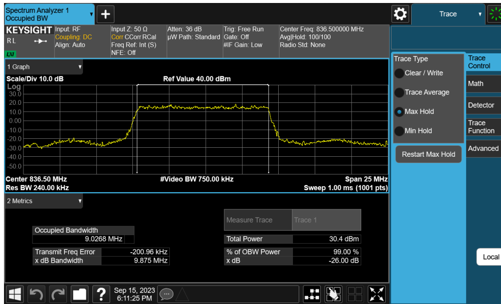
Plot 7-20. Occupied Bandwidth Plot (NR Band n26/5 - 10MHz \pi/2 BPSK - Full RB Configuration – Ant A)
