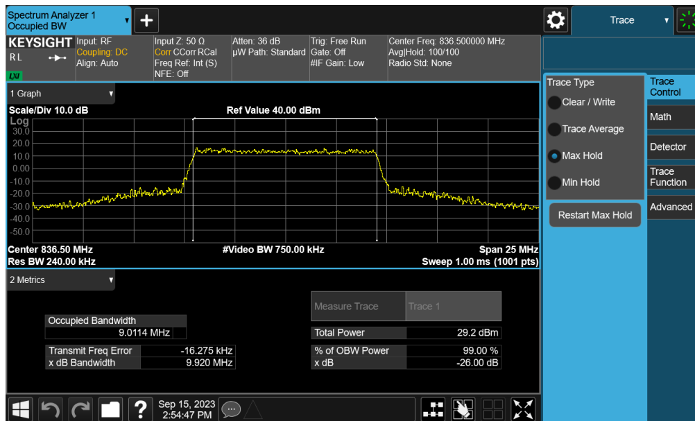
Plot 7-7. Occupied Bandwidth Plot (LTE Band 26/5 - 10MHz 16-QAM - Full RB Configuration – Ant A)
