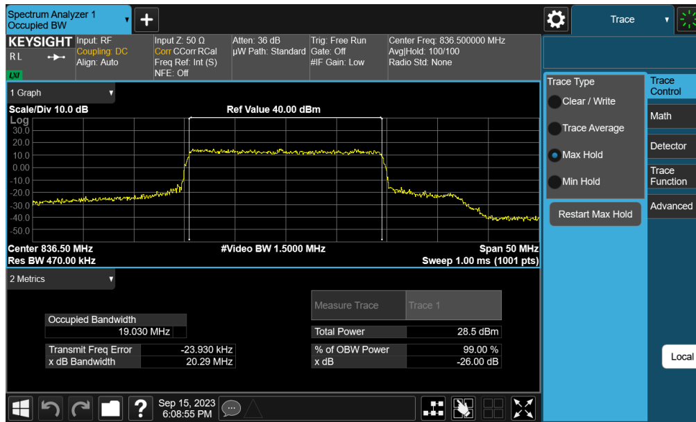
Plot 7-16. Occupied Bandwidth Plot (NR Band n26/5 - 20MHz 16-QAM - Full RB Configuration – Ant A)
