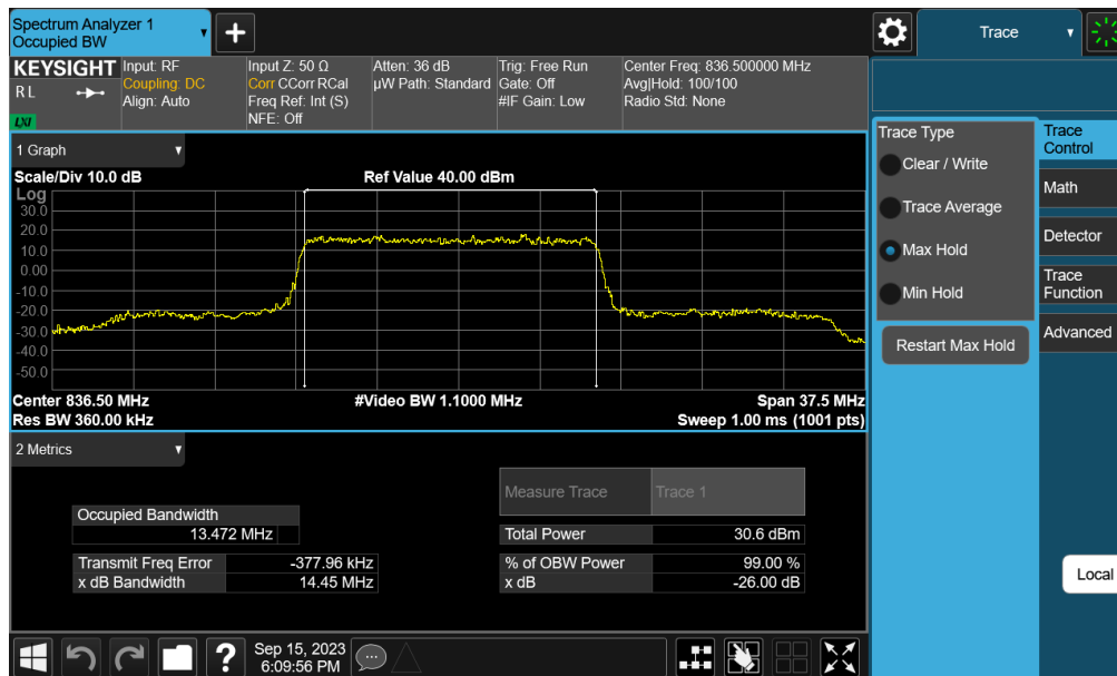
Plot 7-17. Occupied Bandwidth Plot (NR Band n26/5 - 15MHz \pi/2 BPSK - Full RB Configuration – Ant A)
