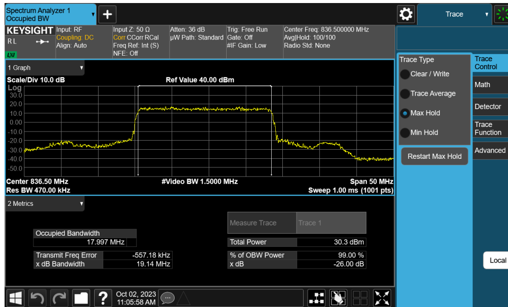
Plot 7-39. Occupied Bandwidth Plot (NR Band n26/5 - 20MHz \pi/2 BPSK - Full RB Configuration – Ant E)
