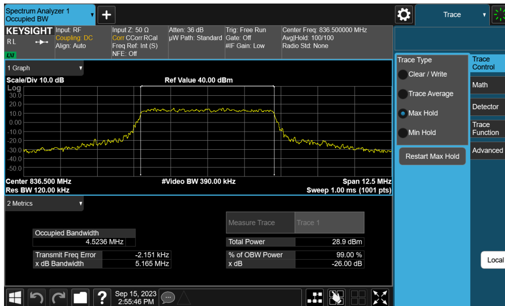
Plot 7-9. Occupied Bandwidth Plot (LTE Band 26/5 - 5MHz 16-QAM - Full RB Configuration – Ant A)
