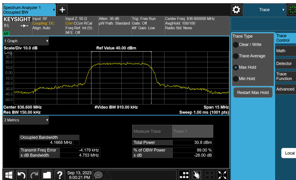
Plot 7-3. Occupied Bandwidth Plot (WCDMA, Ch. 4183 – Ant A)
