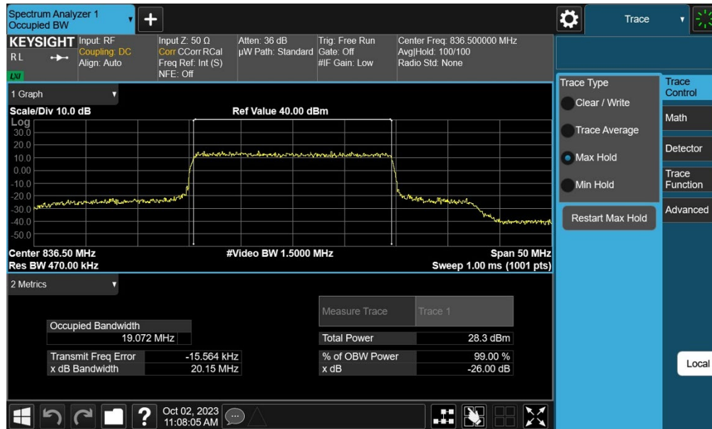
Plot 7-40. Occupied Bandwidth Plot (NR Band n26/5 - 20MHz QPSK - Full RB Configuration – Ant E)
