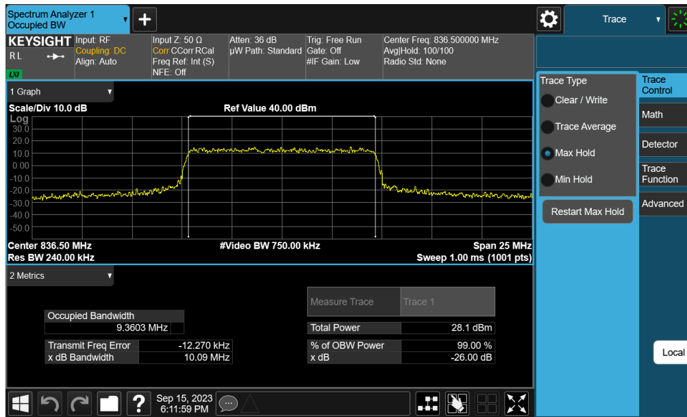
Plot 7-22. Occupied Bandwidth Plot (NR Band n26/5 - 10MHz 16-QAM - Full RB Configuration – Ant A)
