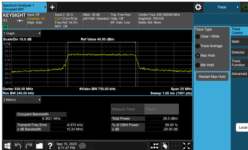
Plot 7-21. Occupied Bandwidth Plot (NR Band n26/5 - 10MHz QPSK - Full RB Configuration – Ant A)
