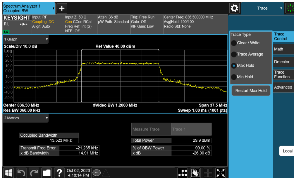
Plot 7-29. Occupied Bandwidth Plot (LTE Band 26 - 15MHz QPSK - Full RB Configuration – Ant E)
