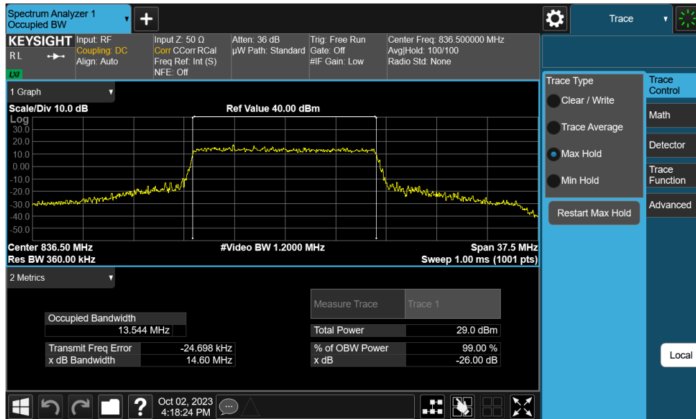
Plot 7-30. Occupied Bandwidth Plot (LTE Band 26 - 15MHz 16-QAM - Full RB Configuration – Ant E)
