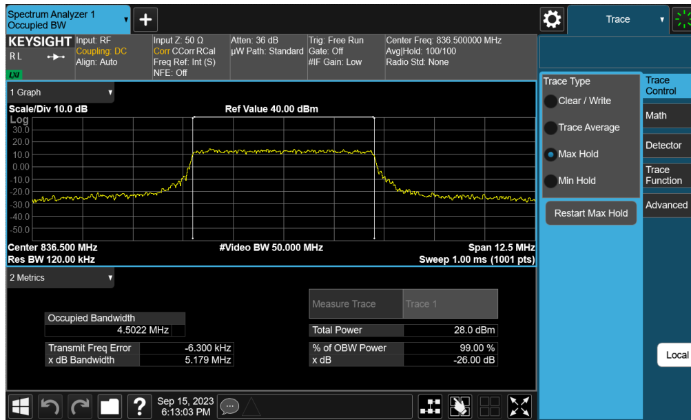
Plot 7-24. Occupied Bandwidth Plot (NR Band n26/5 - 5MHz QPSK - Full RB Configuration – Ant A)
