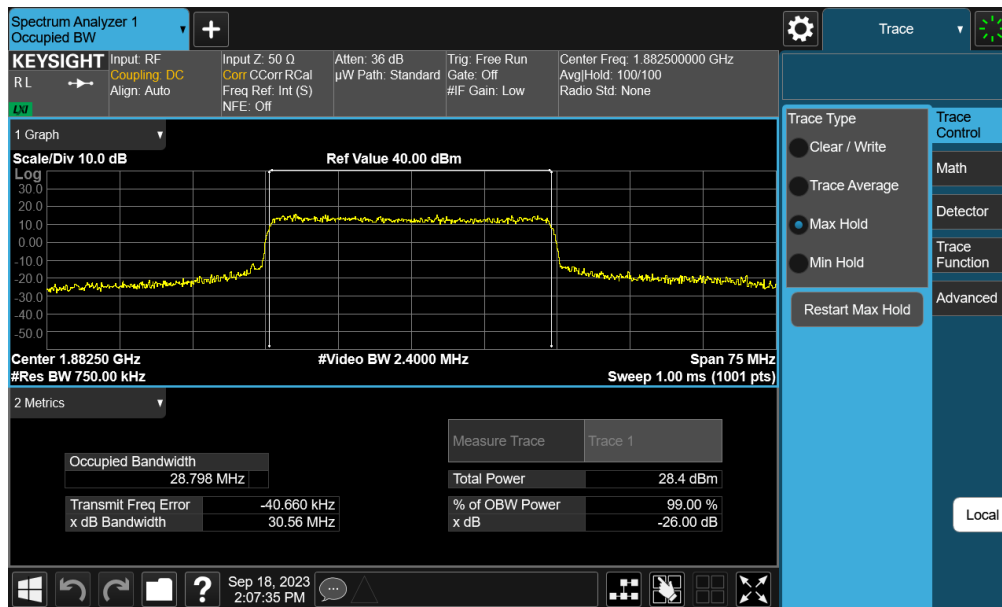
Plot 7-20. Occupied Bandwidth Plot (NR Band n25/2 - 30.0MHz CP-OFDM QPSK - Full RB - ANT A)
