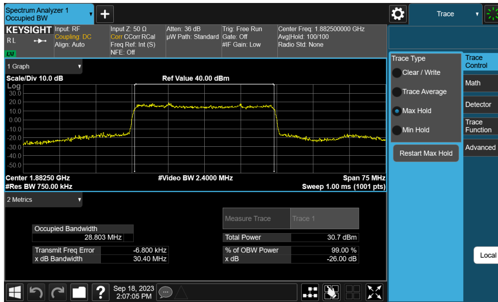
Plot 7-19. Occupied Bandwidth Plot (NR Band n25/2 - 30.0MHz DFT-s-OFDM BPSK - Full RB - ANT A)
