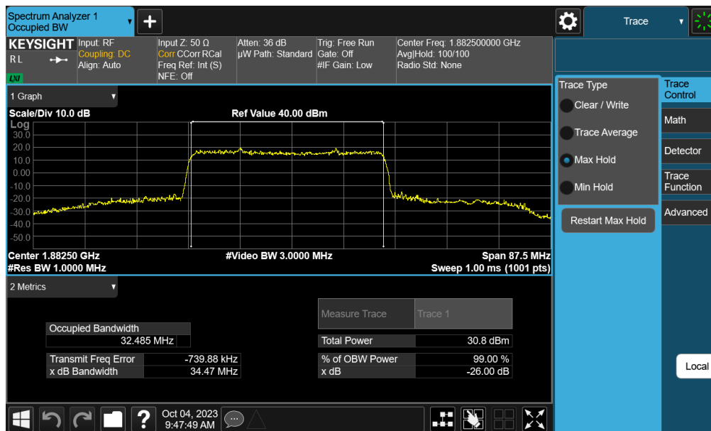
Plot 7-16. Occupied Bandwidth Plot (NR Band n25/2 - 35.0MHz DFT-s-OFDM BPSK - Full RB - ANT A)
