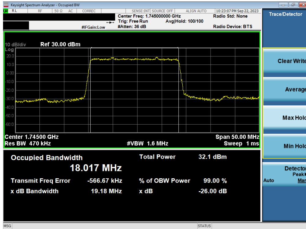
Plot 7-67. Occupied Bandwidth Plot (NR Band n66 - 20.0MHz DFT-s-OFDM BPSK - Full RB – ANT1)
