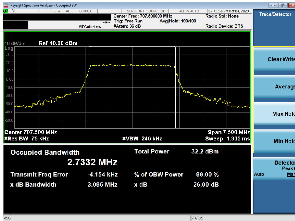
Plot 7-100. Occupied Bandwidth Plot (LTE Band 12 - 3MHz QPSK - Full RB – ANT2)
