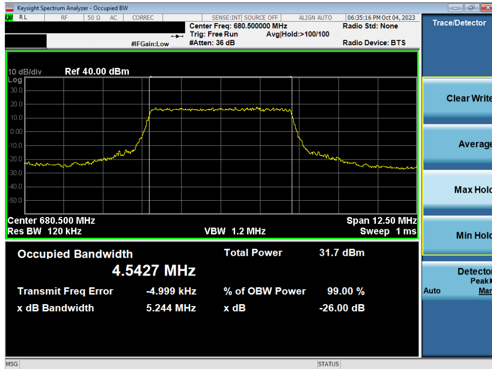
Plot 7-94. Occupied Bandwidth Plot (LTE Band 71 - 5MHz QPSK - Full RB – ANT2)
