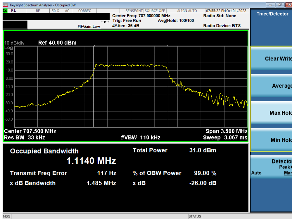
Plot 7-103. Occupied Bandwidth Plot (LTE Band 12 – 1.4MHz 16-QAM - Full RB – ANT2)
