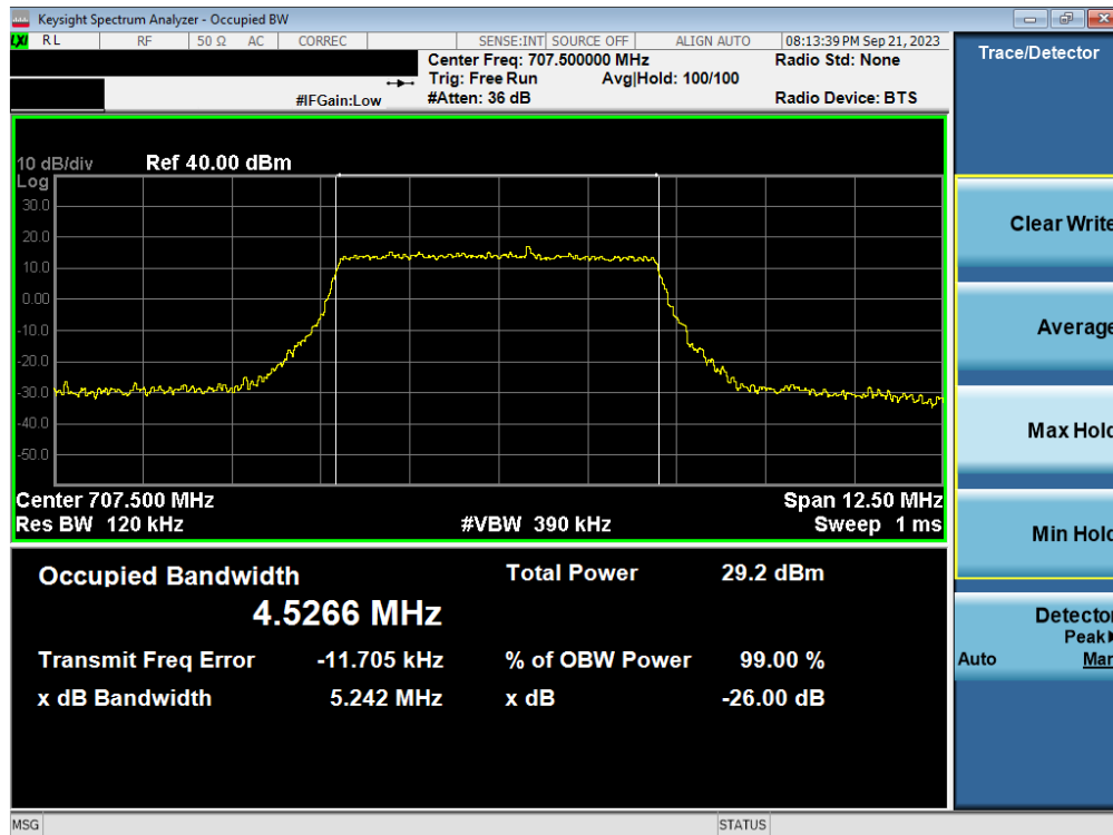
Plot 7-40. Occupied Bandwidth Plot (NR Band n12 - 5MHz CP-OFDM QPSK - Full RB – ANT1)
