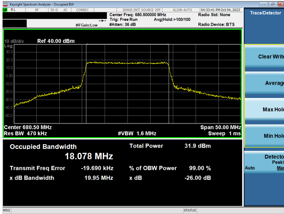
Plot 7-88. Occupied Bandwidth Plot (LTE Band 71 - 20MHz QPSK - Full RB – ANT2)
