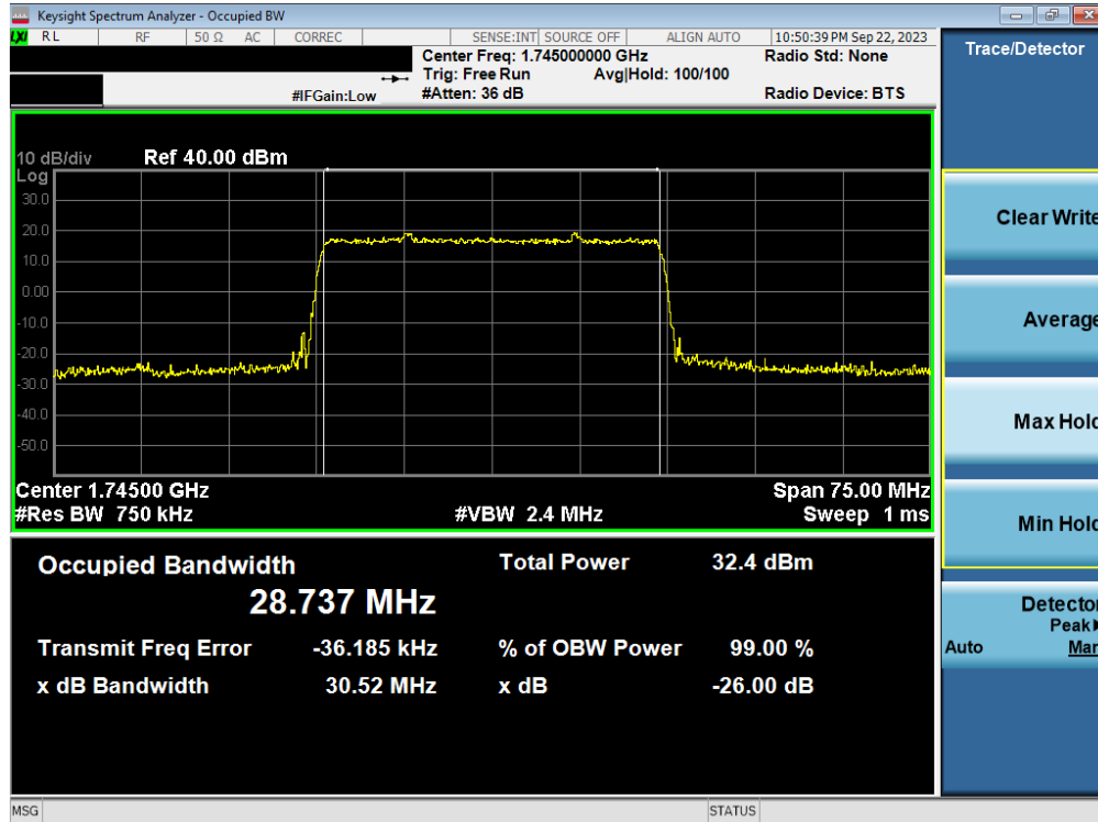
Plot 7-61. Occupied Bandwidth Plot (NR Band n66 - 30.0MHz DFT-s-OFDM BPSK - Full RB – ANT1)
