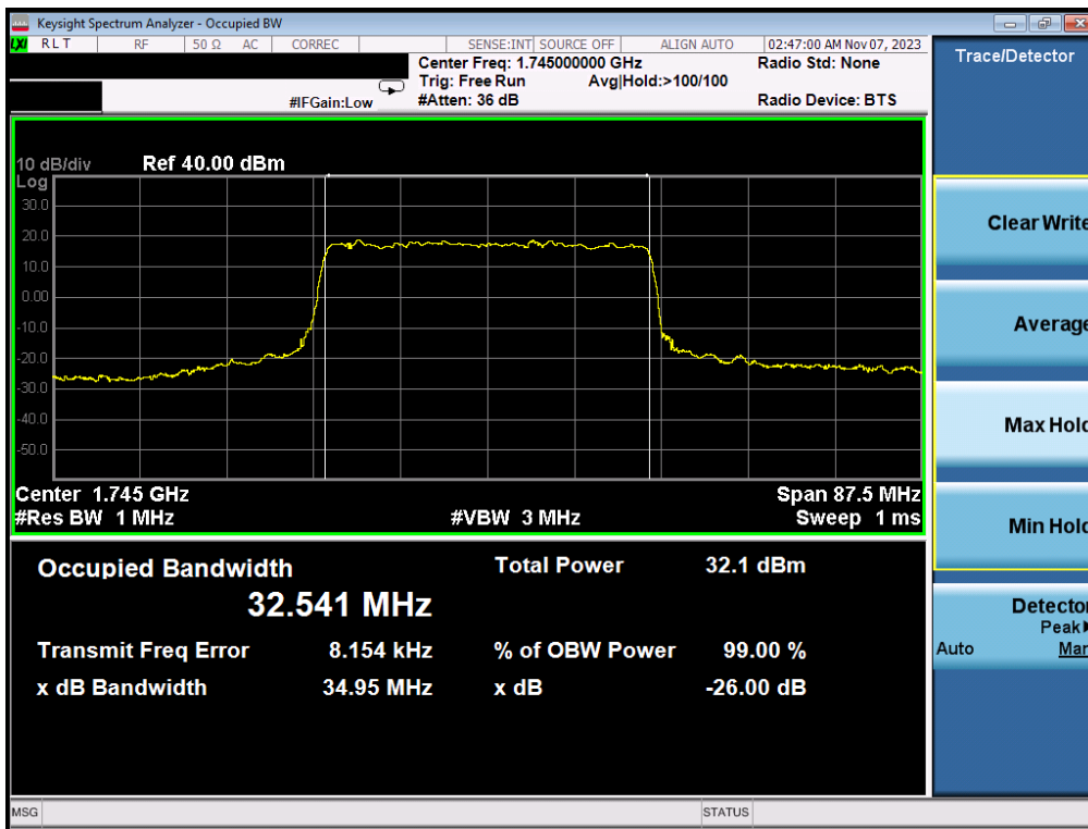
Plot 7-58. Occupied Bandwidth Plot (NR Band n66 - 35.0MHz DFT-s-OFDM BPSK - Full RB – ANT1)
