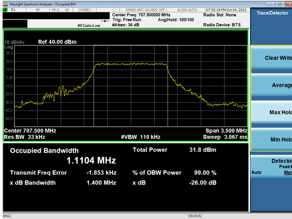
Plot 7-102. Occupied Bandwidth Plot (LTE Band 12 – 1.4MHz QPSK - Full RB – ANT2)
