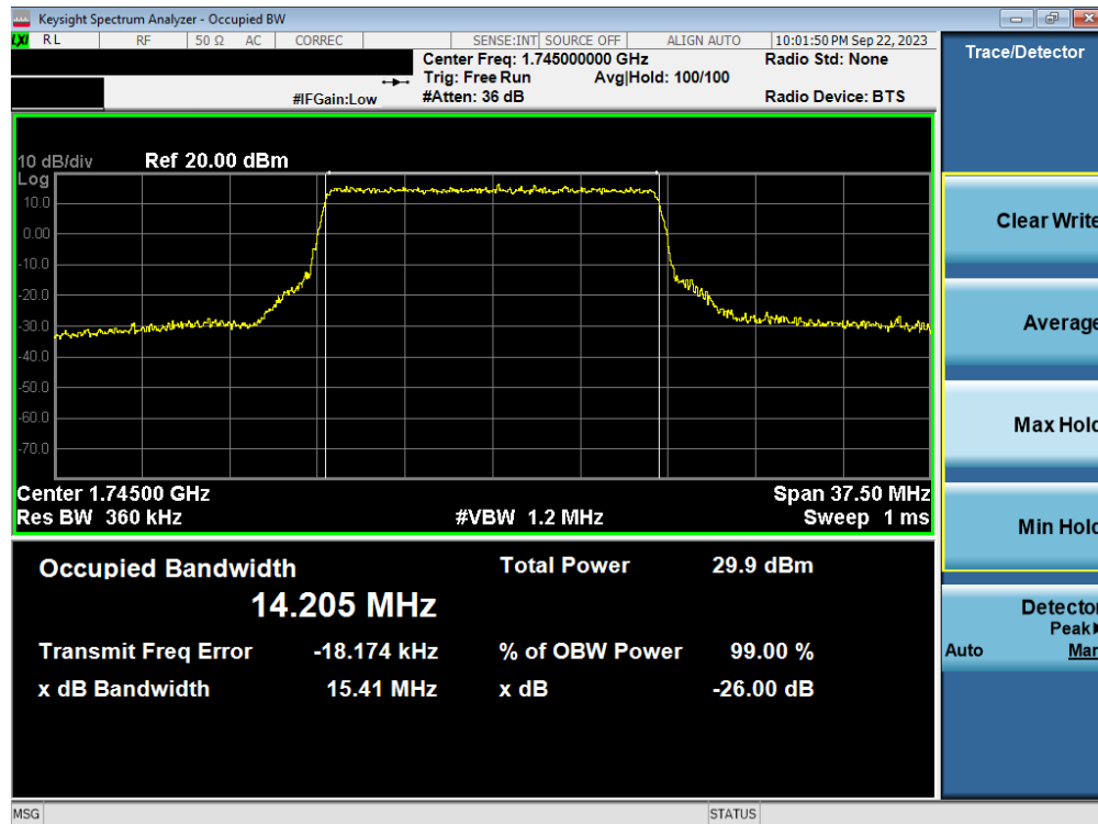
Plot 7-72. Occupied Bandwidth Plot (NR Band n66 - 15.0MHz CP-OFDM 16QAM - Full RB – ANT1)
