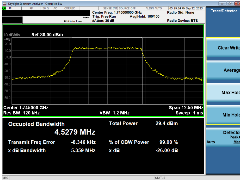
Plot 7-78. Occupied Bandwidth Plot (NR Band n66 - 5.0MHz CP-OFDM 16QAM - Full RB - ANT1)
