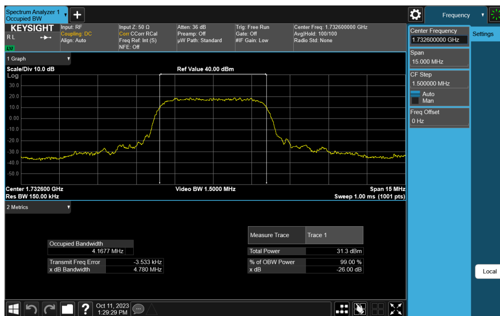
Plot 7-42. Occupied Bandwidth Plot (WCDMA, Ch. 1413 – ANT1)
