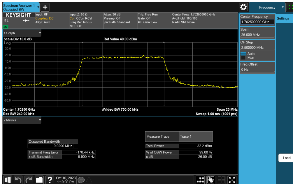
Plot 7-82. Occupied Bandwidth Plot (NR Band n70 - 10.0MHz DFT-s-OFDM BPSK - Full RB – ANT1)
