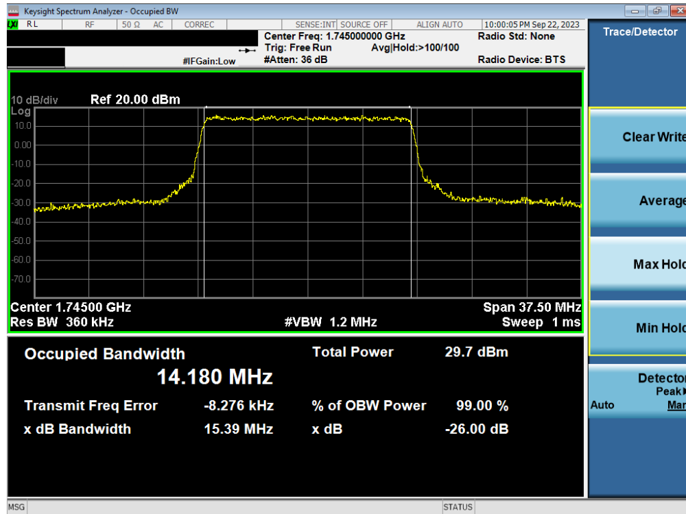
Plot 7-71. Occupied Bandwidth Plot (NR Band n66 - 15.0MHz CP-OFDM QPSK - Full RB – ANT1)
