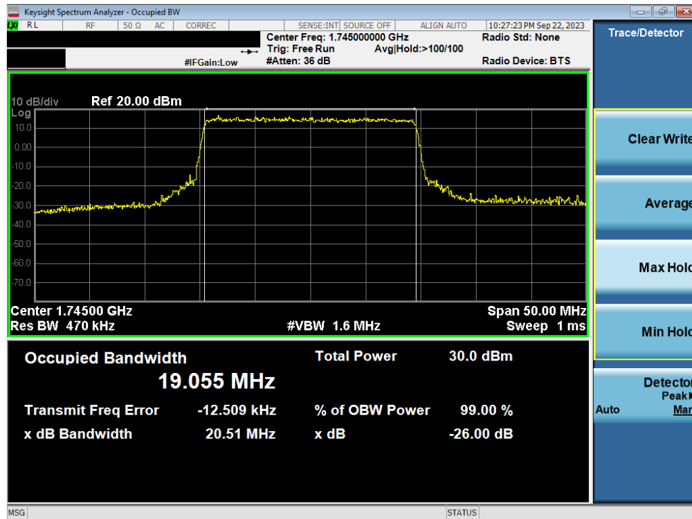
Plot 7-68. Occupied Bandwidth Plot (NR Band n66 - 20.0MHz CP-OFDM QPSK - Full RB – ANT1)
