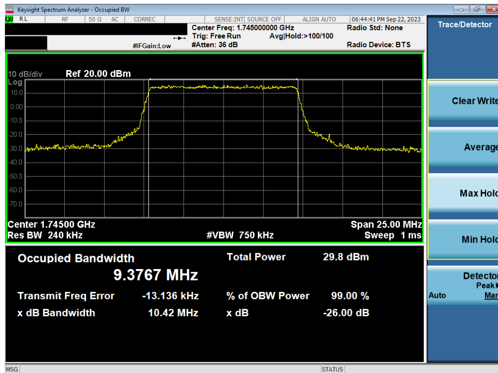
Plot 7-74. Occupied Bandwidth Plot (NR Band n66 - 10.0MHz CP-OFDM QPSK - Full RB – ANT1)
