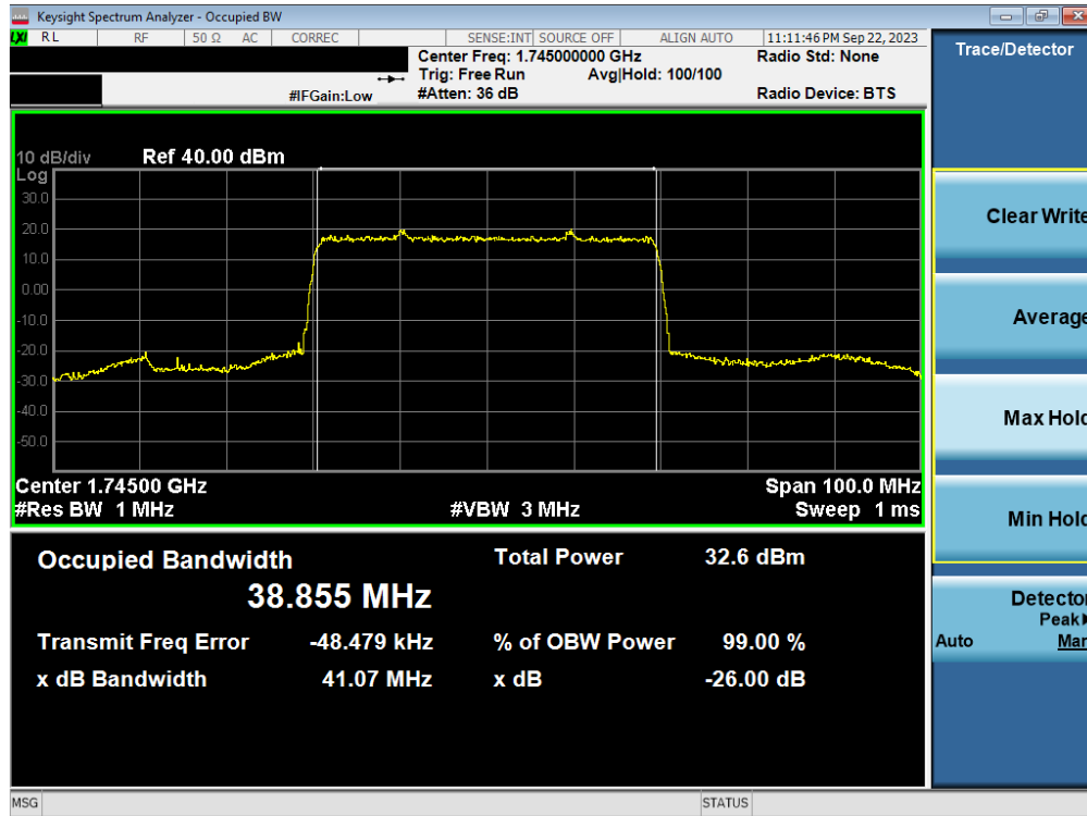
Plot 7-55. Occupied Bandwidth Plot (NR Band n66 - 40.0MHz DFT-s-OFDM BPSK - Full RB – ANT1)
