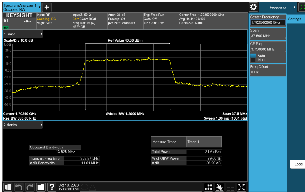
Plot 7-79. Occupied Bandwidth Plot (NR Band n70 - 15.0MHz DFT-s-OFDM BPSK - Full RB – ANT1)
