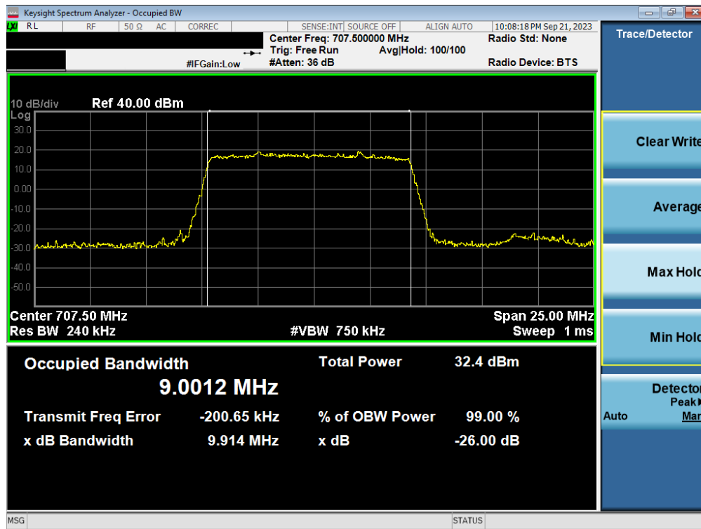
Plot 7-36. Occupied Bandwidth Plot (NR Band n12 - 10MHz DFT-s-OFDM BPSK - Full RB – ANT1)
