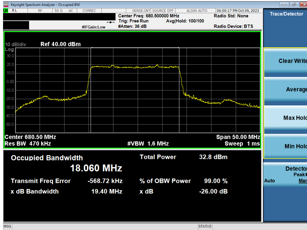
Plot 7-108. Occupied Bandwidth Plot (NR Band n71 - 20MHz DFT-s-OFDM BPSK - Full RB – ANT2)
