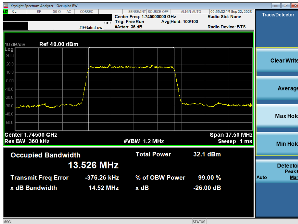
Plot 7-70. Occupied Bandwidth Plot (NR Band n66 - 15.0MHz DFT-s-OFDM BPSK - Full RB – ANT1)
