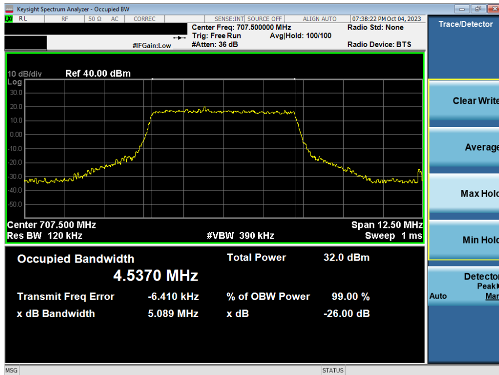
Plot 7-98. Occupied Bandwidth Plot (LTE Band 12 - 5MHz QPSK - Full RB – ANT2)
