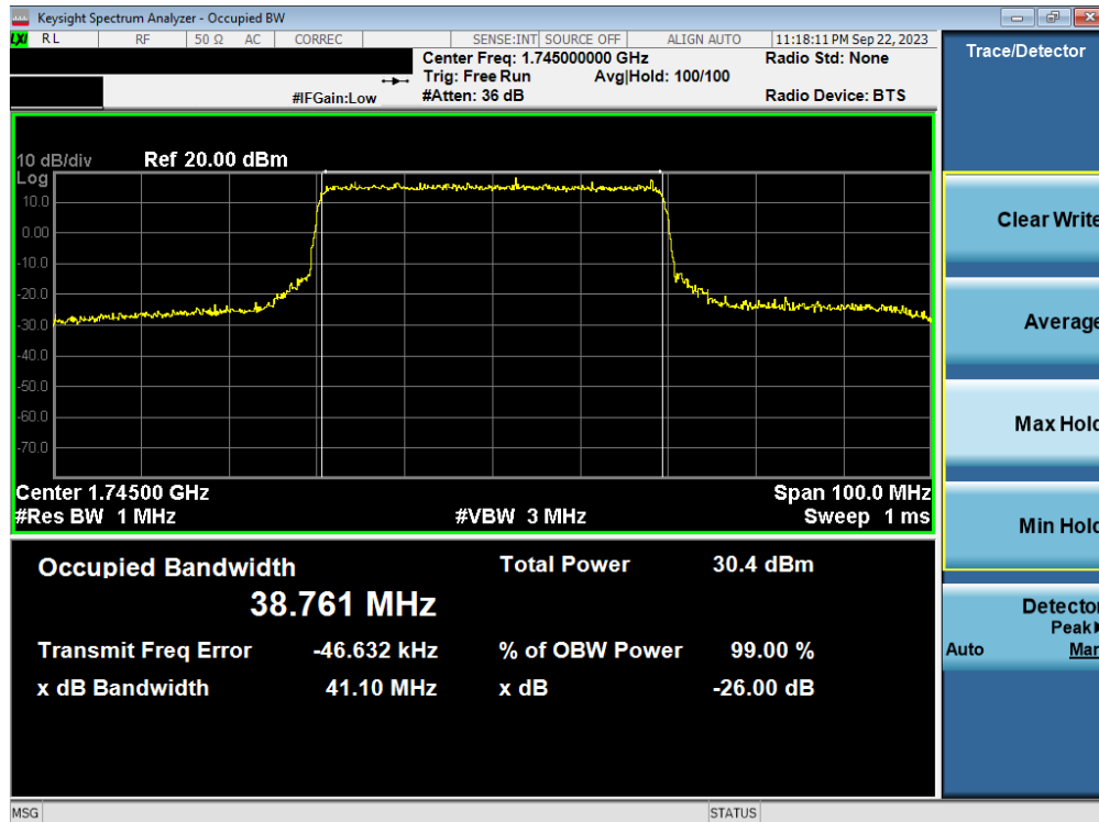
Plot 7-56. Occupied Bandwidth Plot (NR Band n66 - 40.0MHz CP-OFDM QPSK - Full RB – ANT1)
