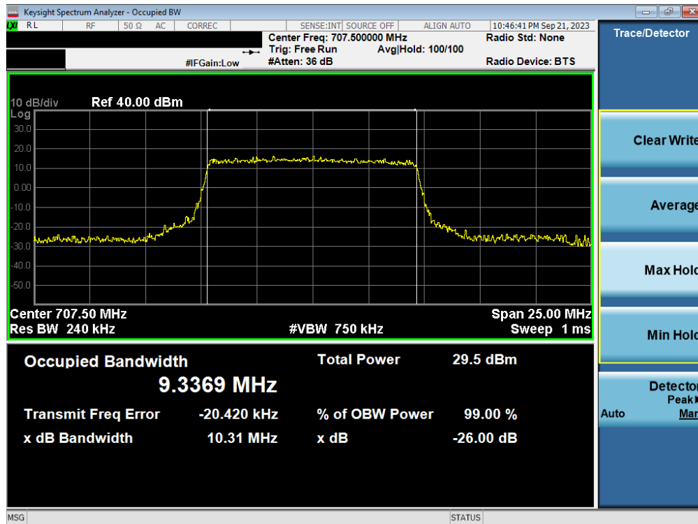
Plot 7-38. Occupied Bandwidth Plot (NR Band n12 - 10MHz CP-OFDM 16-QAM - Full RB – ANT1)
