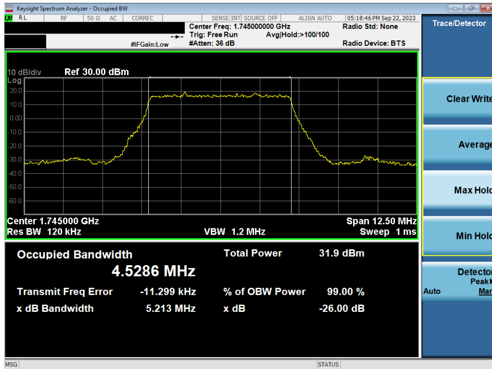
Plot 7-76. Occupied Bandwidth Plot (NR Band n66 - 5.0MHz DFT-s-OFDM BPSK - Full RB – ANT1)
