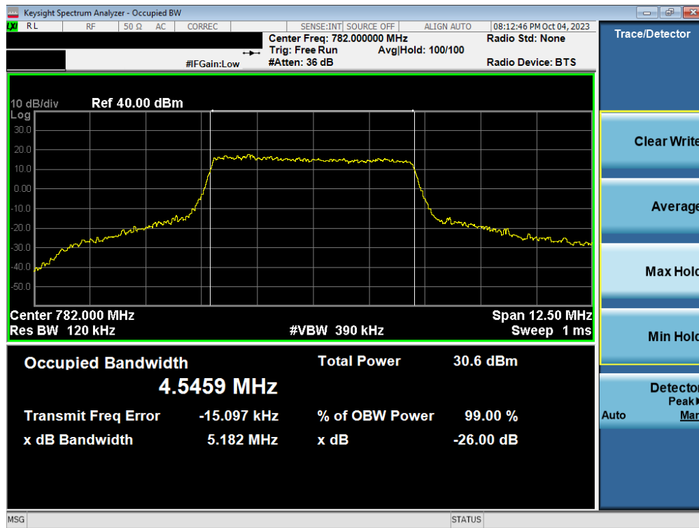
Plot 7-107. Occupied Bandwidth Plot (LTE Band 13 - 5MHz 16-QAM - Full RB – ANT2)
