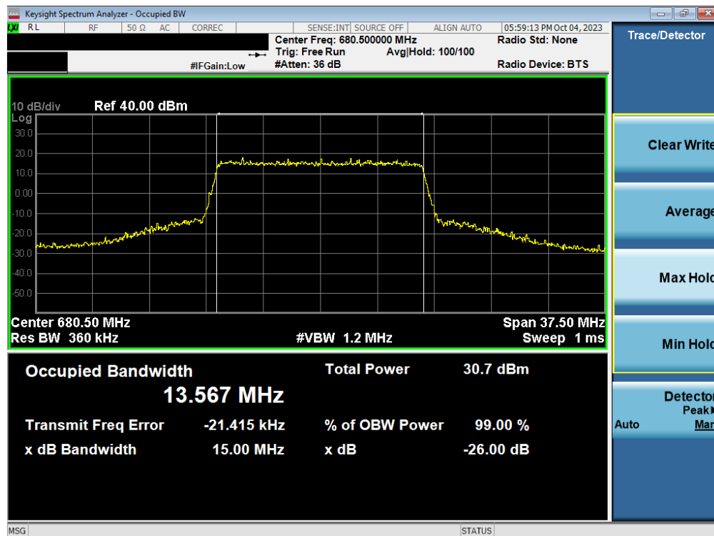
Plot 7-91. Occupied Bandwidth Plot (LTE Band 71 - 15MHz 16-QAM - Full RB – ANT2)
