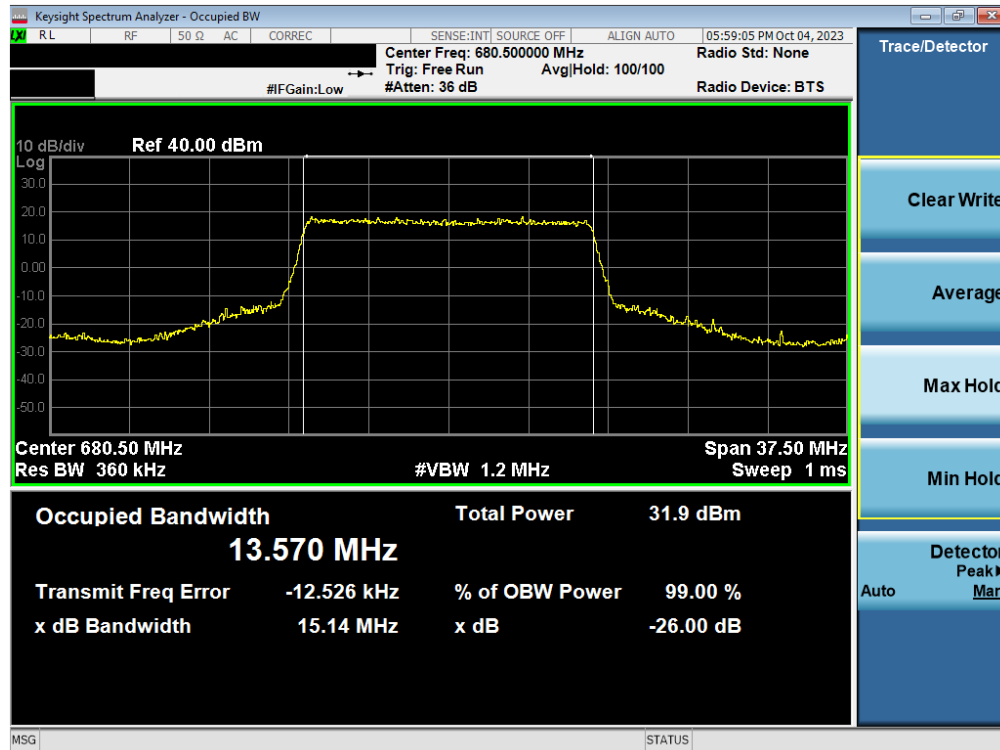
Plot 7-90. Occupied Bandwidth Plot (LTE Band 71 - 15MHz QPSK - Full RB – ANT2)
