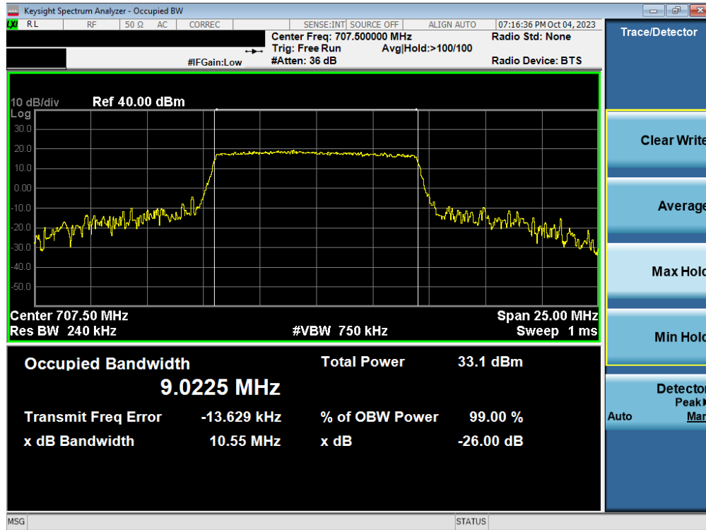
Plot 7-96. Occupied Bandwidth Plot (LTE Band 12 - 10MHz QPSK - Full RB – ANT2)
