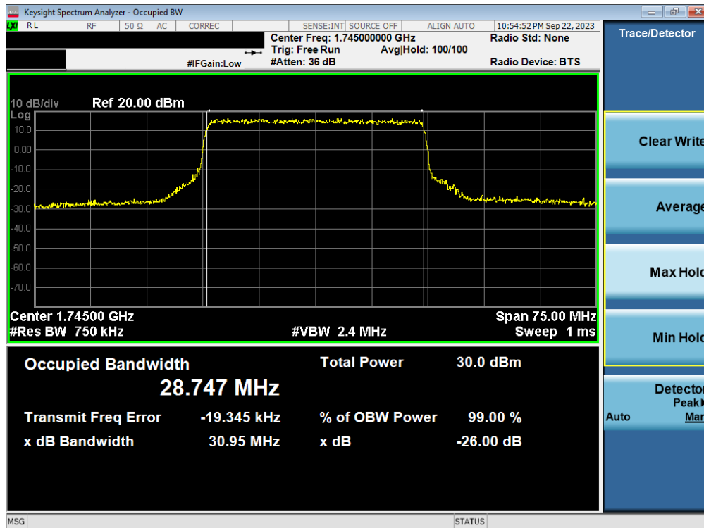
Plot 7-62. Occupied Bandwidth Plot (NR Band n66 - 30.0MHz CP-OFDM QPSK - Full RB – ANT1)
