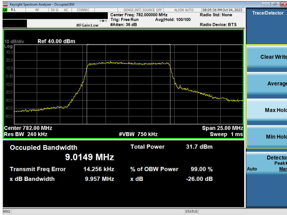
Plot 7-104. Occupied Bandwidth Plot (LTE Band 13 - 10MHz QPSK - Full RB – ANT2)
