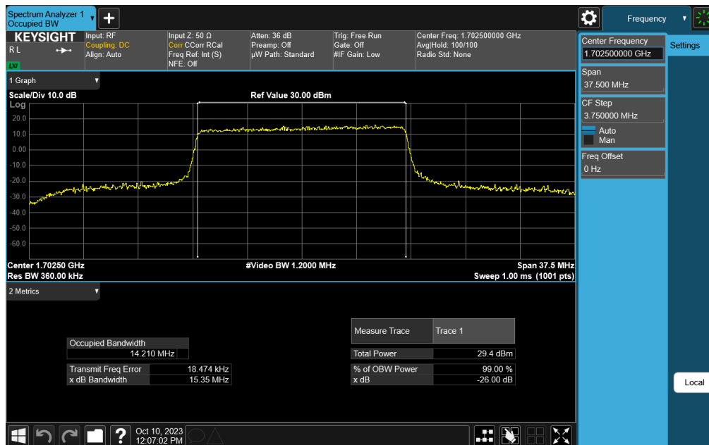
Plot 7-80. Occupied Bandwidth Plot (NR Band n70 - 15.0MHz CP-OFDM QPSK - Full RB – ANT1)
