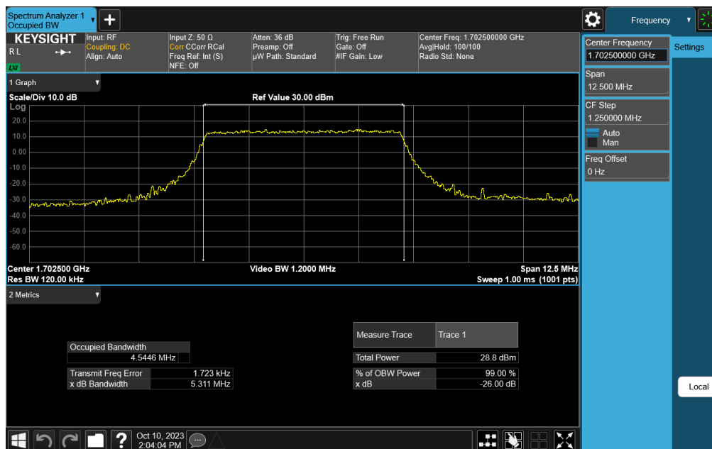
Plot 7-86. Occupied Bandwidth Plot (NR Band n70 - 5.0MHz CP-OFDM QPSK - Full RB – ANT1)
