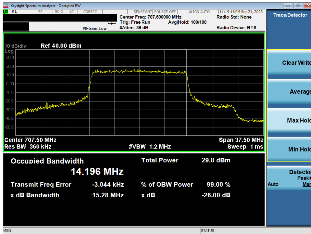
Plot 7-35. Occupied Bandwidth Plot (NR Band n12 - 15MHz CP-OFDM 16-QAM - Full RB – ANT1)
