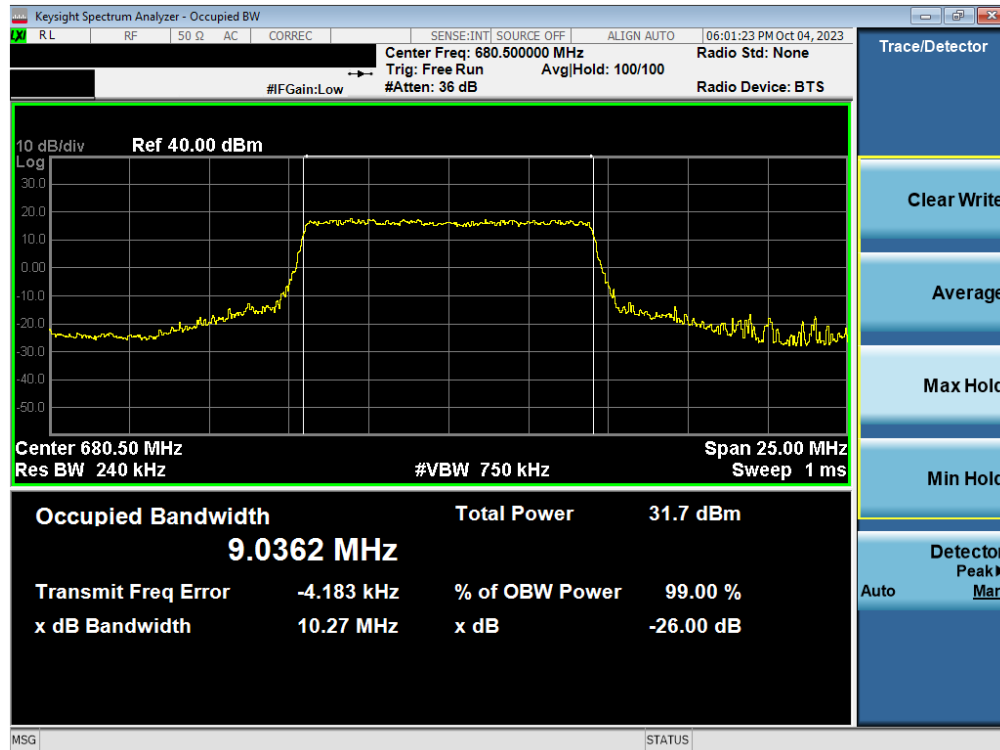
Plot 7-92. Occupied Bandwidth Plot (LTE Band 71 - 10MHz QPSK - Full RB – ANT2)
