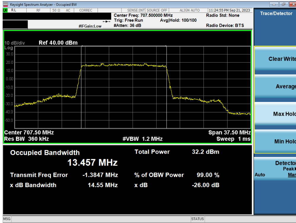
Plot 7-33. Occupied Bandwidth Plot (NR Band n12 - 15MHz DFT-s-OFDM BPSK - Full RB – ANT1)
