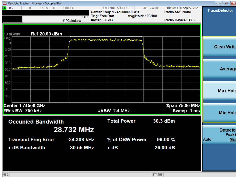
Plot 7-63. Occupied Bandwidth Plot (NR Band n66 - 30.0MHz CP-OFDM 16QAM - Full RB – ANT1)
