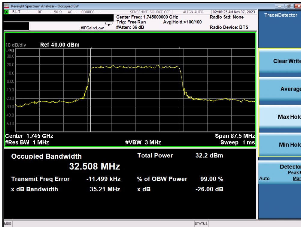
Plot 7-59. Occupied Bandwidth Plot (NR Band n66 - 35.0MHz CP-OFDM QPSK - Full RB – ANT1)
