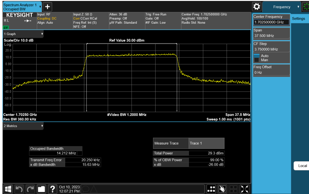
Plot 7-81. Occupied Bandwidth Plot (NR Band n70 - 15.0MHz CP-OFDM 16QAM - Full RB – ANT1)
