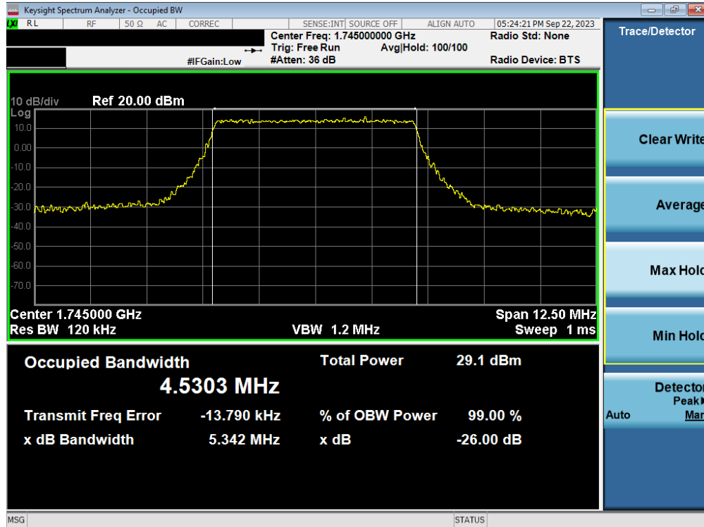
Plot 7-77. Occupied Bandwidth Plot (NR Band n66 - 5.0MHz CP-OFDM QPSK - Full RB - ANT1)
