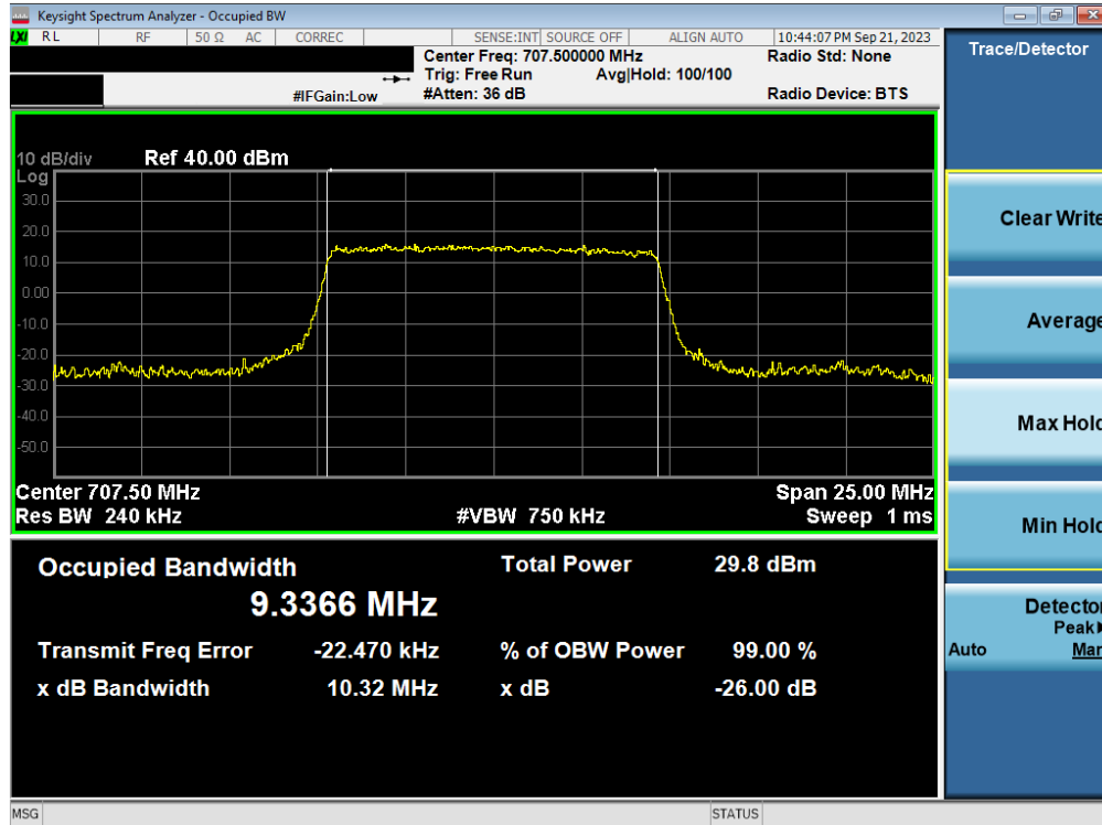
Plot 7-37. Occupied Bandwidth Plot (NR Band n12 - 10MHz CP-OFDM QPSK - Full RB – ANT1)
