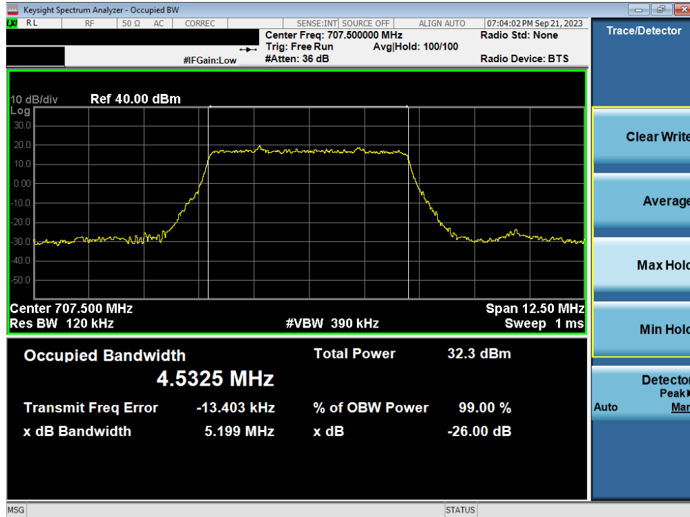
Plot 7-39. Occupied Bandwidth Plot (NR Band n12 - 5MHz DFT-s-OFDM BPSK - Full RB – ANT1)
