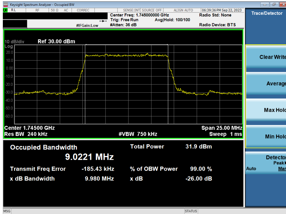
Plot 7-73. Occupied Bandwidth Plot (NR Band n66 - 10.0MHz DFT-s-OFDM BPSK - Full RB – ANT1)
