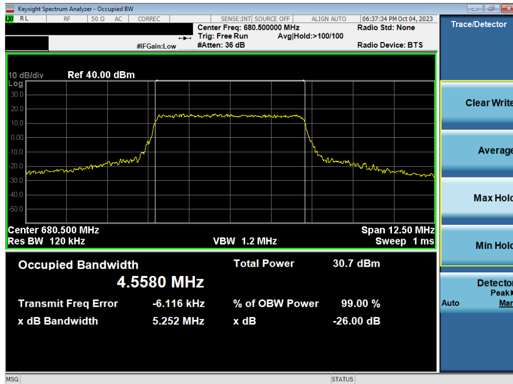
Plot 7-95. Occupied Bandwidth Plot (LTE Band 71 - 5MHz 16-QAM - Full RB – ANT2)
