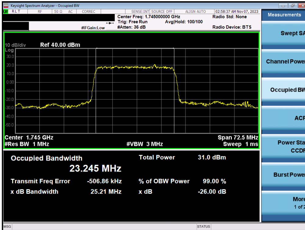
Plot 7-64. Occupied Bandwidth Plot (NR Band n66 - 25.0MHz DFT-s-OFDM BPSK - Full RB – ANT1)
