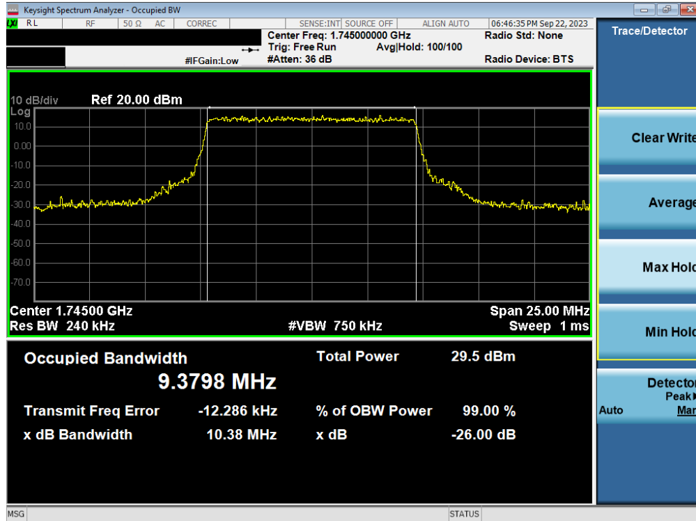
Plot 7-75. Occupied Bandwidth Plot (NR Band n66 - 10.0MHz CP-OFDM 16QAM - Full RB – ANT1)
