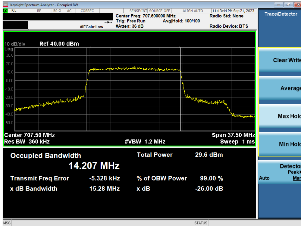
Plot 7-34. Occupied Bandwidth Plot (NR Band n12 - 15MHz CP-OFDM QPSK - Full RB – ANT1)
