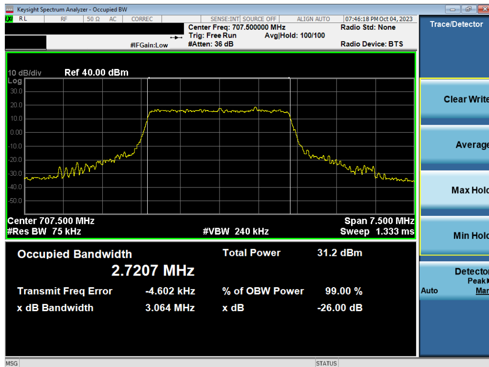
Plot 7-101. Occupied Bandwidth Plot (LTE Band 12 - 3MHz 16-QAM - Full RB – ANT2)
