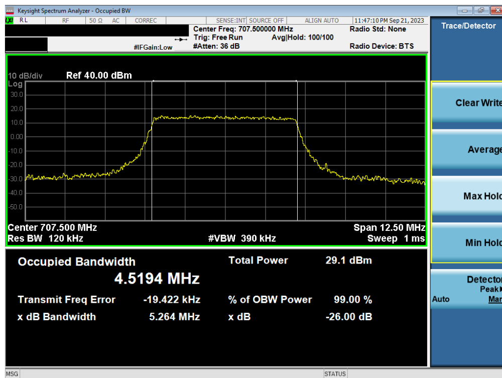
Plot 7-41. Occupied Bandwidth Plot (NR Band n12 - 5MHz CP-OFDM 16-QAM - Full RB – ANT1)
