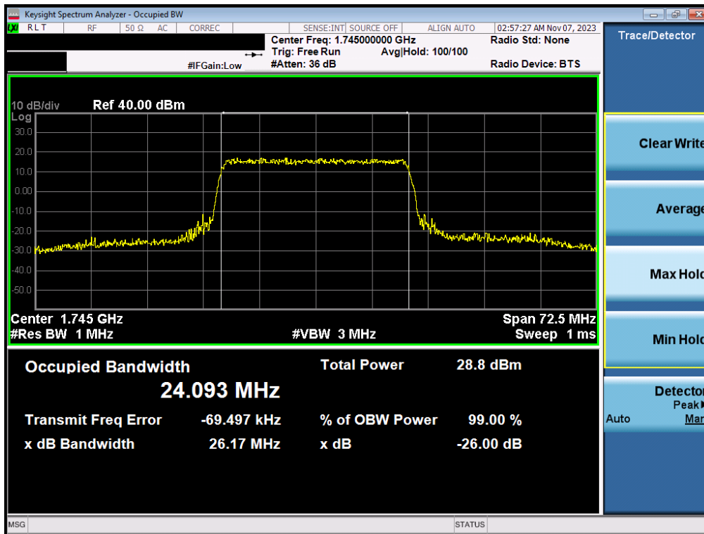
Plot 7-66. Occupied Bandwidth Plot (NR Band n66 - 25.0MHz CP-OFDM 16QAM - Full RB – ANT1)
