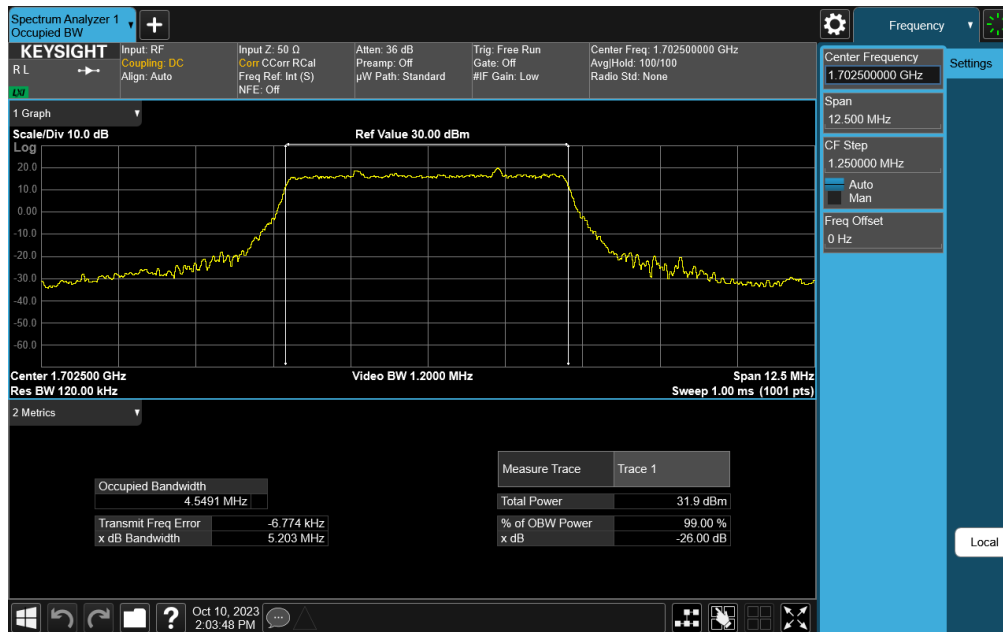
Plot 7-85. Occupied Bandwidth Plot (NR Band n70 - 5.0MHz DFT-s-OFDM BPSK - Full RB – ANT1)
