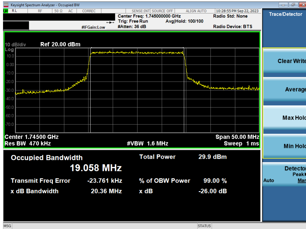
Plot 7-69. Occupied Bandwidth Plot (NR Band n66 - 20.0MHz CP-OFDM 16QAM - Full RB – ANT1)
