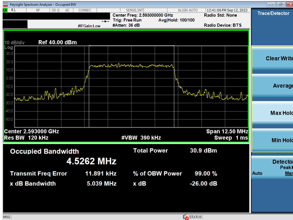
Plot 7-28. Occupied Bandwidth Plot (LTE Band 41(PC3)/38 - 5MHz 16-QAM - Full RB - Ant1)
