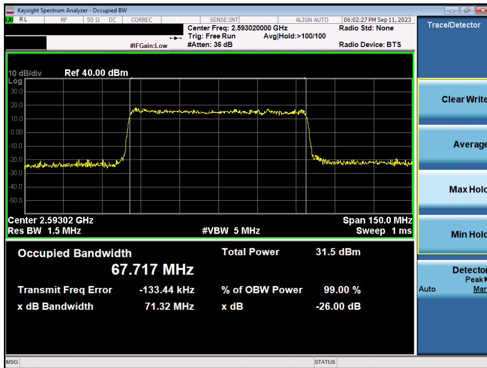
Plot 7-70. Occupied Bandwidth Plot (NR Band n41 - 70MHz 16-QAM - Full RB Configuration - Ant1)
