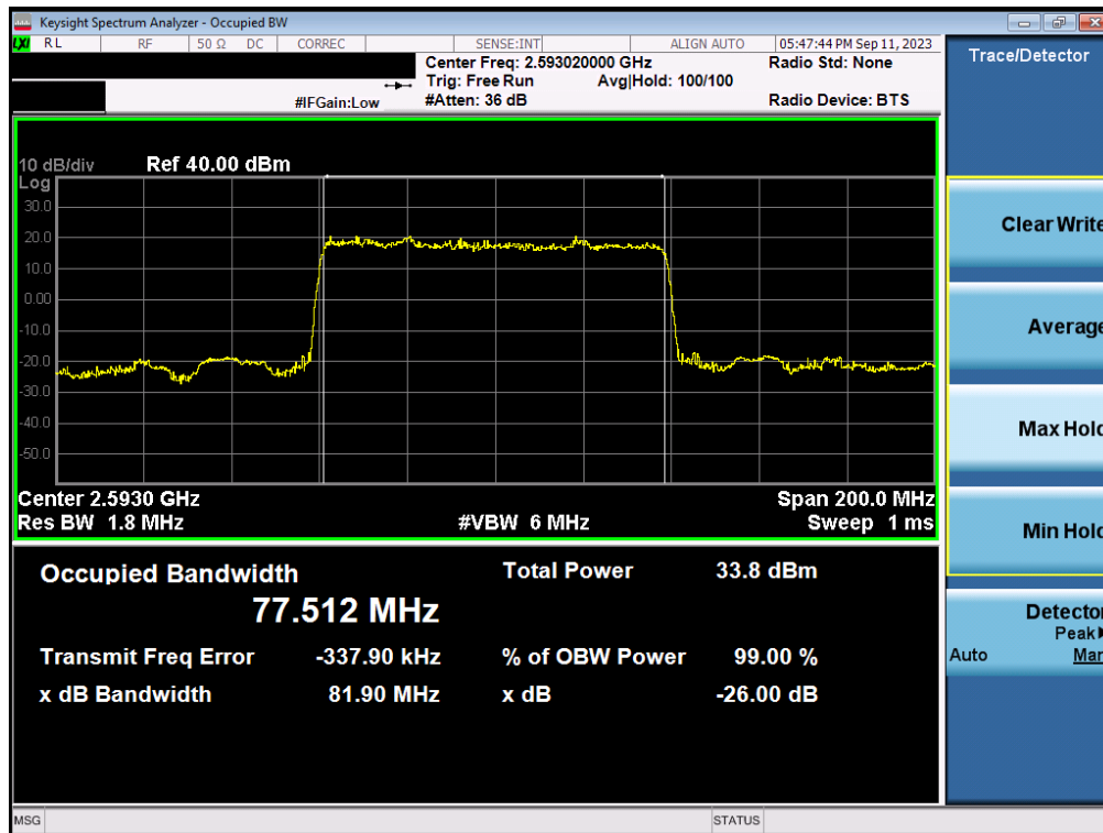
Plot 7-65. Occupied Bandwidth Plot (NR Band n41 - 80MHz \pi/2 BPSK - Full RB Configuration - Ant1)
