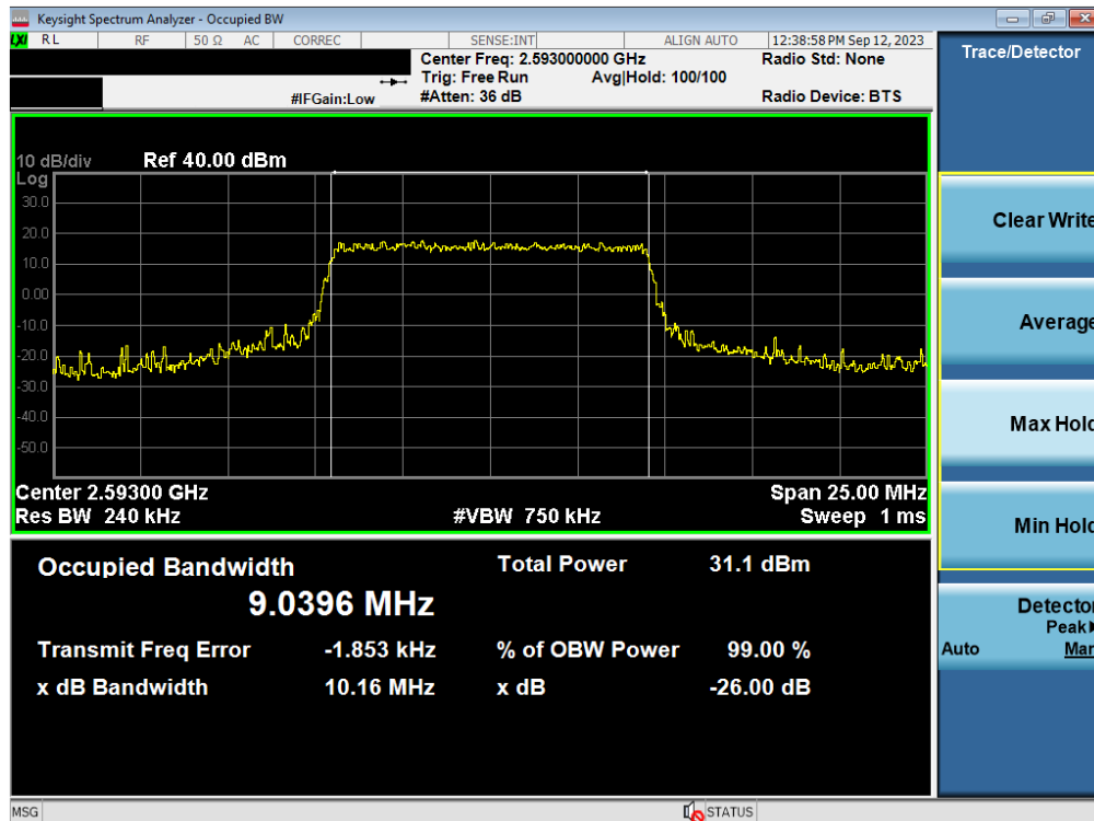
Plot 7-26. Occupied Bandwidth Plot (LTE Band 41(PC3)/38 - 10MHz 16-QAM - Full RB - Ant1)
