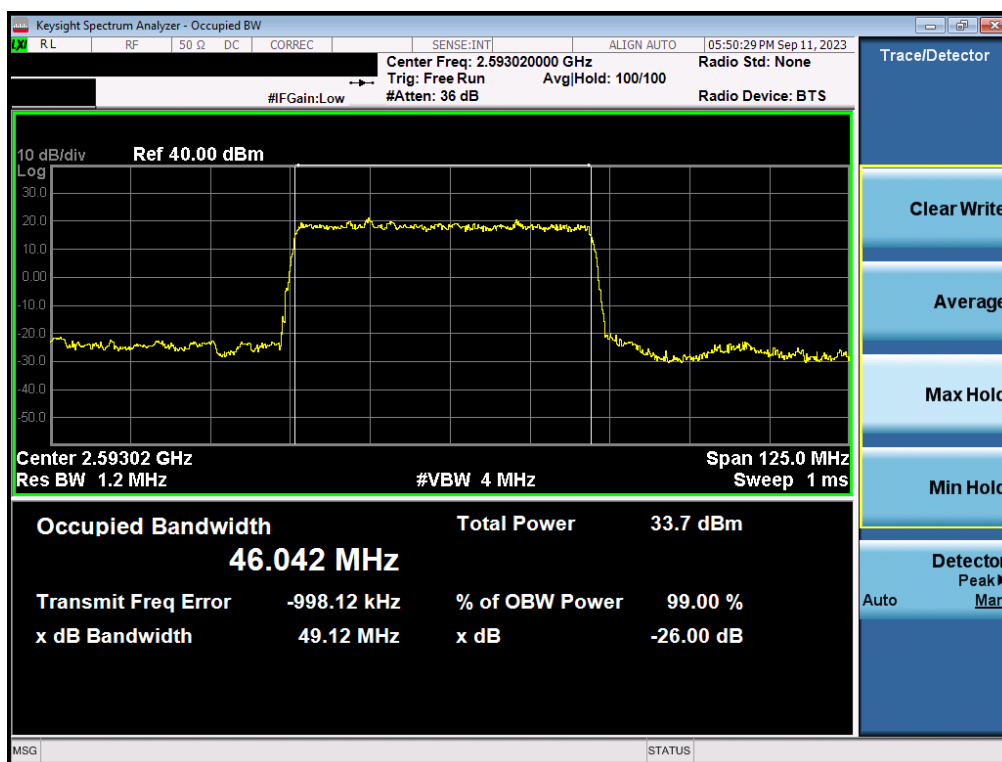
Plot 7-74. Occupied Bandwidth Plot (NR Band n41 - 50MHz \pi/2 BPSK - Full RB Configuration - Ant1)
