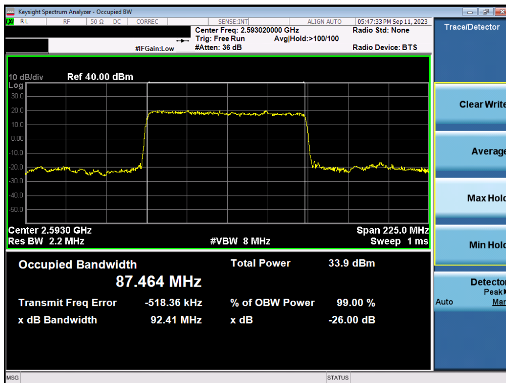
Plot 7-62. Occupied Bandwidth Plot (NR Band n41 - 90MHz \pi/2 BPSK - Full RB Configuration - Ant1)
