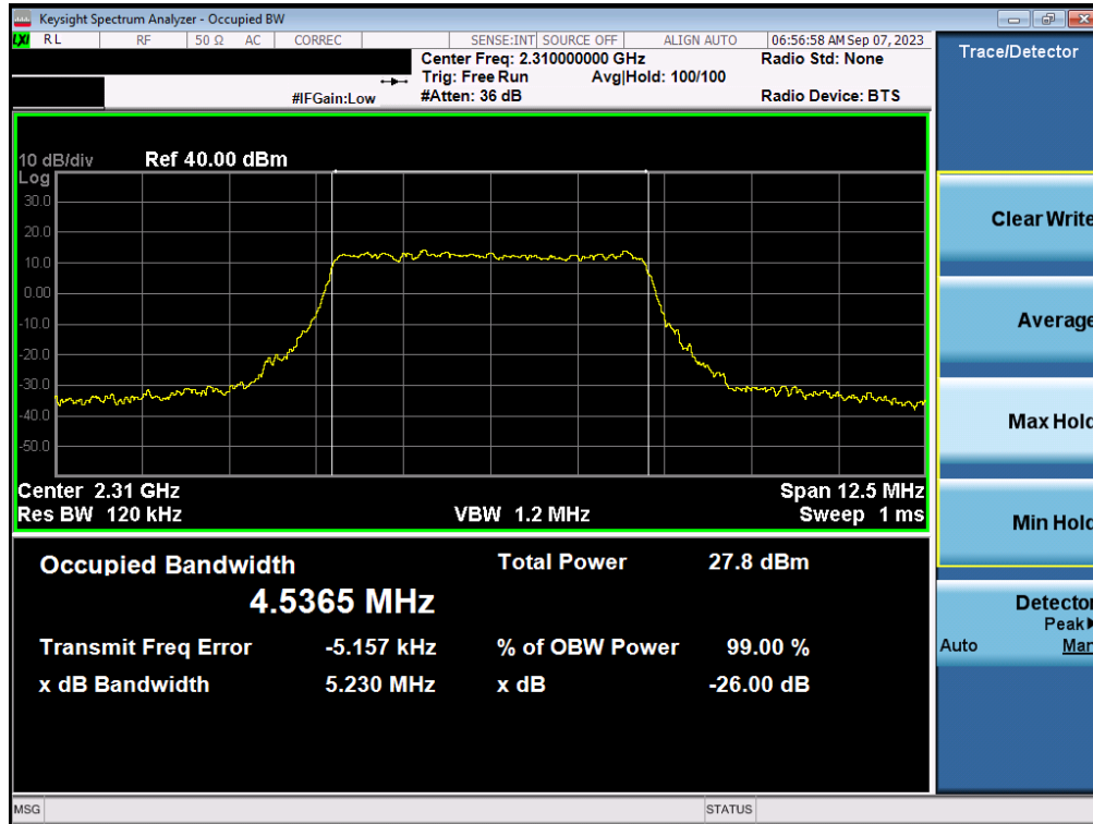
Plot 7-33. Occupied Bandwidth Plot (NR Band n30 - 5MHz QPSK - Full RB - Ant1)
