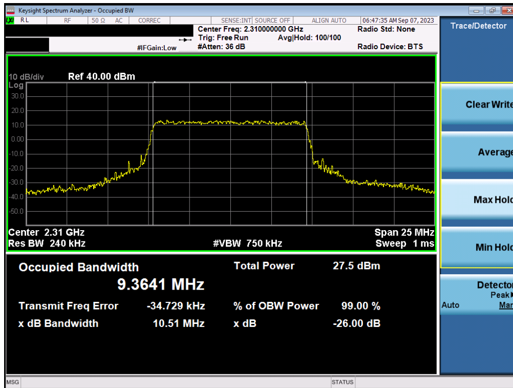
Plot 7-31. Occupied Bandwidth Plot (NR Band n30 - 10MHz 16-QAM - Full RB - Ant1)
