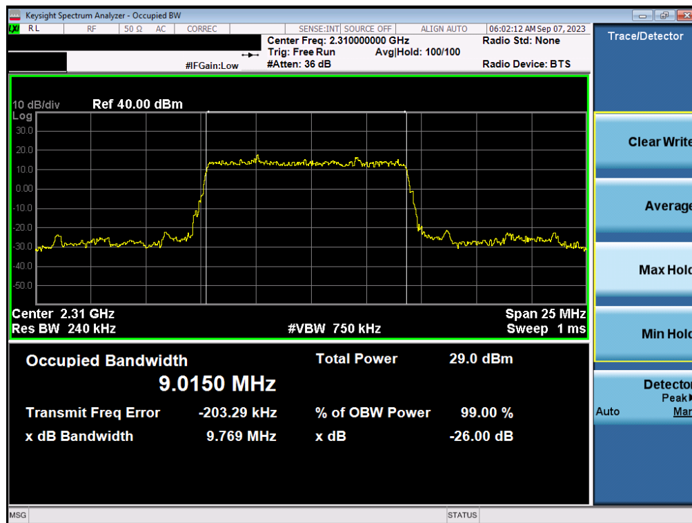
Plot 7-29. Occupied Bandwidth Plot (NR Band n30 - 10MHz \pi/2 BPSK - Full RB - Ant1)
