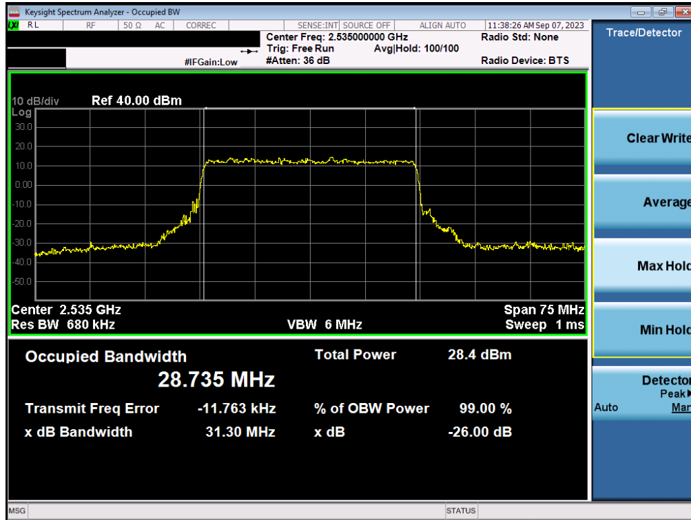
Plot 7-43. Occupied Bandwidth Plot (NR Band n7 - 30MHz 16-QAM - Full RB - Ant1)
