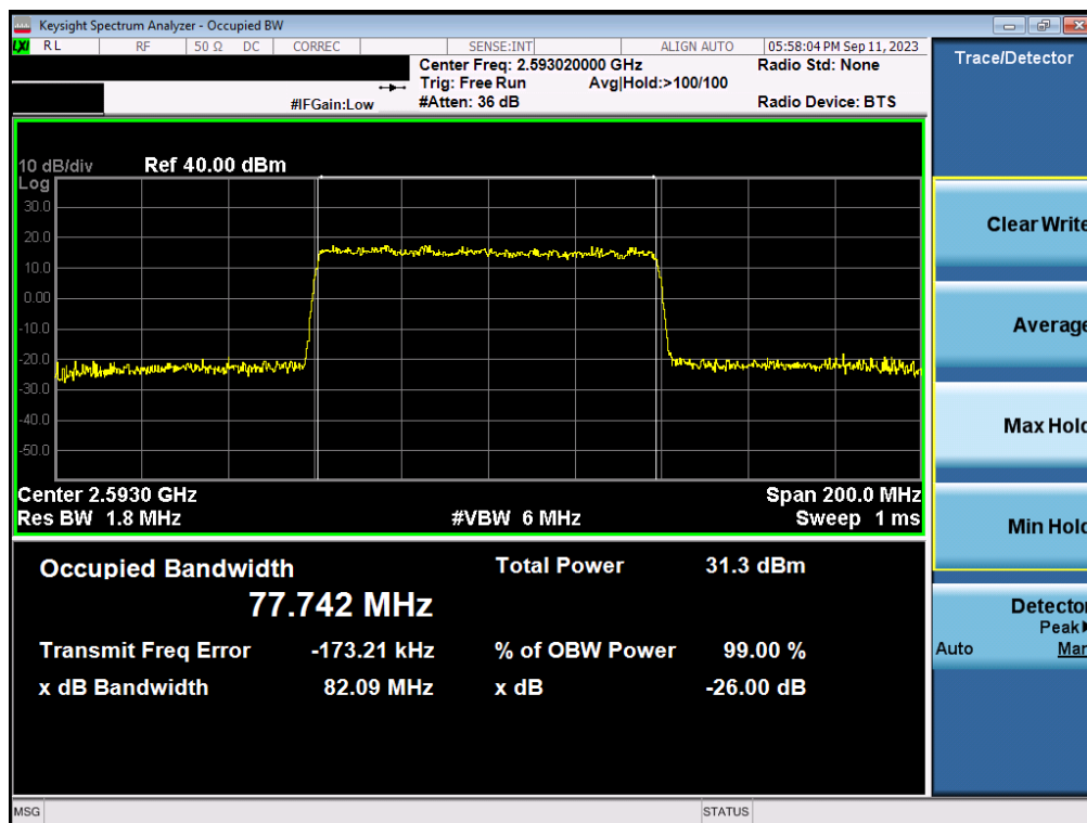
Plot 7-66. Occupied Bandwidth Plot (NR Band n41 - 80MHz QPSK - Full RB Configuration - Ant1)
