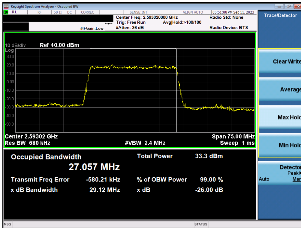
Plot 7-80. Occupied Bandwidth Plot (NR Band n41 - 30MHz \pi/2 BPSK - Full RB Configuration - Ant1)
