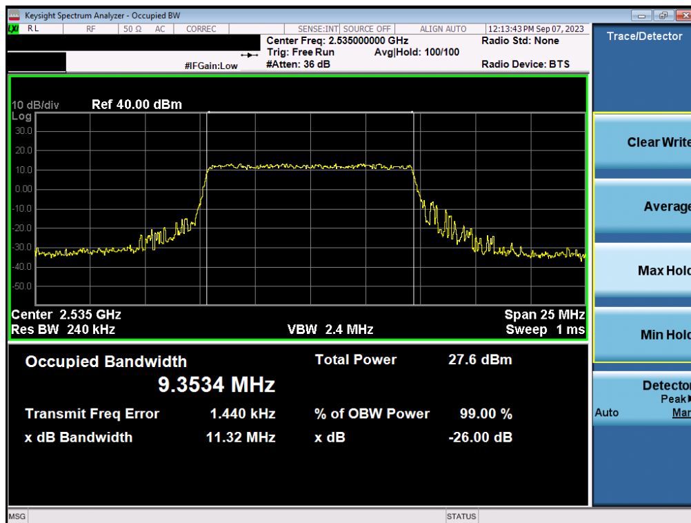
Plot 7-54. Occupied Bandwidth Plot (NR Band n7 - 10MHz QPSK - Full RB - Ant1)
