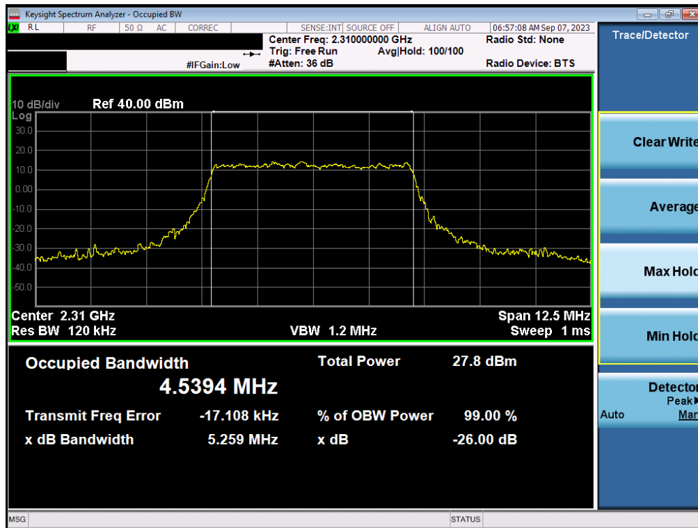
Plot 7-34. Occupied Bandwidth Plot (NR Band n30 - 5MHz 16-QAM - Full RB - Ant1)
