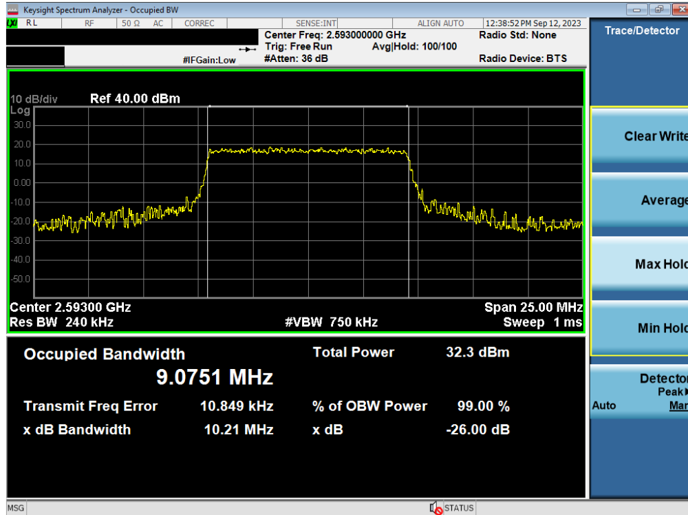
Plot 7-25. Occupied Bandwidth Plot (LTE Band 41(PC3)/38 - 10MHz QPSK - Full RB - Ant1)
