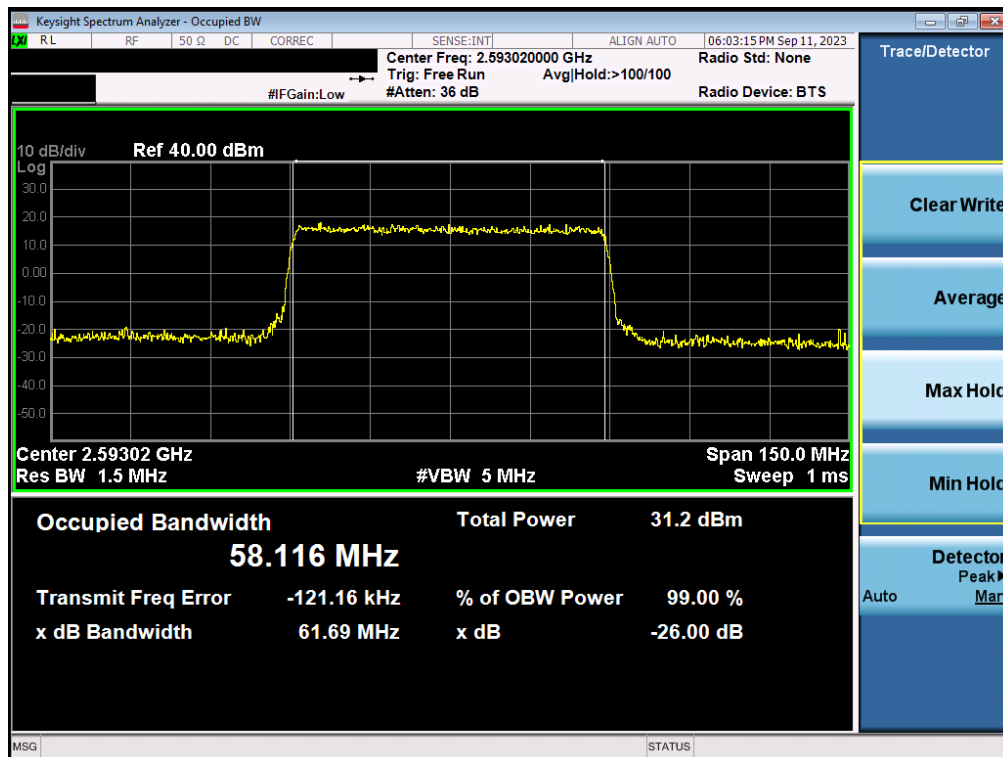
Plot 7-72. Occupied Bandwidth Plot (NR Band n41 - 60MHz QPSK - Full RB Configuration - Ant1)
