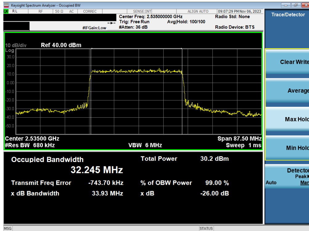
Plot 7-38. Occupied Bandwidth Plot (NR Band n7 - 35MHz \pi/2 BPSK - Full RB - Ant1)
