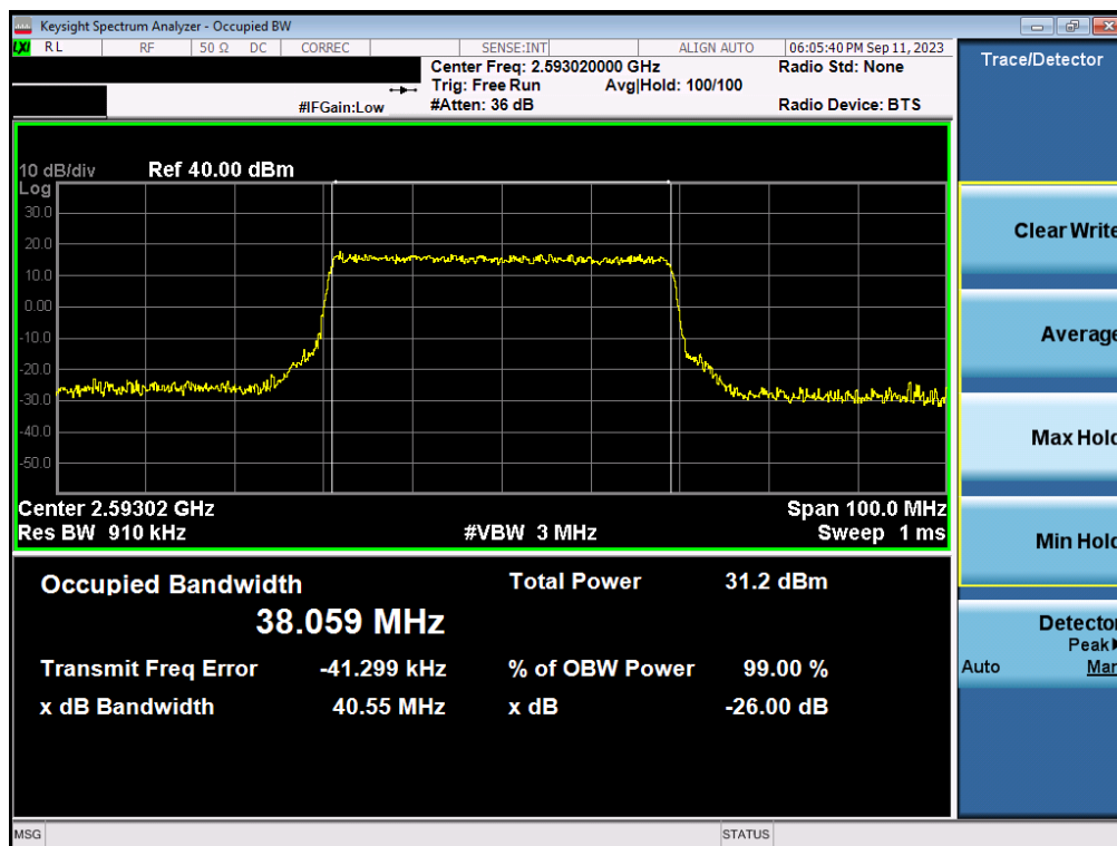
Plot 7-78. Occupied Bandwidth Plot (NR Band n41 - 40MHz QPSK - Full RB Configuration - Ant1)
