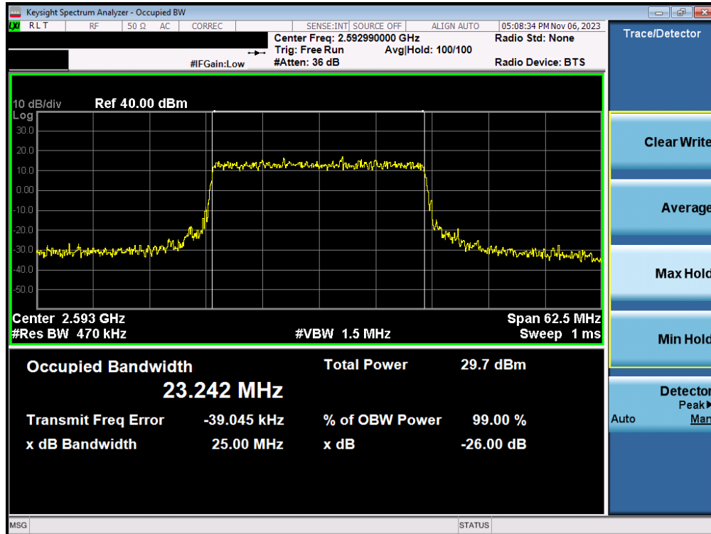
Plot 7-85. Occupied Bandwidth Plot (NR Band n41 - 25MHz 16-QAM - Full RB Configuration - Ant1)
