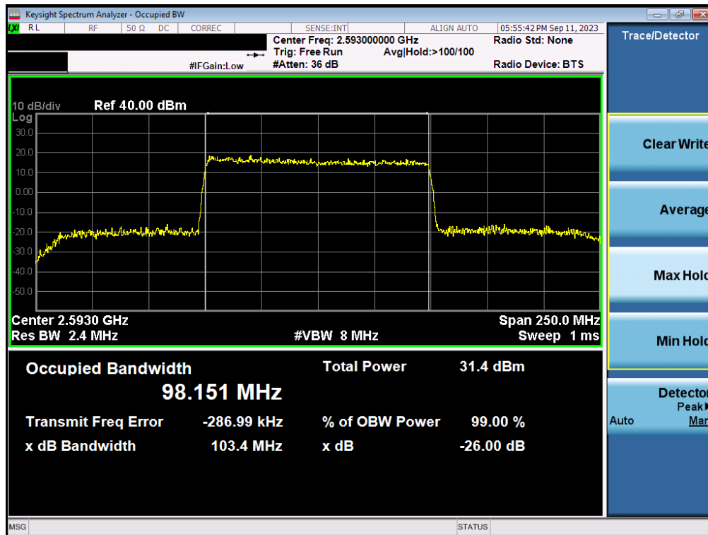
Plot 7-61. Occupied Bandwidth Plot (NR Band n41 - 100MHz 16-QAM - Full RB Configuration - Ant1)
