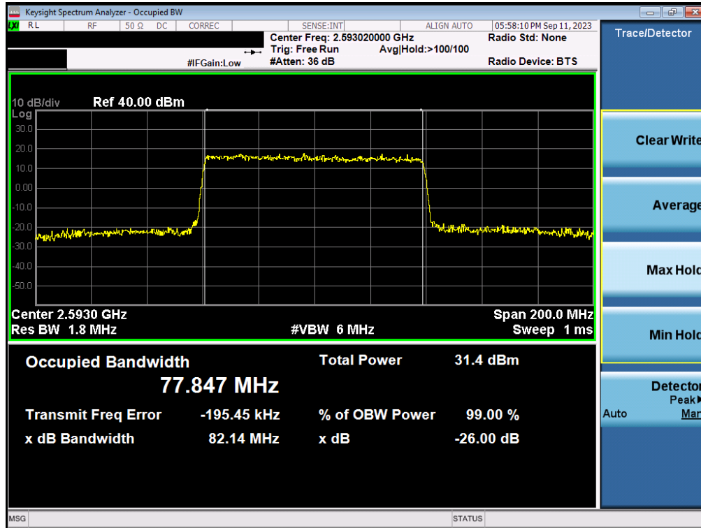
Plot 7-67. Occupied Bandwidth Plot (NR Band n41 - 80MHz 16-QAM - Full RB Configuration - Ant1)
