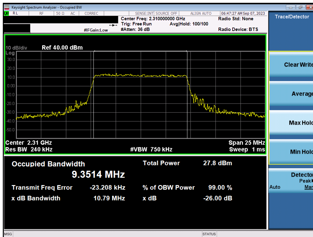
Plot 7-30. Occupied Bandwidth Plot (NR Band n30 - 10MHz QPSK - Full RB - Ant1)
