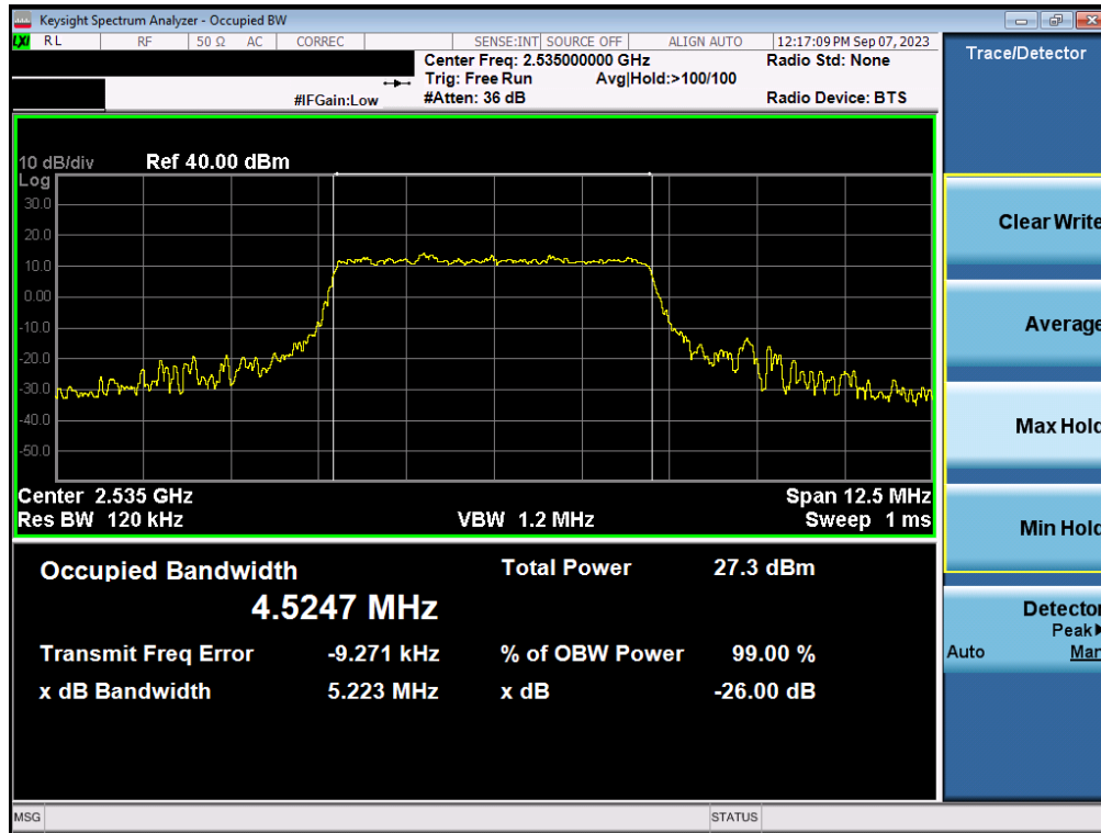
Plot 7-58. Occupied Bandwidth Plot (NR Band n7 - 5MHz 16-QAM - Full RB - Ant1)
