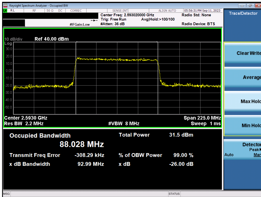
Plot 7-64. Occupied Bandwidth Plot (NR Band n41 - 90MHz 16-QAM - Full RB Configuration - Ant1)
