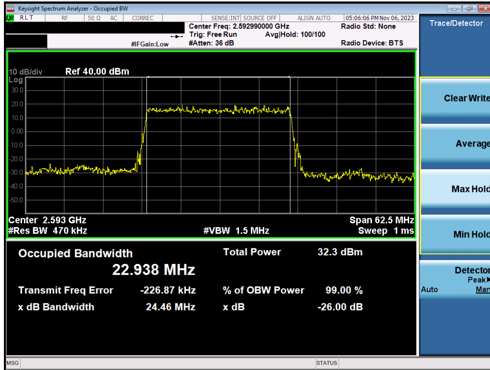
Plot 7-83. Occupied Bandwidth Plot (NR Band n41 - 25MHz \pi/2 BPSK - Full RB Configuration - Ant1)
