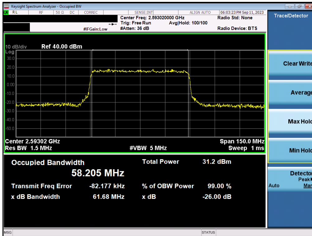
Plot 7-73. Occupied Bandwidth Plot (NR Band n41 - 60MHz 16-QAM - Full RB Configuration - Ant1)
