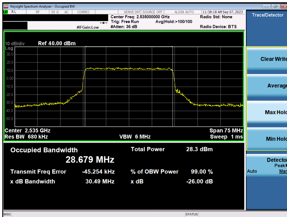
Plot 7-42. Occupied Bandwidth Plot (NR Band n7 - 30MHz QPSK - Full RB - Ant1)
