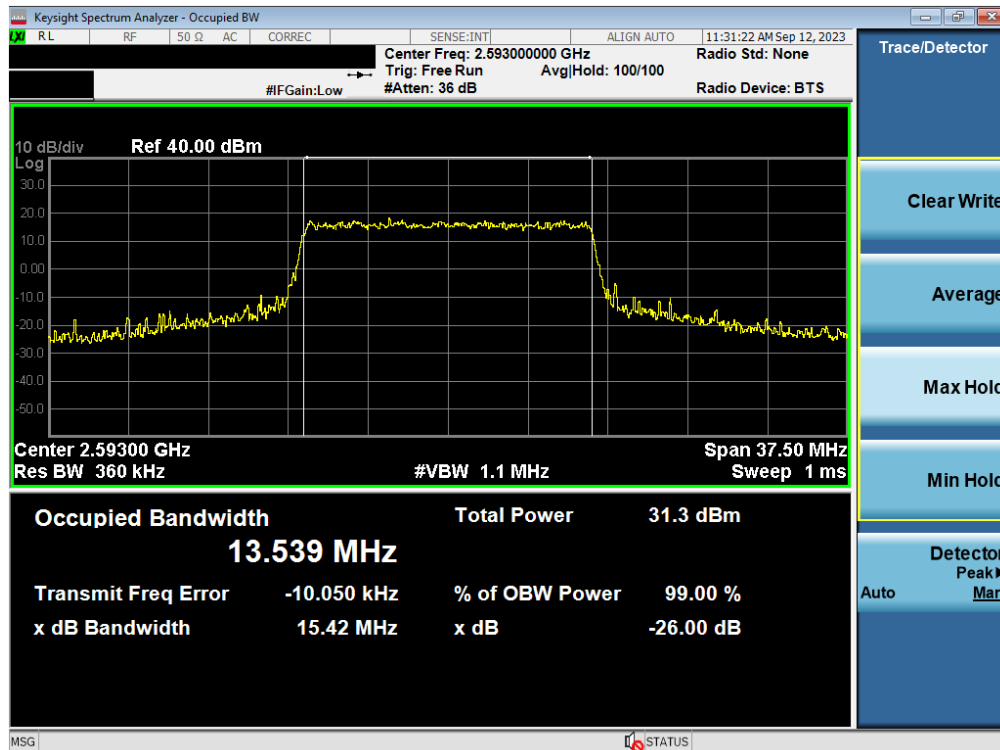
Plot 7-24. Occupied Bandwidth Plot (LTE Band 41(PCI3)/38 - 15MHz 16-QAM - Full RB - Ant1)
