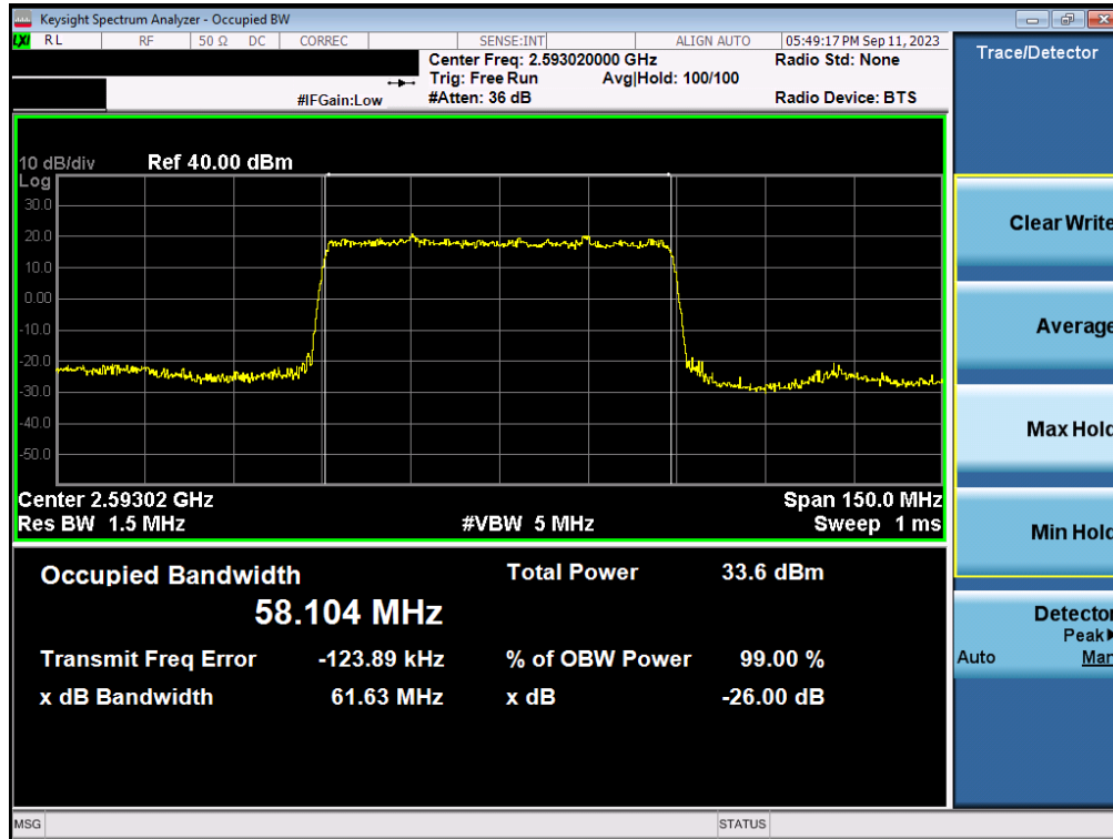
Plot 7-71. Occupied Bandwidth Plot (NR Band n41 - 60MHz \pi/2 BPSK - Full RB Configuration - Ant1)
