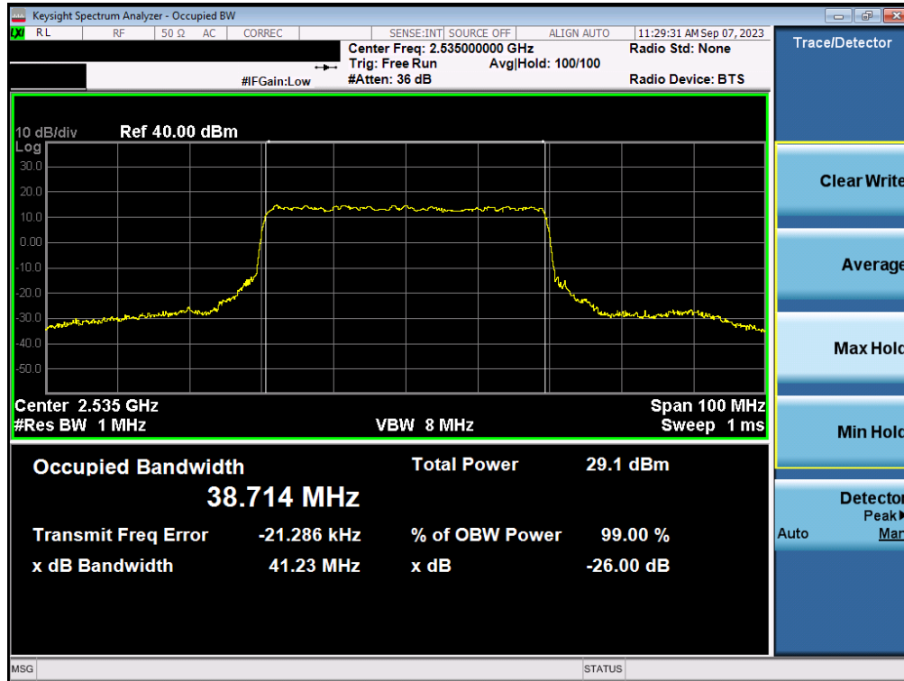
Plot 7-37. Occupied Bandwidth Plot (NR Band n7 - 40MHz 16-QAM - Full RB - Ant1)
