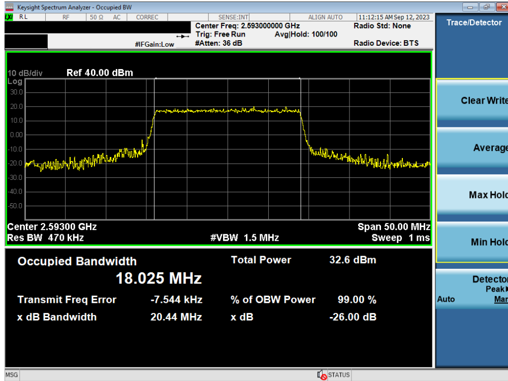
Plot 7-21. Occupied Bandwidth Plot (LTE Band 41(PC3)/38 - 20MHz QPSK - Full RB - Ant1)
