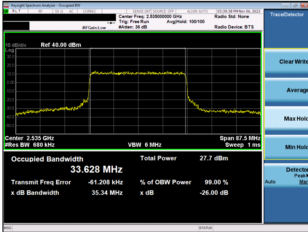
Plot 7-39. Occupied Bandwidth Plot (NR Band n7 - 35MHz QPSK - Full RB - Ant1)
