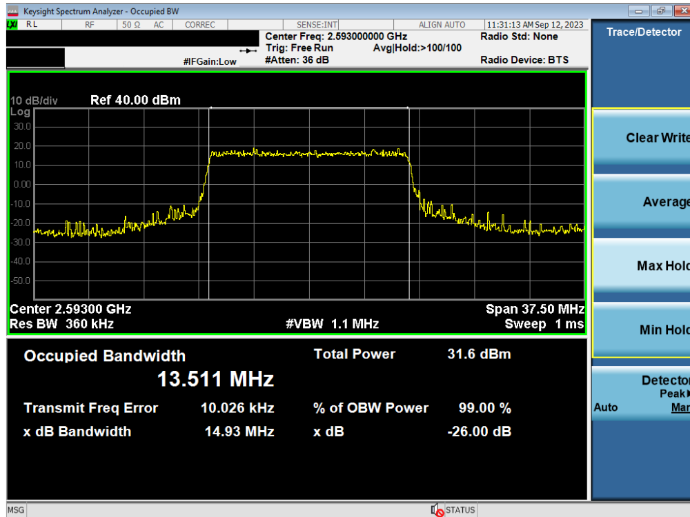
Plot 7-23. Occupied Bandwidth Plot (LTE Band 41(PCI3)/38 - 15MHz QPSK - Full RB - Ant1)
