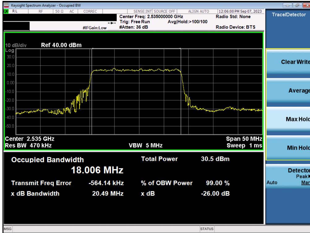
Plot 7-47. Occupied Bandwidth Plot (NR Band n7 - 20MHz \pi/2 BPSK - Full RB - Ant1)
