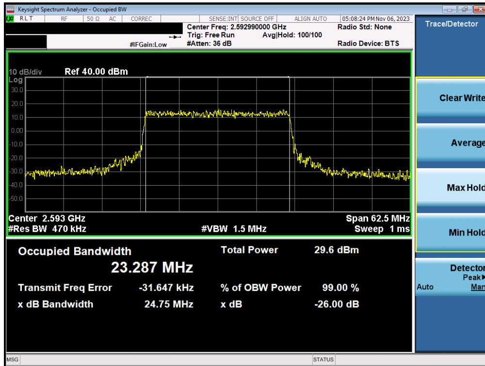
Plot 7-84. Occupied Bandwidth Plot (NR Band n41 - 25MHz QPSK - Full RB Configuration - Ant1)
