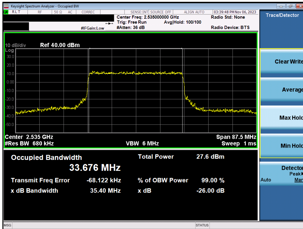
Plot 7-40. Occupied Bandwidth Plot (NR Band n7 - 35MHz 16-QAM - Full RB - Ant1)
