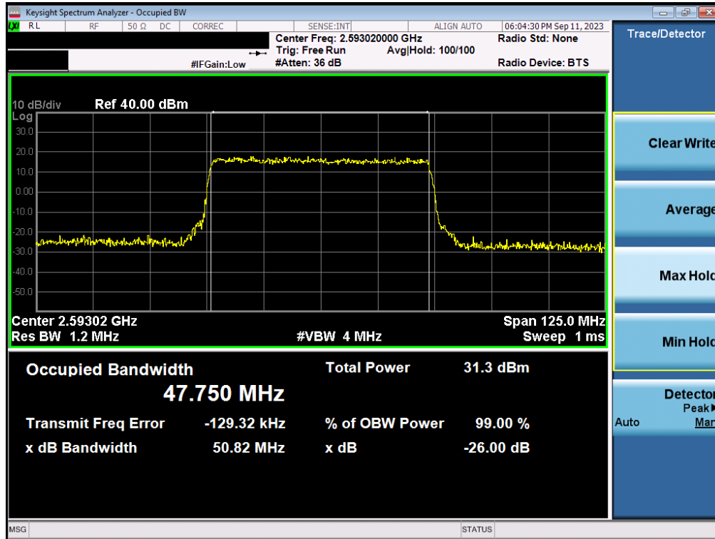
Plot 7-75. Occupied Bandwidth Plot (NR Band n41 - 50MHz QPSK - Full RB Configuration - Ant1)
