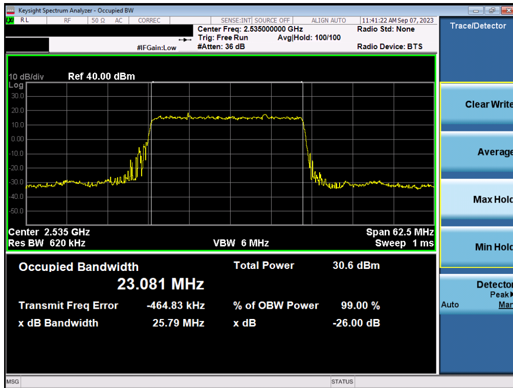
Plot 7-44. Occupied Bandwidth Plot (NR Band n7 - 25MHz \pi/2 BPSK - Full RB - Ant1)
