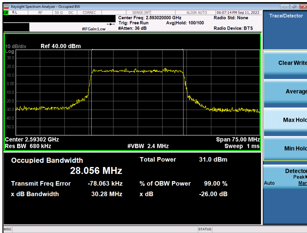
Plot 7-82. Occupied Bandwidth Plot (NR Band n41 - 30MHz 16-QAM - Full RB Configuration - Ant1)
