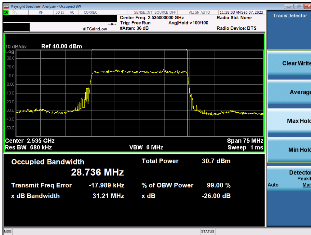
Plot 7-41. Occupied Bandwidth Plot (NR Band n7 - 30MHz \pi/2 BPSK - Full RB - Ant1)
