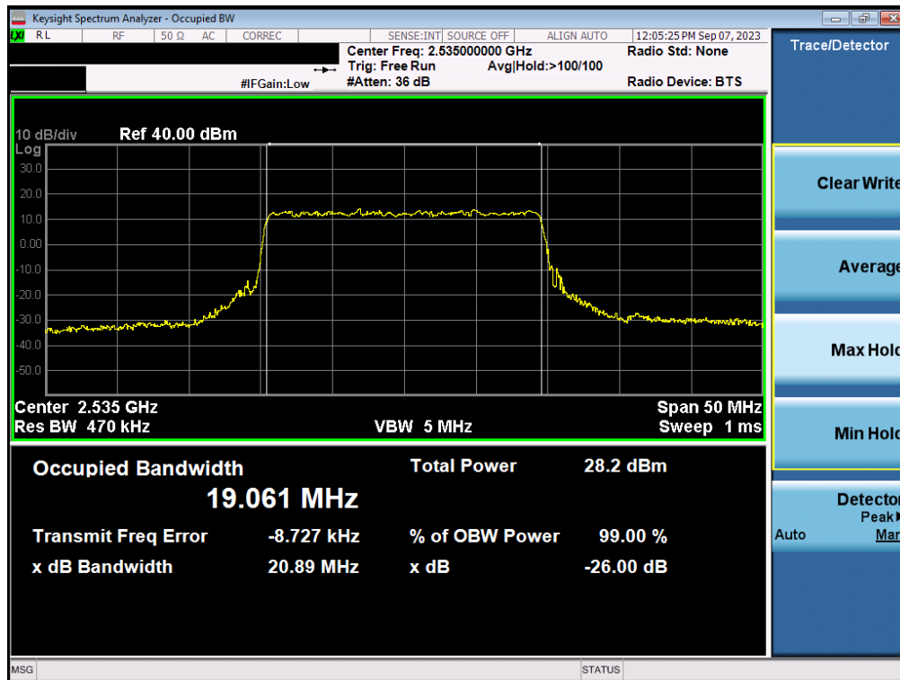
Plot 7-49. Occupied Bandwidth Plot (NR Band n7 - 20MHz 16-QAM - Full RB - Ant1)
