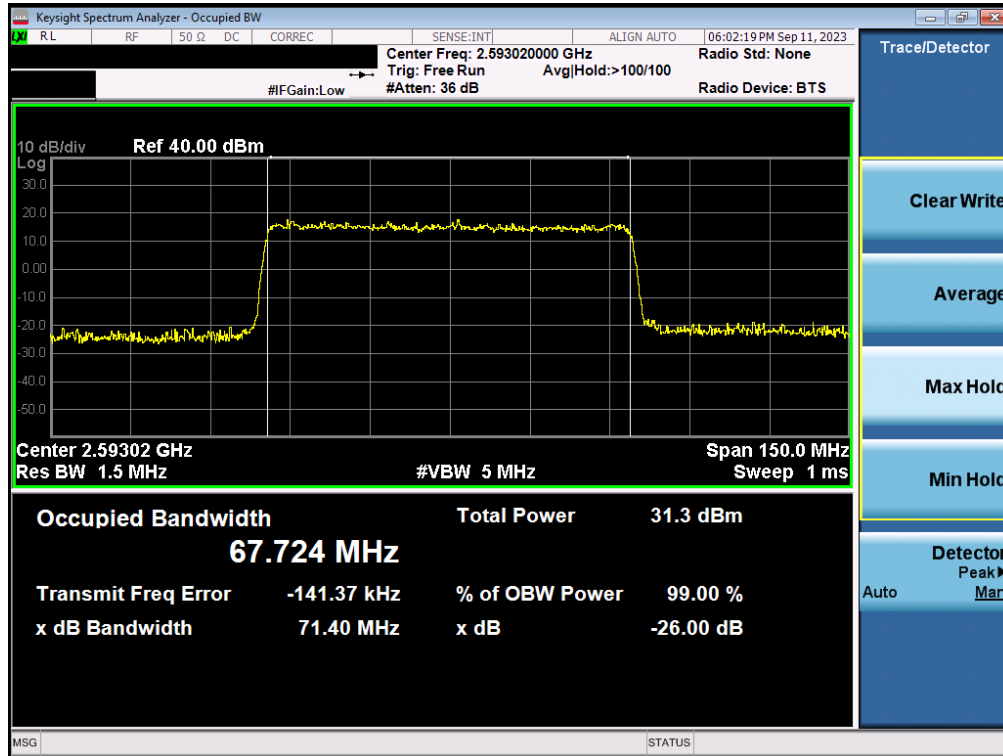
Plot 7-69. Occupied Bandwidth Plot (NR Band n41 - 70MHz QPSK - Full RB Configuration - Ant1)
