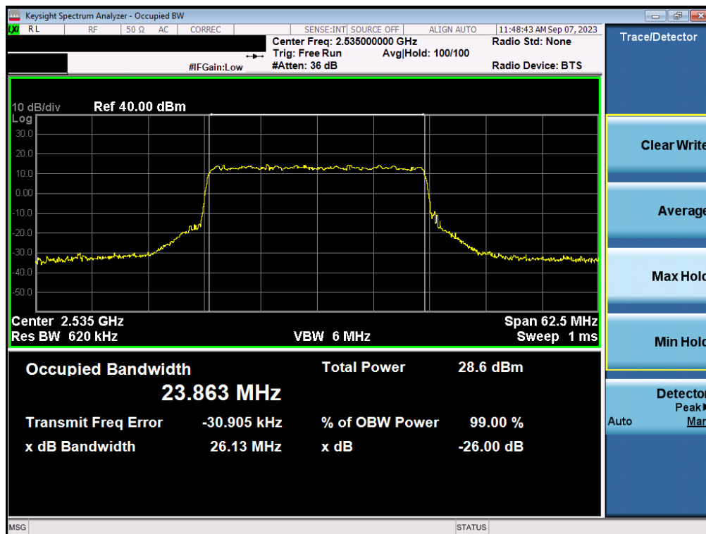
Plot 7-46. Occupied Bandwidth Plot (NR Band n7 - 25MHz 16-QAM - Full RB - Ant1)
