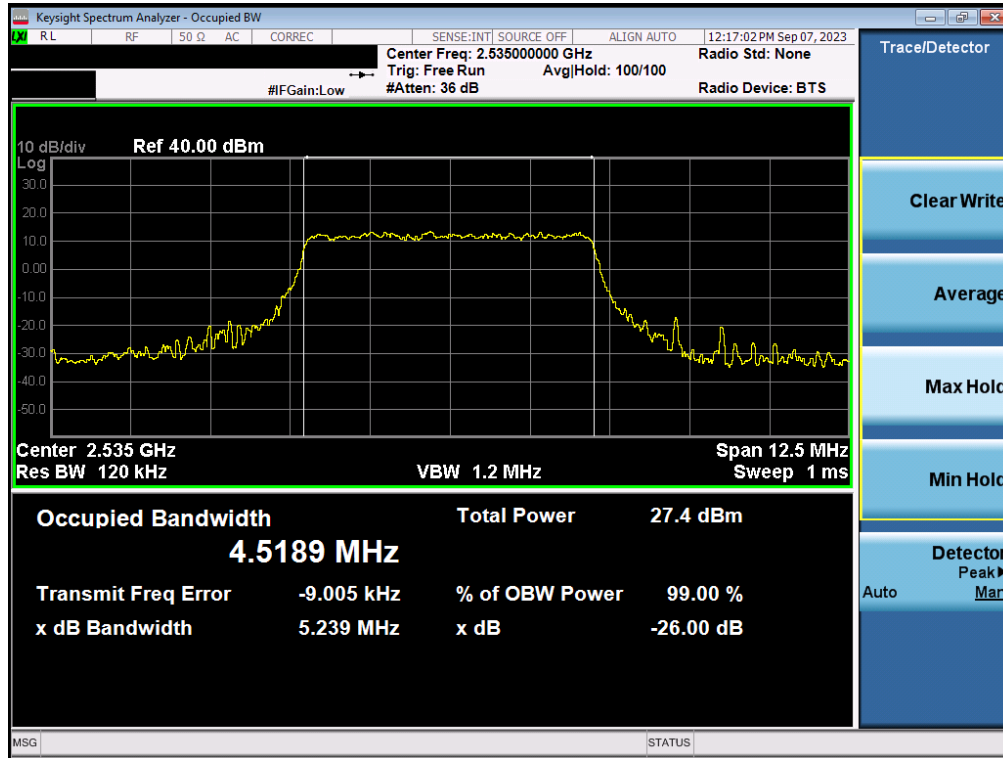
Plot 7-57. Occupied Bandwidth Plot (NR Band n7 - 5MHz QPSK - Full RB - Ant1)
