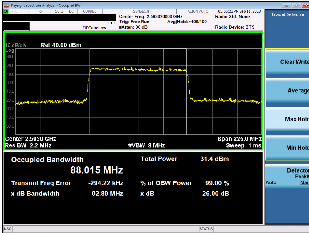
Plot 7-63. Occupied Bandwidth Plot (NR Band n41 - 90MHz QPSK - Full RB Configuration - Ant1)
