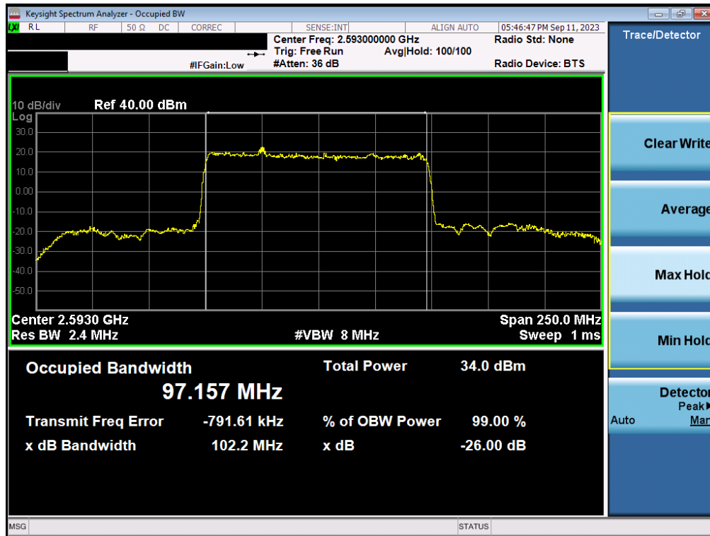
Plot 7-59. Occupied Bandwidth Plot (NR Band n41 - 100MHz \pi/2 BPSK - Full RB Configuration - Ant1)
