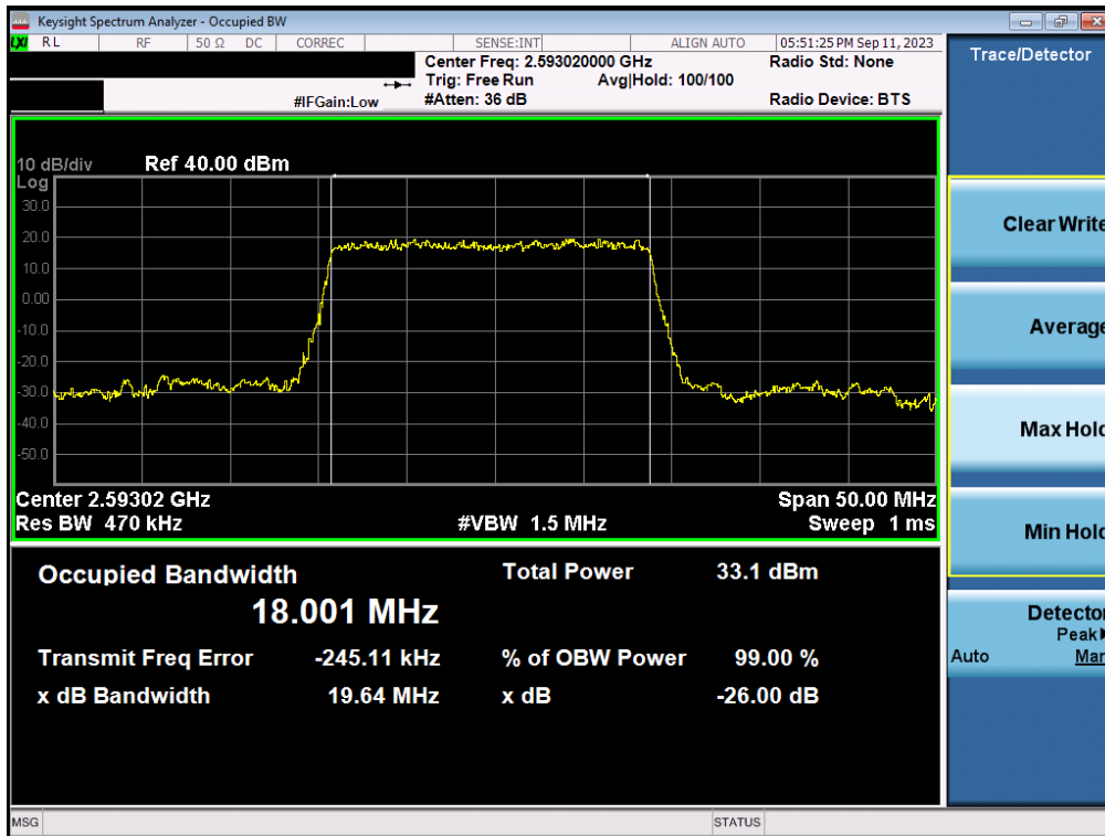
Plot 7-86. Occupied Bandwidth Plot (NR Band n41 - 20MHz \pi/2 BPSK - Full RB Configuration - Ant1)
