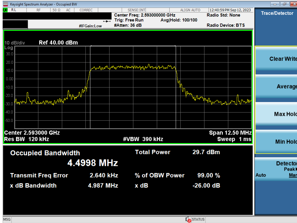
Plot 7-27. Occupied Bandwidth Plot (LTE Band 41(PC3)/38 - 5MHz QPSK - Full RB - Ant1)
