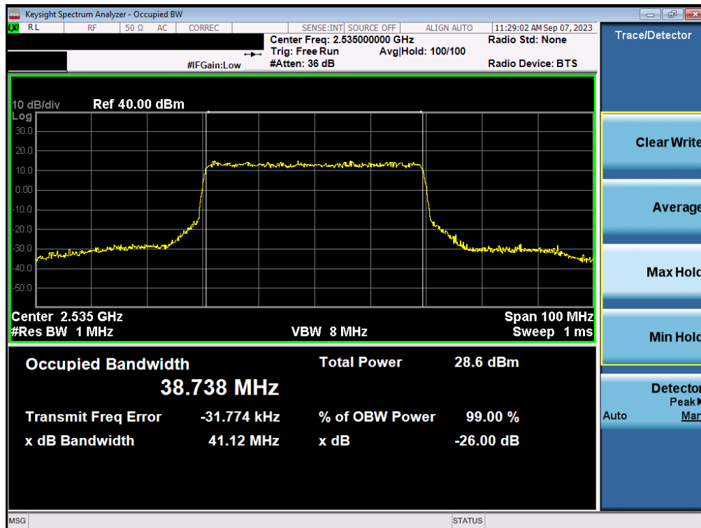
Plot 7-36. Occupied Bandwidth Plot (NR Band n7 - 40MHz QPSK - Full RB - Ant1)
