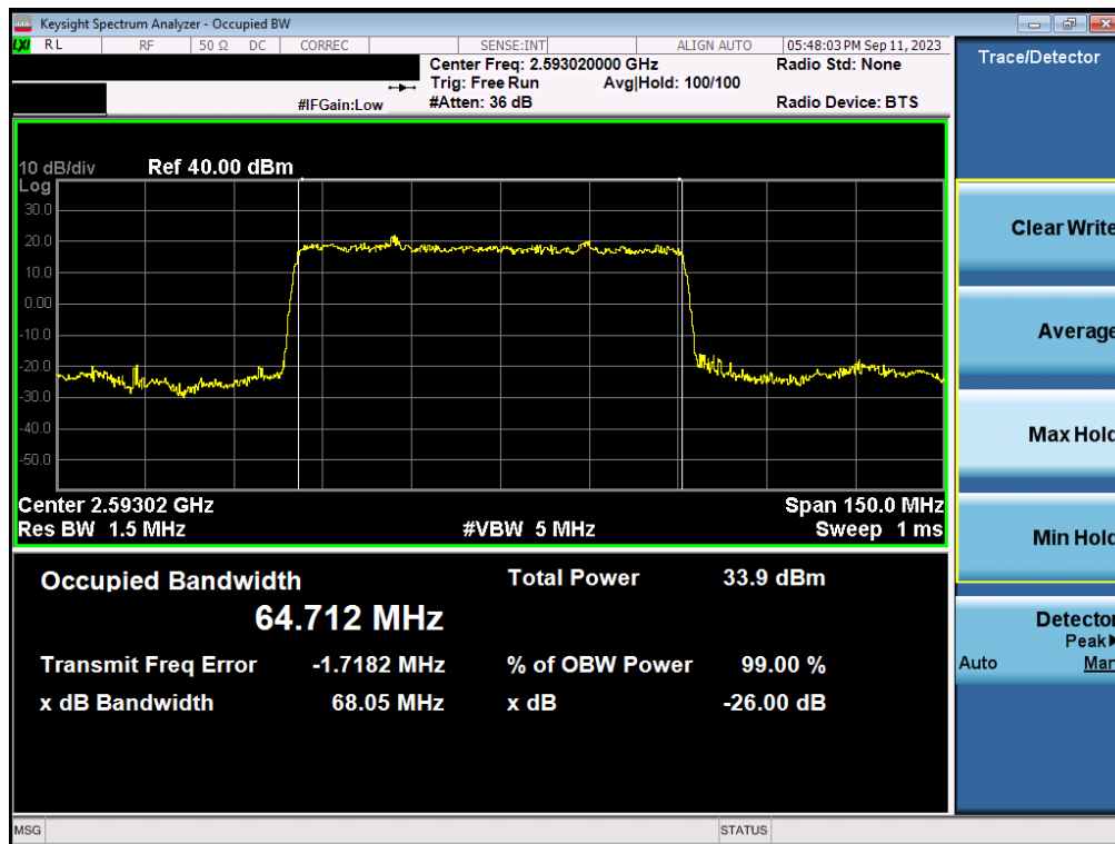
Plot 7-68. Occupied Bandwidth Plot (NR Band n41 - 70MHz \pi/2 BPSK - Full RB Configuration - Ant1)
