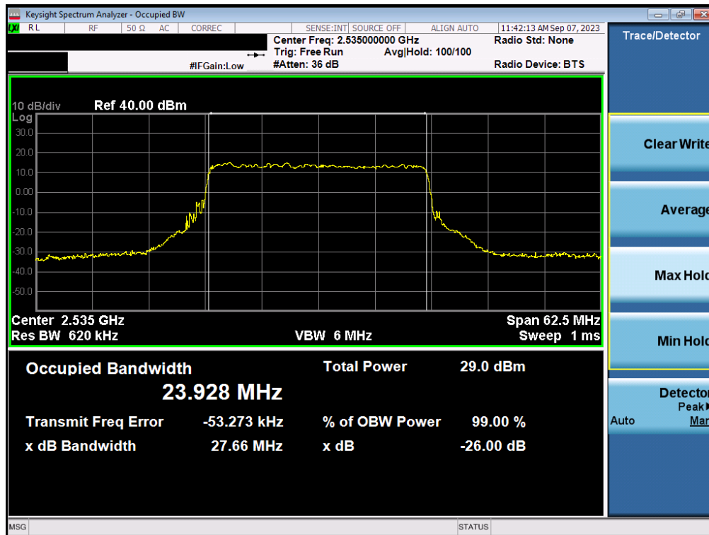
Plot 7-45. Occupied Bandwidth Plot (NR Band n7 - 25MHz QPSK - Full RB - Ant1)
