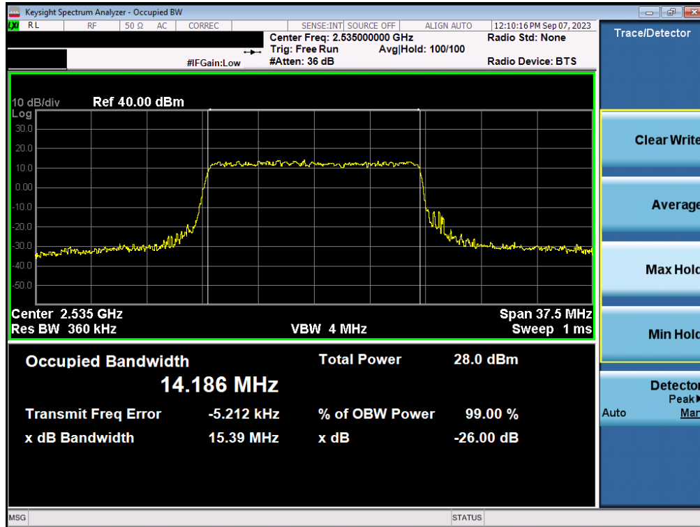
Plot 7-51. Occupied Bandwidth Plot (NR Band n7 - 15MHz QPSK - Full RB - Ant1)
