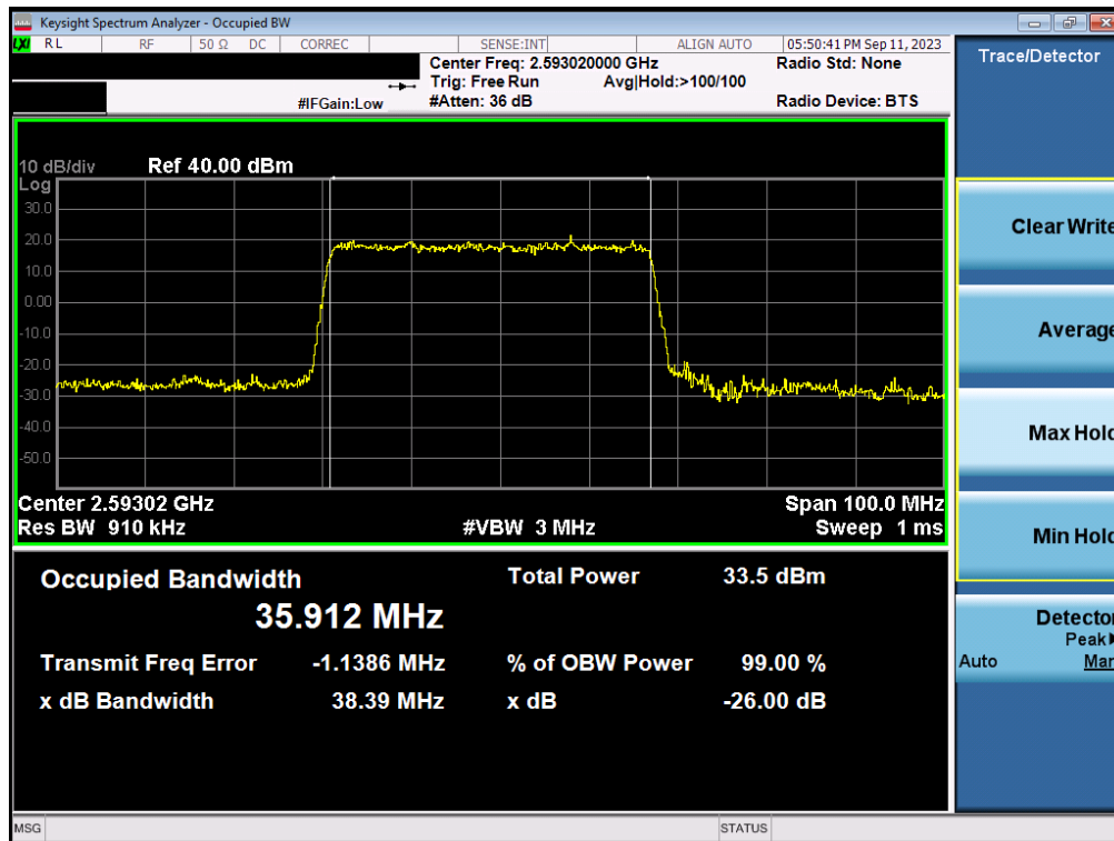
Plot 7-77. Occupied Bandwidth Plot (NR Band n41 - 40MHz \pi/2 BPSK - Full RB Configuration - Ant1)
