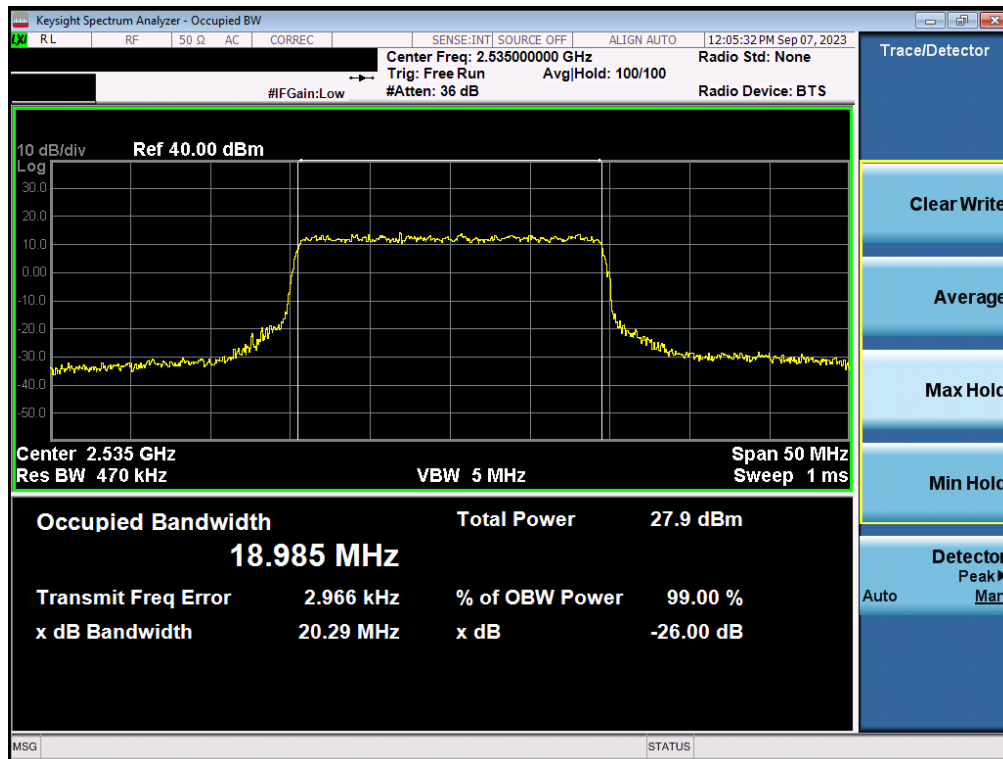
Plot 7-48. Occupied Bandwidth Plot (NR Band n7 - 20MHz QPSK - Full RB - Ant1)
