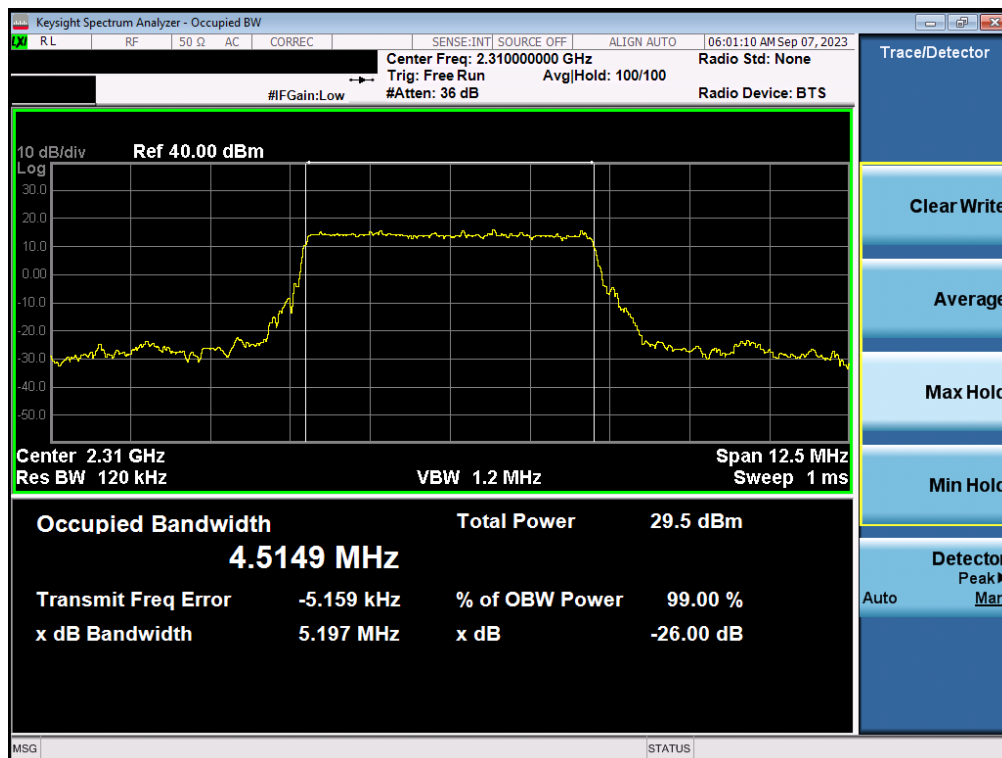
Plot 7-32. Occupied Bandwidth Plot (NR Band n30 - 5MHz \pi/2 BPSK - Full RB - Ant1)
