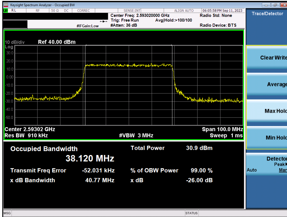
Plot 7-79. Occupied Bandwidth Plot (NR Band n41 - 40MHz 16-QAM - Full RB Configuration - Ant1)
