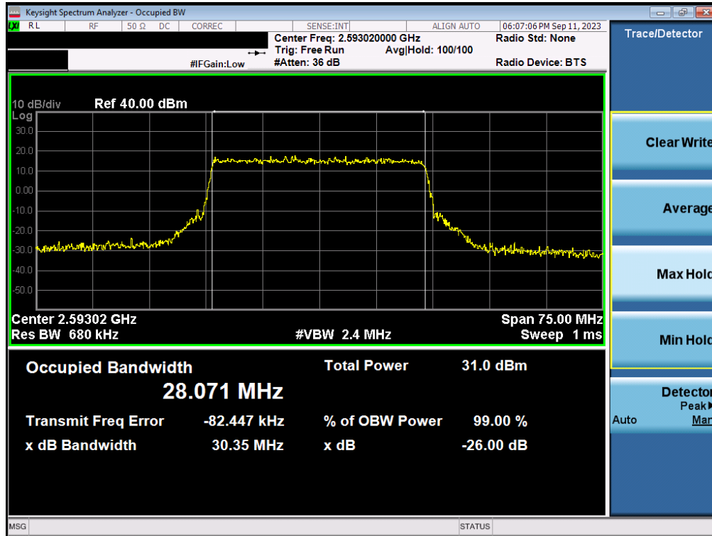
Plot 7-81. Occupied Bandwidth Plot (NR Band n41 - 30MHz QPSK - Full RB Configuration - Ant1)
