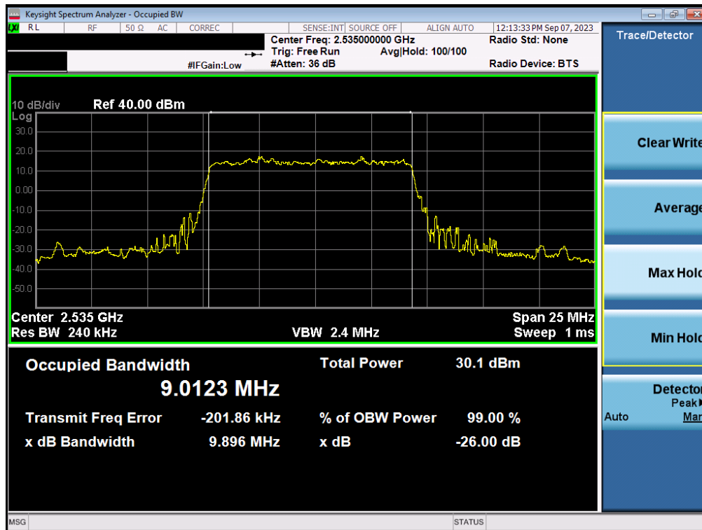
Plot 7-53. Occupied Bandwidth Plot (NR Band n7 - 10MHz \pi/2 BPSK - Full RB - Ant1)
