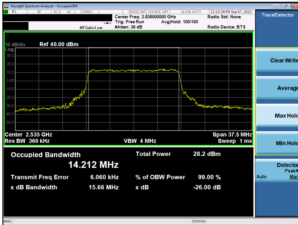
Plot 7-52. Occupied Bandwidth Plot (NR Band n7 - 15MHz 16-QAM - Full RB - Ant1)
