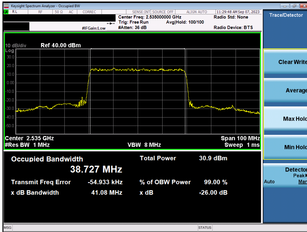
Plot 7-35. Occupied Bandwidth Plot (NR Band n7 - 40MHz \pi/2 BPSK - Full RB - Ant1)
