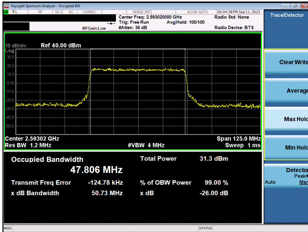
Plot 7-76. Occupied Bandwidth Plot (NR Band n41 - 50MHz 16-QAM - Full RB Configuration - Ant1)
