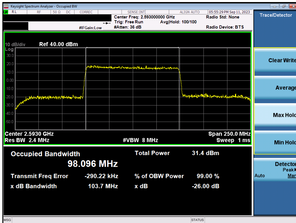
Plot 7-60. Occupied Bandwidth Plot (NR Band n41 - 100MHz QPSK - Full RB Configuration - Ant1)
