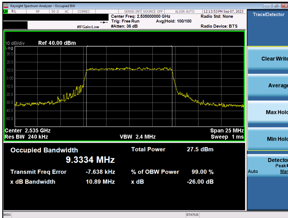
Plot 7-55. Occupied Bandwidth Plot (NR Band n7 - 10MHz 16-QAM - Full RB - Ant1)
