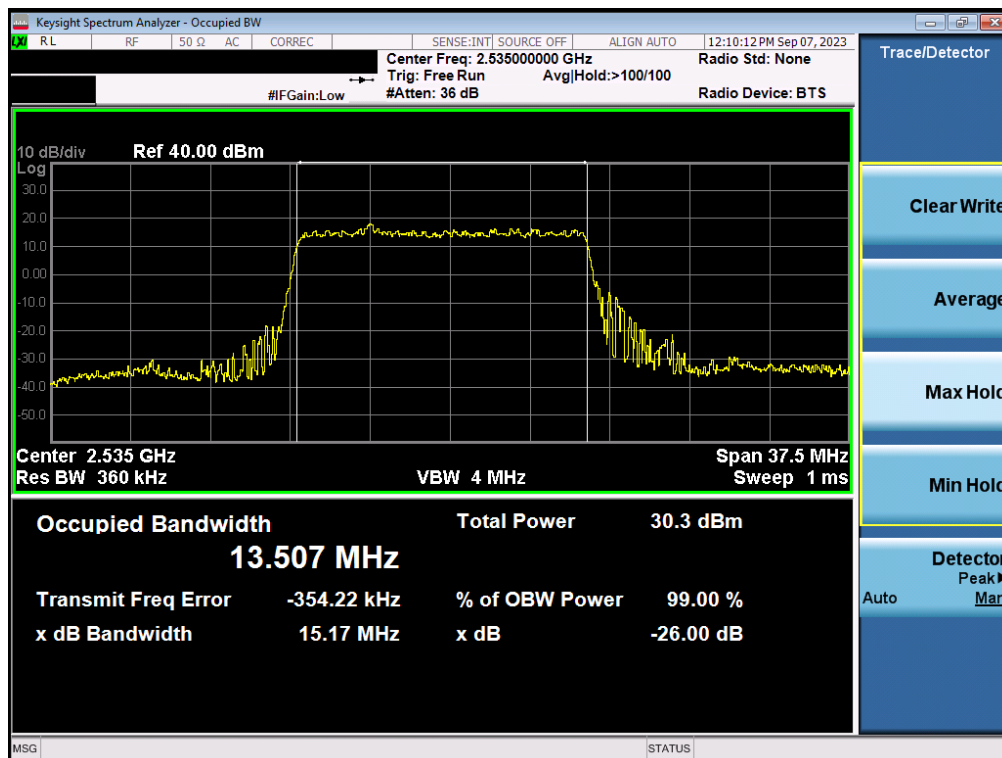
Plot 7-50. Occupied Bandwidth Plot (NR Band n7 - 15MHz \pi/2 BPSK - Full RB - Ant1)
