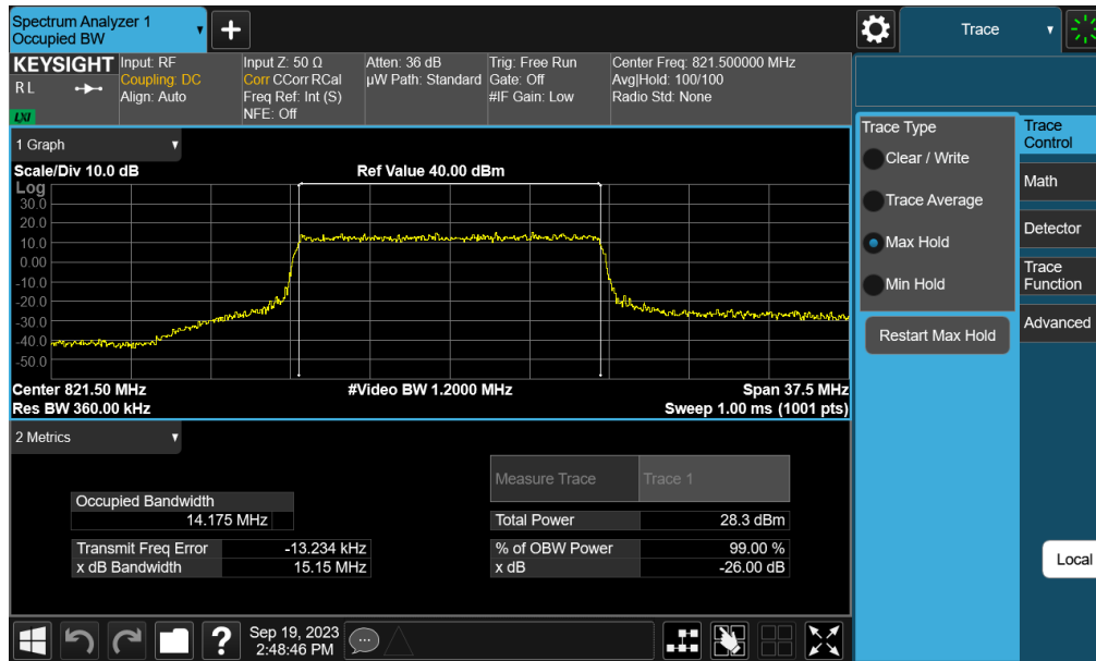
Plot 7-19. Occupied Bandwidth Plot (NR Band n26 - 15MHz QPSK - Full RB Configuration – Ant A)
