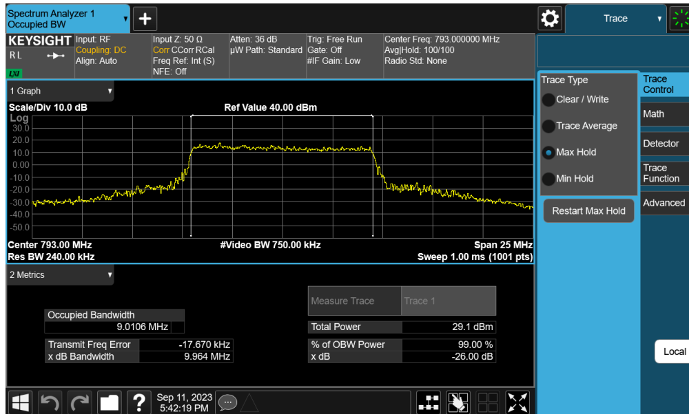
Plot 7-2. Occupied Bandwidth Plot (LTE Band 14 - 10MHz 16-QAM - Full RB Configuration – Ant A)
