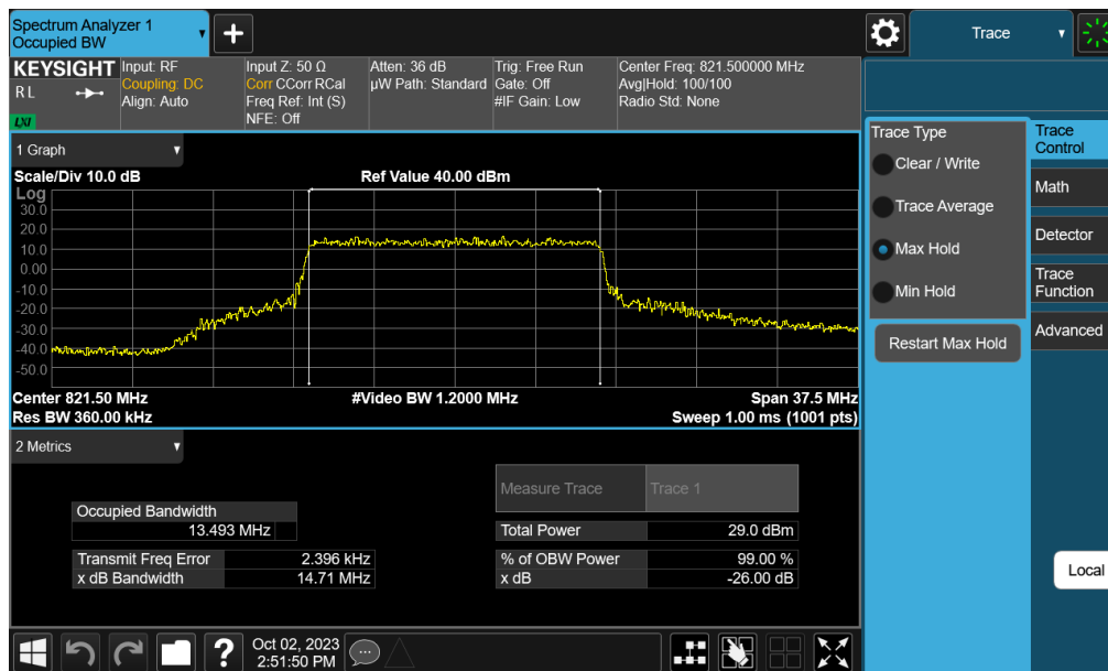
Plot 7-32. Occupied Bandwidth Plot (LTE Band 26 - 15MHz 16-QAM - Full RB Configuration – Ant E)
