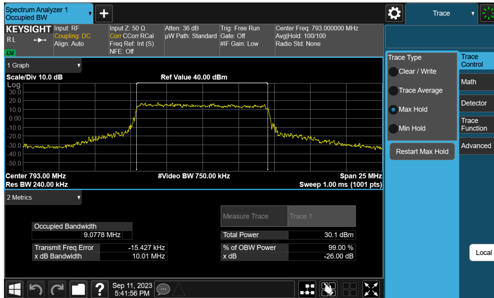
Plot 7-1. Occupied Bandwidth Plot (LTE Band 14 - 10MHz QPSK - Full RB Configuration – Ant A)
