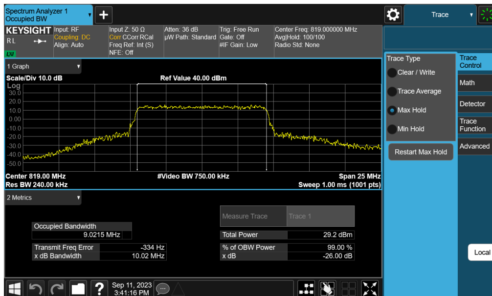
Plot 7-8. Occupied Bandwidth Plot (LTE Band 26 - 10MHz 16-QAM - Full RB Configuration – Ant A)
