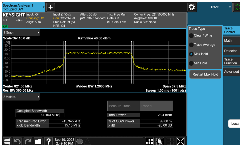
Plot 7-20. Occupied Bandwidth Plot (NR Band n26 - 15MHz 16-QAM - Full RB Configuration – Ant A)
