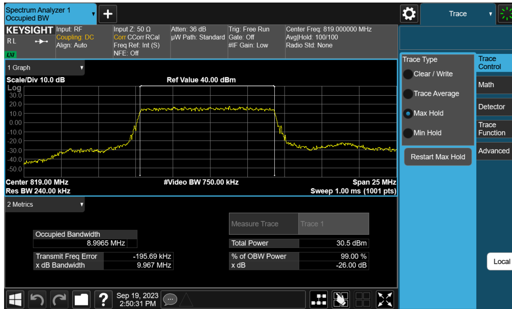
Plot 7-21. Occupied Bandwidth Plot (NR Band n26 - 10MHz \pi/2 BPSK - Full RB Configuration – Ant A)
