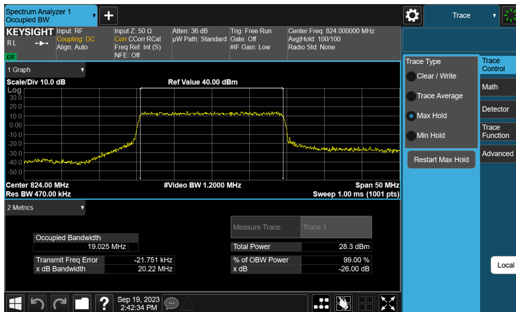
Plot 7-16. Occupied Bandwidth Plot (NR Band n26 - 20MHz QPSK - Full RB Configuration – Ant A)
