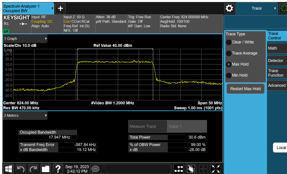
Plot 7-15. Occupied Bandwidth Plot (NR Band n26 - 20MHz \pi/2 BPSK - Full RB Configuration – Ant A)
