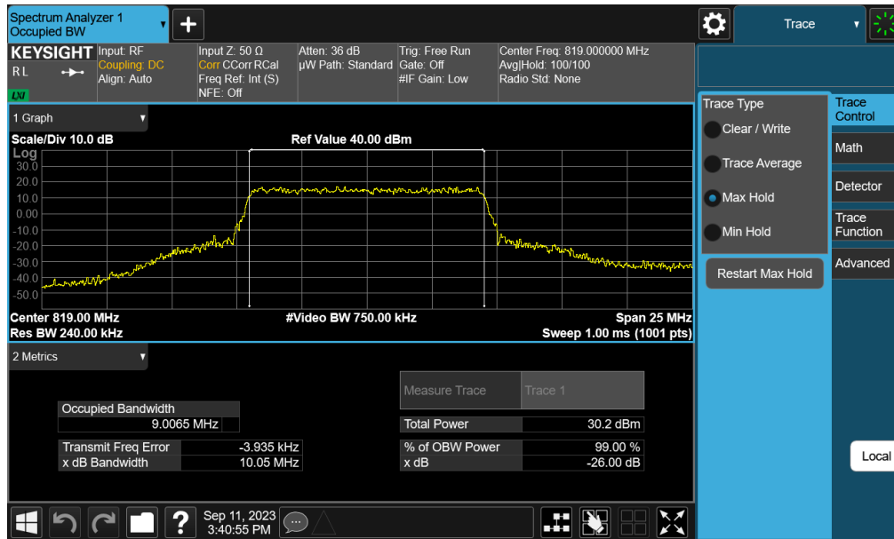
Plot 7-7. Occupied Bandwidth Plot (LTE Band 26 - 10MHz QPSK - Full RB Configuration – Ant A)
