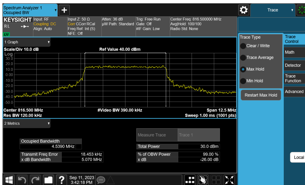
Plot 7-9. Occupied Bandwidth Plot (LTE Band 26 - 5MHz QPSK - Full RB Configuration – Ant A)
