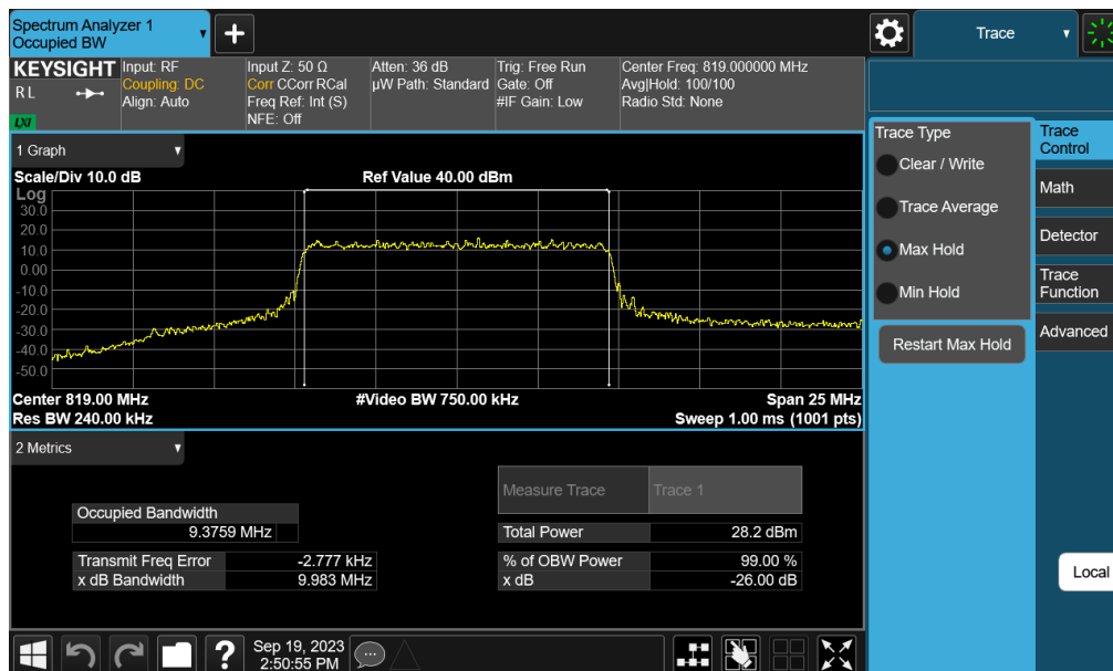
Plot 7-22. Occupied Bandwidth Plot (NR Band n26 - 10MHz QPSK - Full RB Configuration – Ant A)
