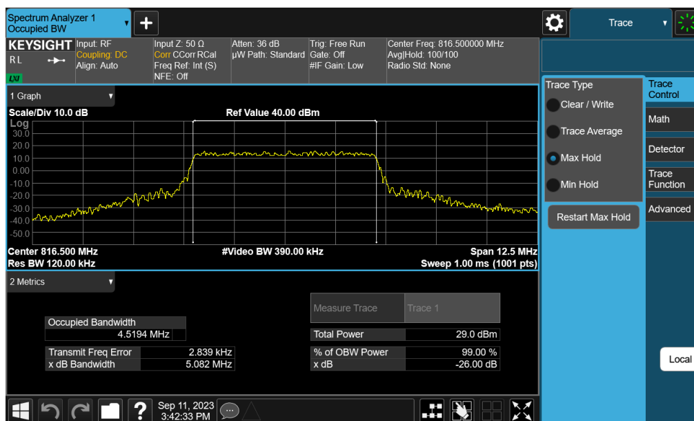
Plot 7-10. Occupied Bandwidth Plot (LTE Band 26 - 5MHz 16-QAM - Full RB Configuration – Ant A)
