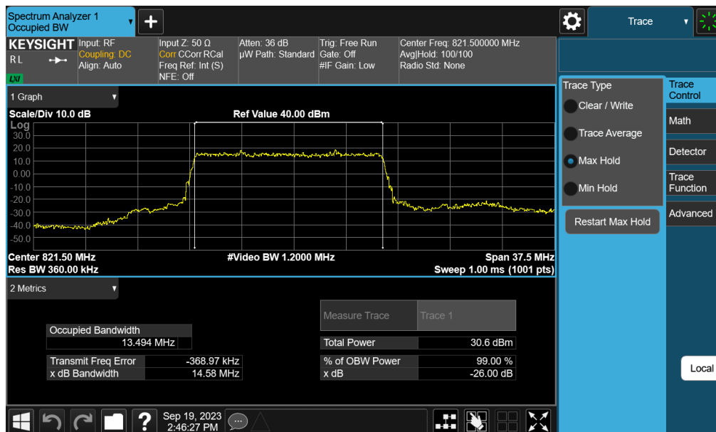
Plot 7-18. Occupied Bandwidth Plot (NR Band n26 - 15MHz \pi/2 BPSK - Full RB Configuration – Ant A)
