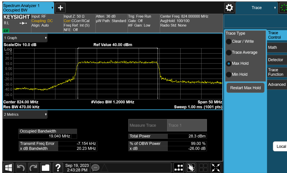
Plot 7-17. Occupied Bandwidth Plot (NR Band n26 - 20MHz 16-QAM - Full RB Configuration – Ant A)
