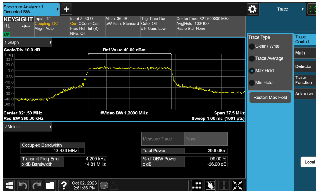
Plot 7-31. Occupied Bandwidth Plot (LTE Band 26 - 15MHz QPSK - Full RB Configuration – Ant E)
