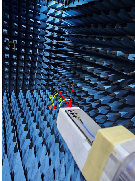
Figure 1: Geometry for SM-S928U for Radiation patterns.
