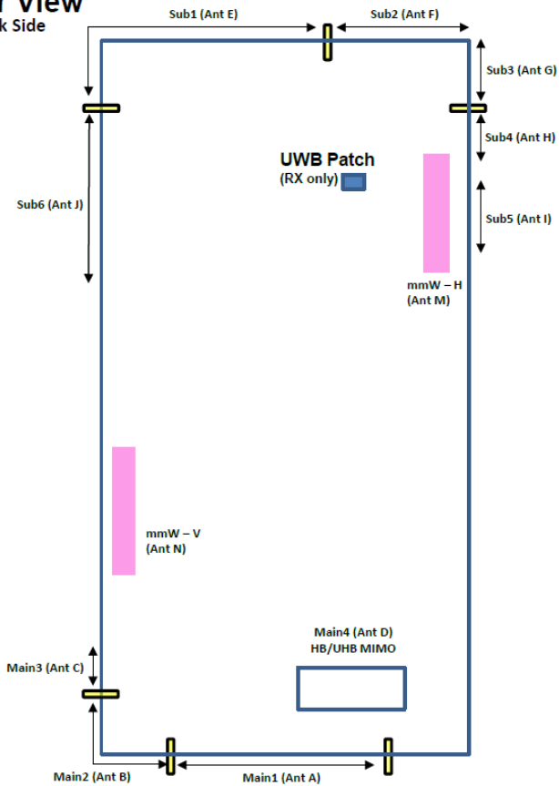
Figure C-1 DUT Antenna Locations
