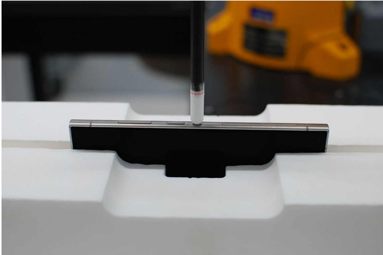
Figure C-3 Near Field Power Density Test Setup Photo – Right Edge at 2 mm
