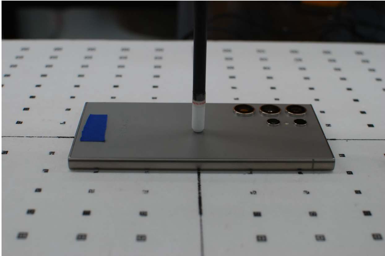
Figure C-3 Near Field Power Density Test Setup Photo – Back Side at 2 mm
