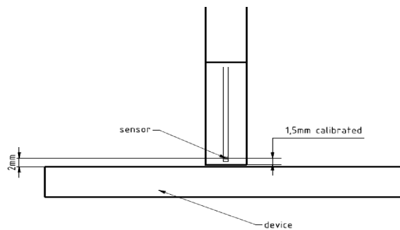
Figure C-2 EUMMWVx Probe
