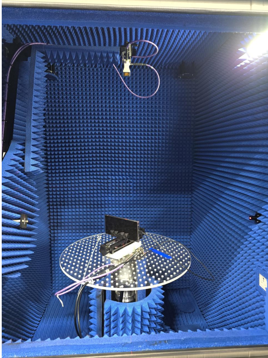
Test Setup Photo 11 – Radiated Power Test Setup (Figure 7-1f)
