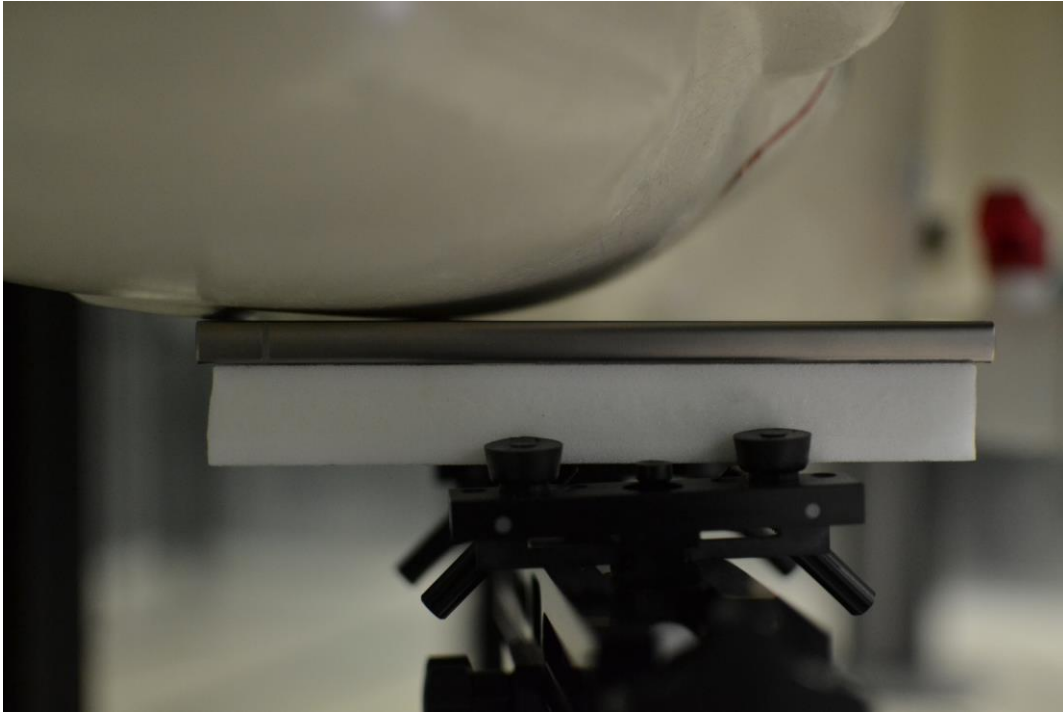
Test Setup Photo 13 – Radiated SAR Right, Cheek
