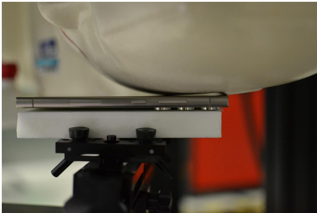
Test Setup Photo 15 – Radiated SAR Left, Cheek
