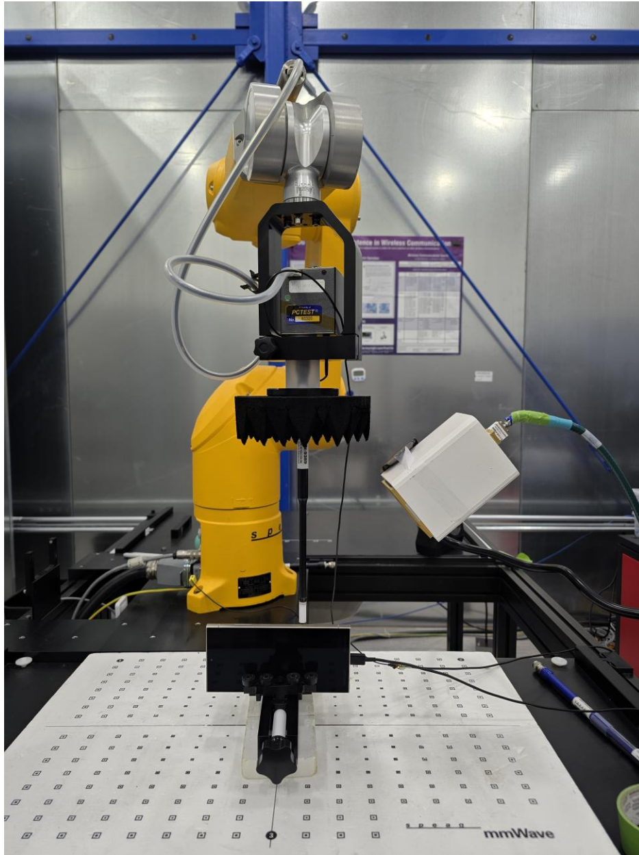
Test Setup Photo 12 – Radiated Power Test Setup (Figure 7-1f)
