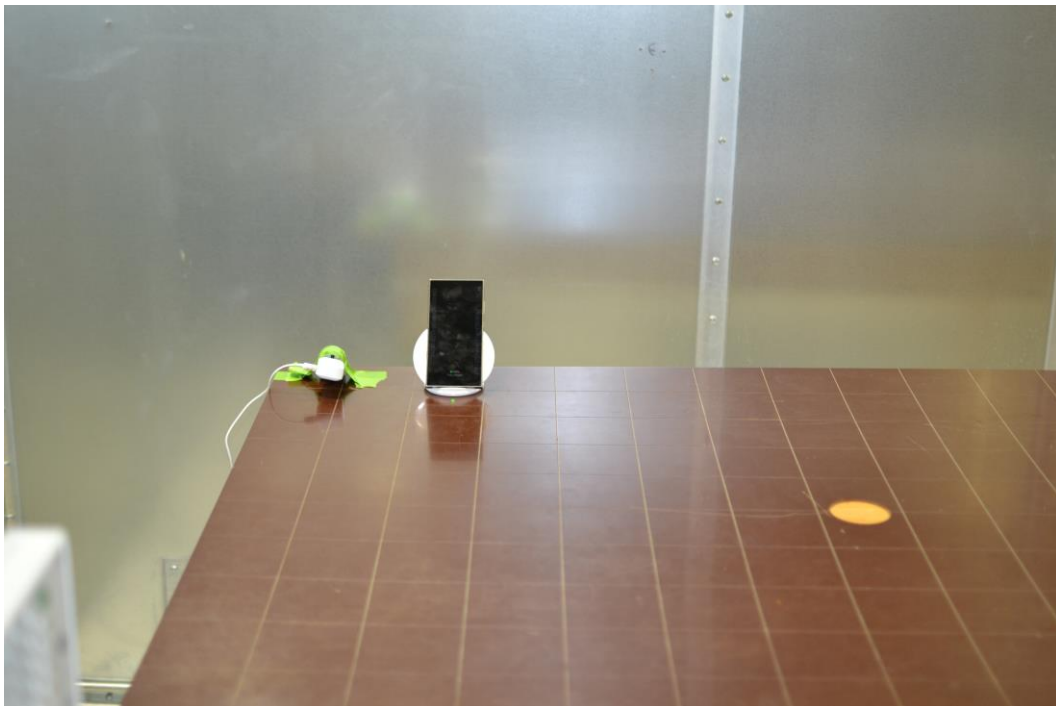
Figure 4. Test Setup – ACLC WCP – <30MHz
