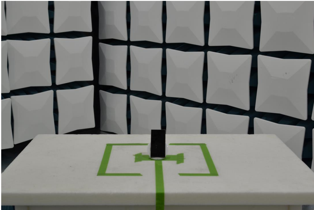
Figure 15. Test Setup – WCP Position – 30MHz-1GHz
