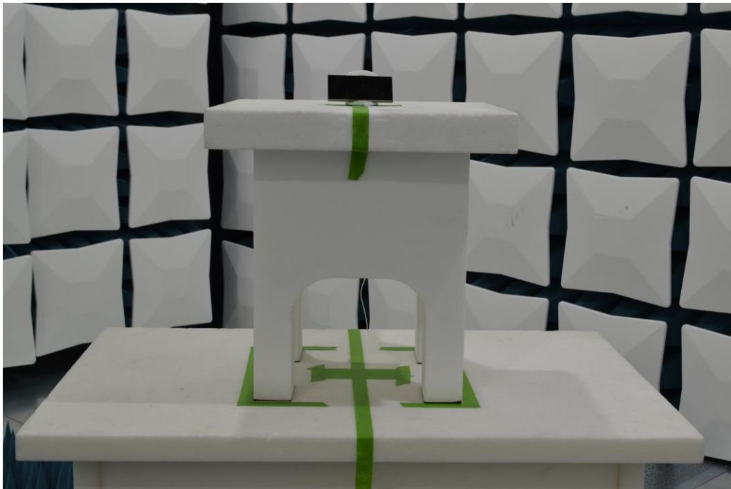
Figure 10. Test Setup – WCP Position – 1GHz-40GHz
