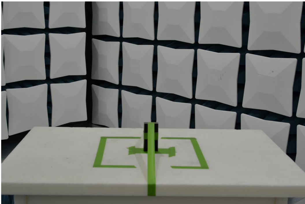
Figure 14. Test Setup – Z Position – 30MHz-1GHz
