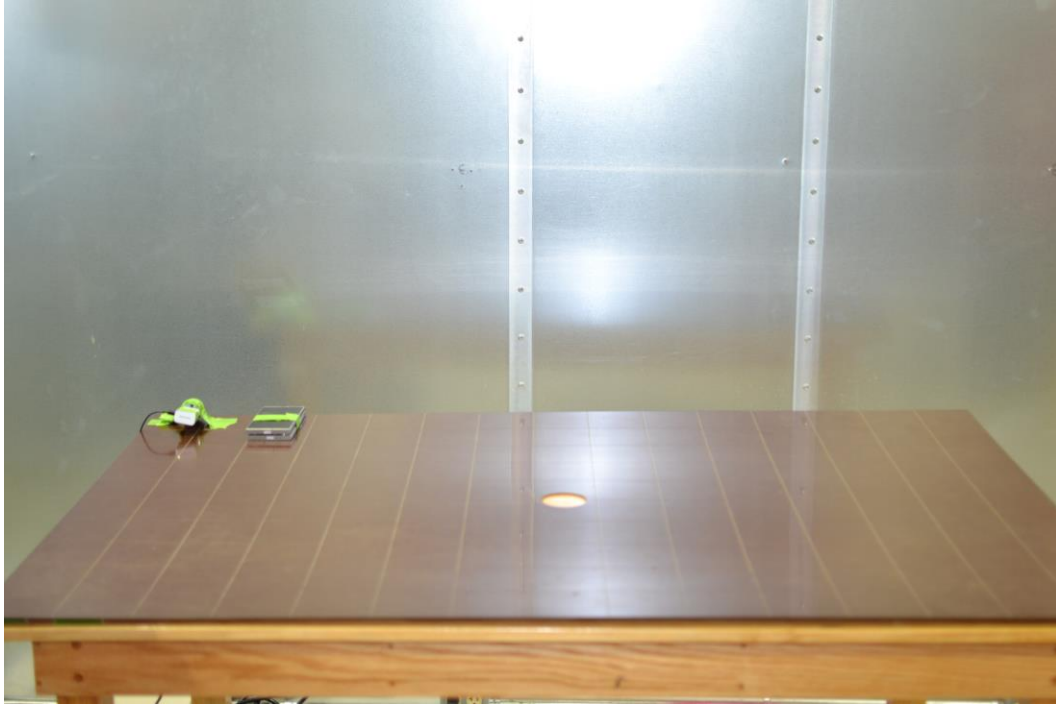
Figure 5. Test Setup – ACLC WPT – <30MHz
