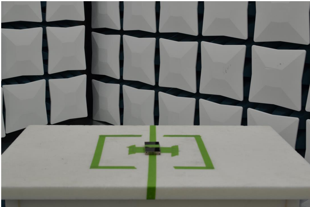
Figure 12. Test Setup – X Position – 30MHz-1GHz
