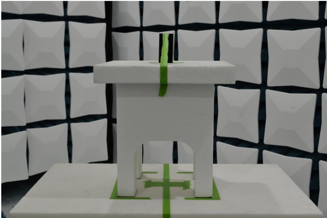
Figure 9. Test Setup – Z Position – 1GHz-40GHz
