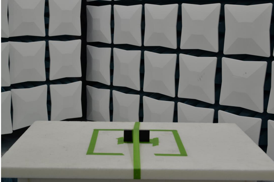
Figure 13. Test Setup – Y Position – 30MHz-1GHz
