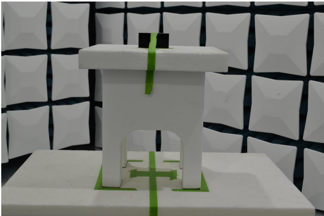
Figure 8. Test Setup – Y Position – 1GHz-40GHz
