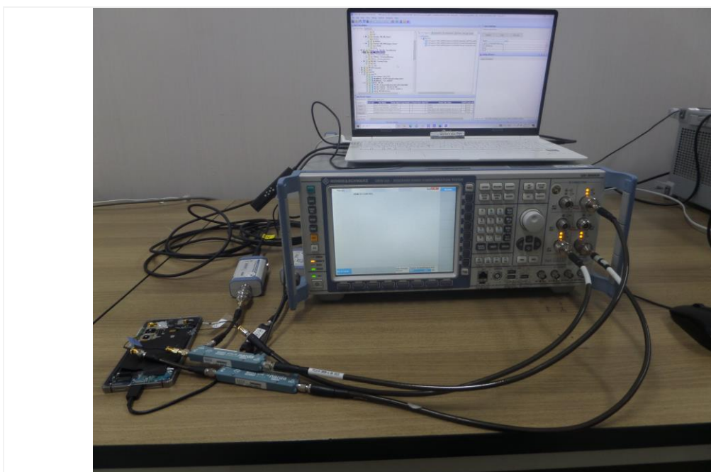
Test setup photo-8 (DBS)
