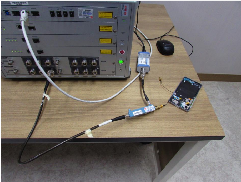
Test setup photo-3 (5G Sub 6)
