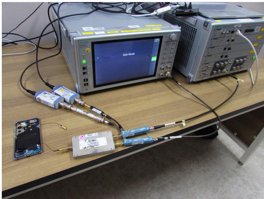
Test setup photo-4 (5G Sub 6 NSA)
