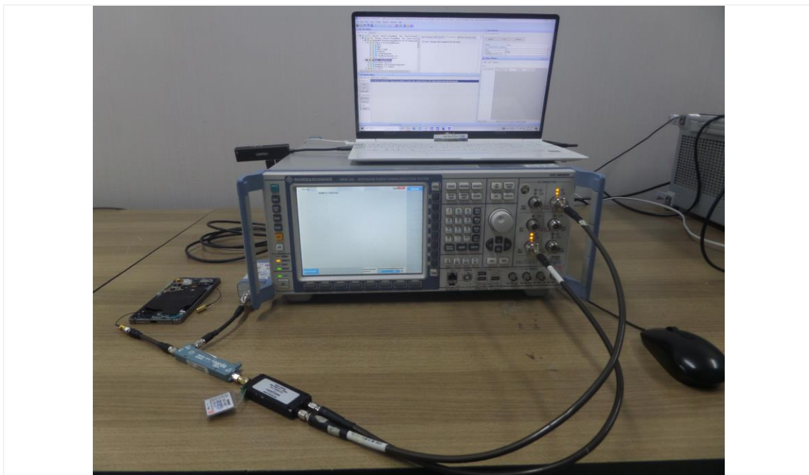
Test setup photo-2 (Legacy)
