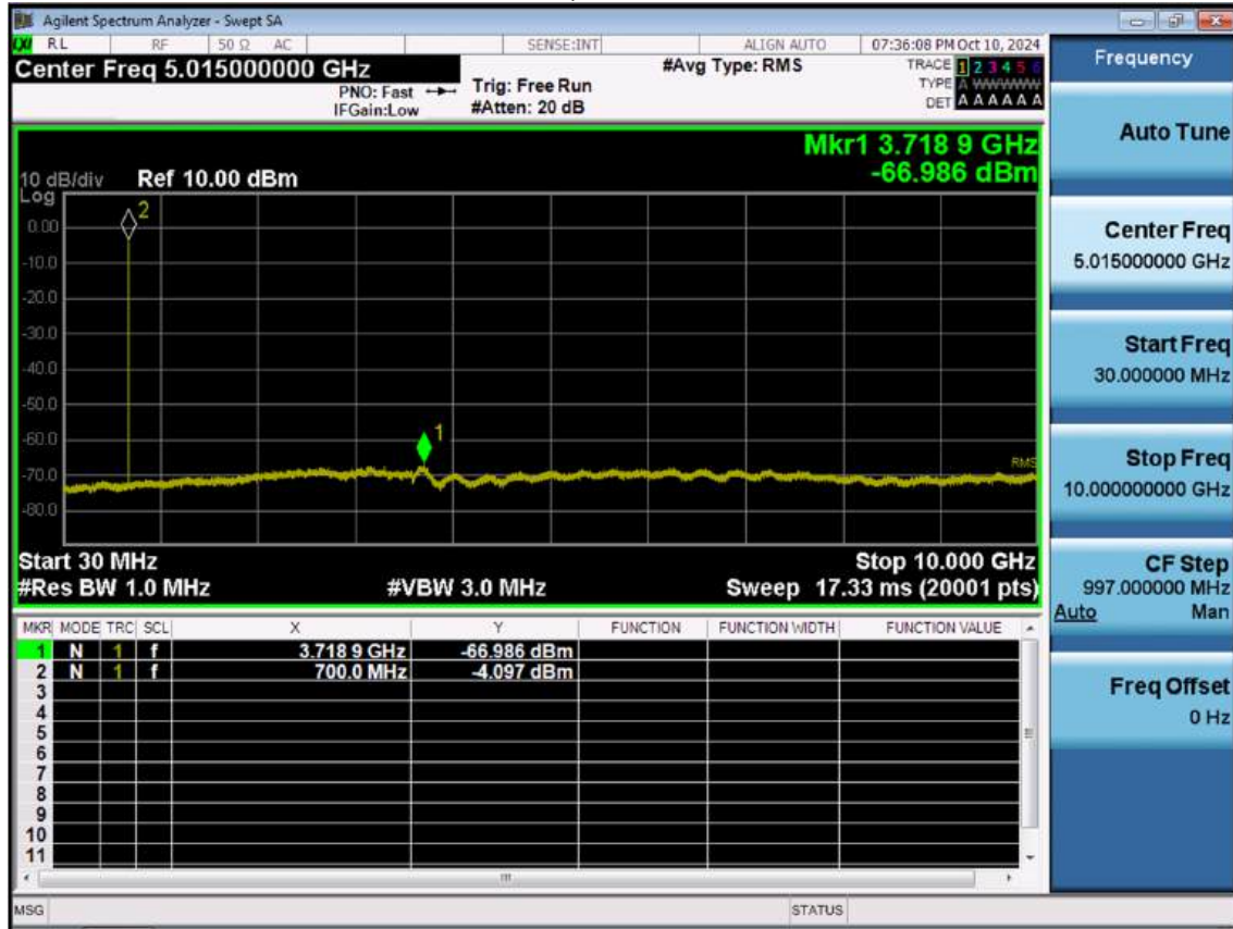
LTE B12_3 M_Conducted Spurious(30 M-10 G)_Low_QPSK_1RB
