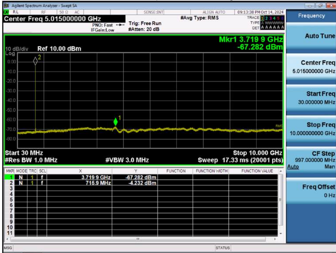
LTE B12_10 M_Conducted Spurious(30 M-10 G)_High_QPSK_1RB
