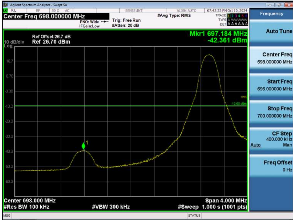
LTE B12_5 M_Band Edge_Low_QPSK_1RB
