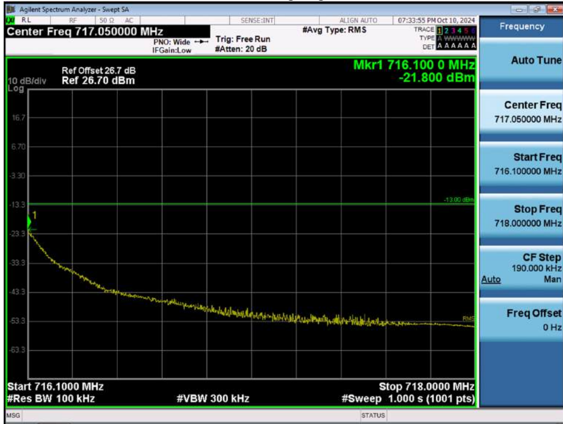
LTE B12_1.4M_Band Edge_High_QPSK_1RB(2)
