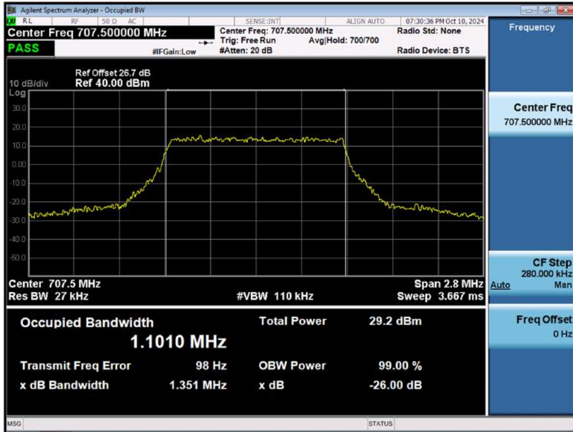
LTE B12_1.4M_OBW_Mid_64QAM_FullRB
