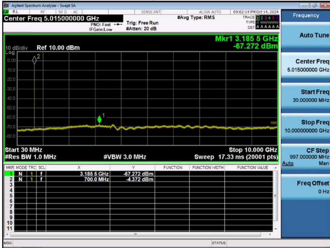
LTE B12_5 M_Conducted Spurious(30 M-10 G)_Low_QPSK_1RB
