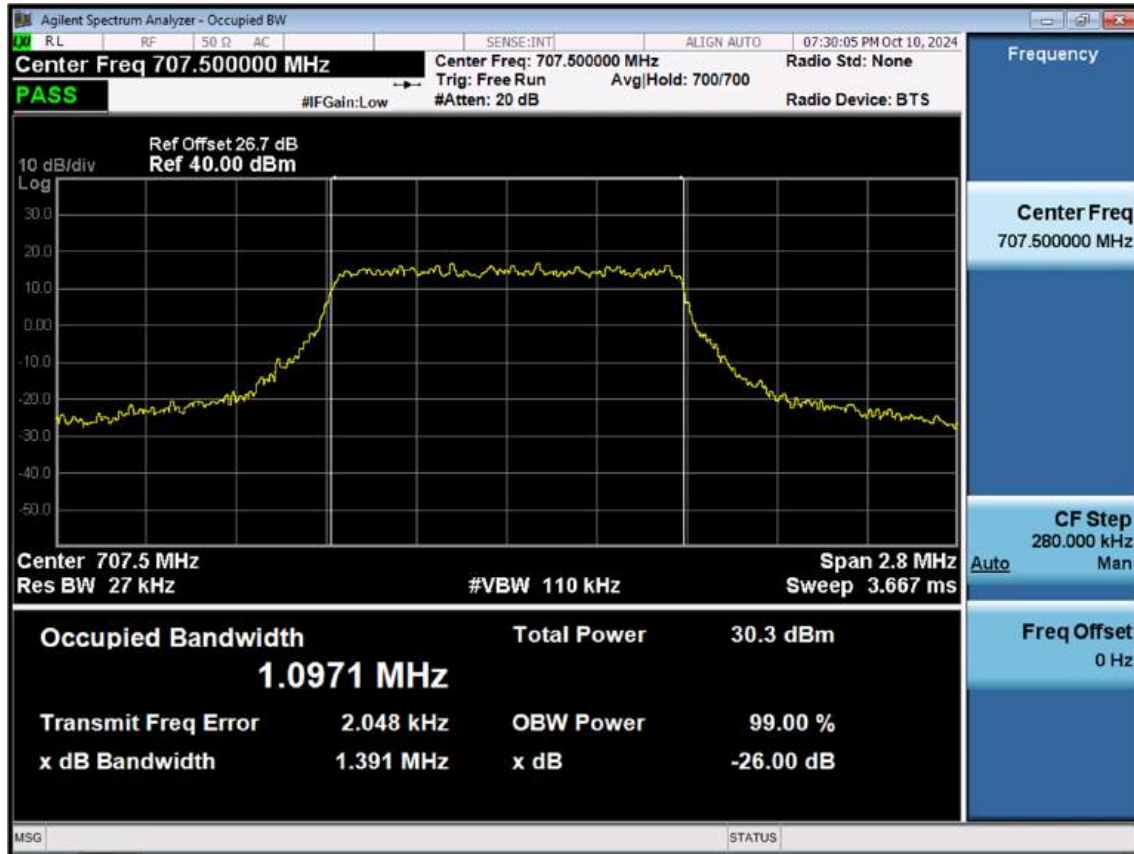
LTE B12_1.4M_OBW_Mid_16QAM_FullRB
