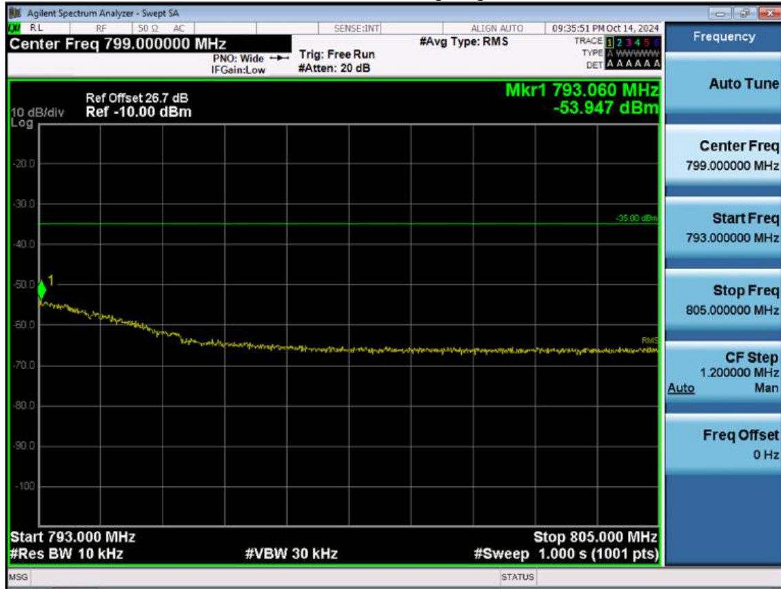
LTE B13_5 M_Extended Band Edge_High_QPSK_FullRB
