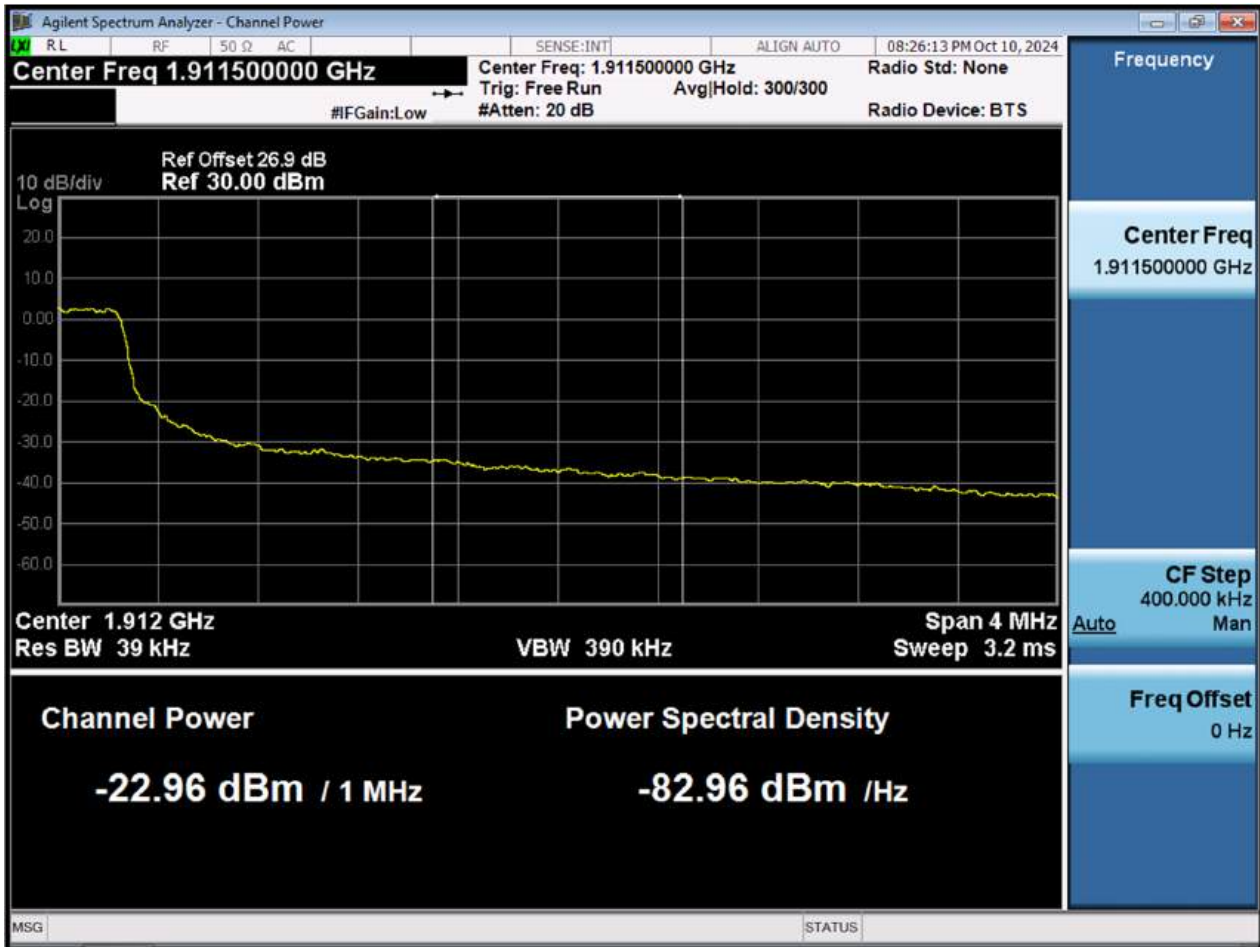
BW5 M_BandEdge_Highest Channel_QPSK_FullRB(2)
