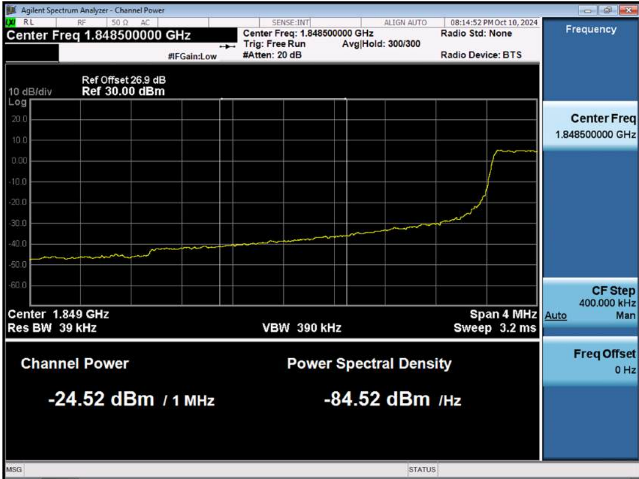
BW3 M_BandEdge_Lowest Channel_QPSK_FullRB(2)
