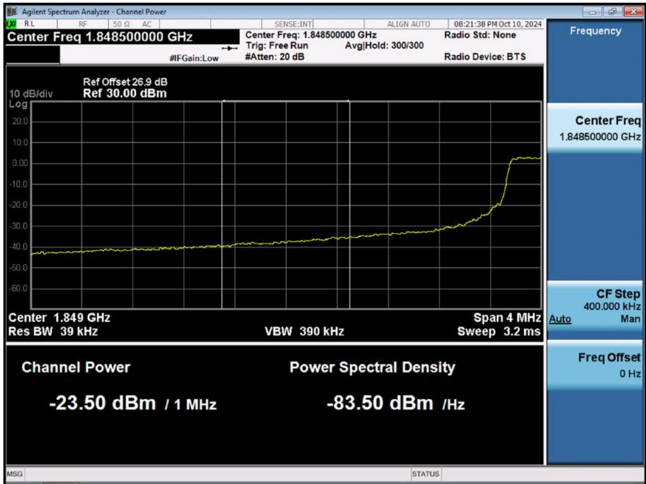
BW5 M_BandEdge_Lowest Channel_QPSK_FullRB(2)
