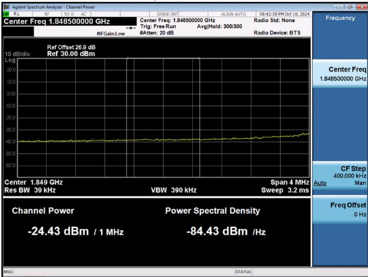
BW20 M_BandEdge_Lowest Channel_QPSK_FullRB(2)
