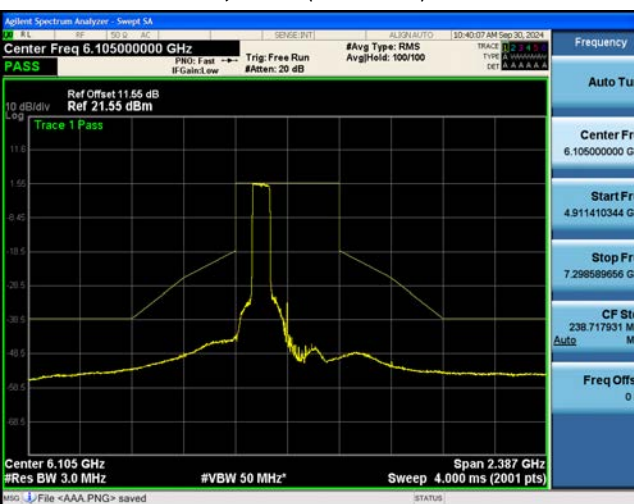
Bandwidth 320M, Ch. 31(6105 MHz) 996 Tones 67 RU
