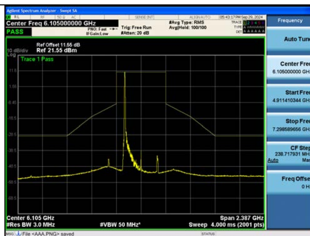
Bandwidth 320M, Ch. 31(6105 MHz) 242 Tones 61 RU
