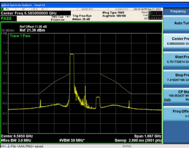
Bandwidth 320M, Ch. 127(6585 MHz)484 Tones 65 RU
