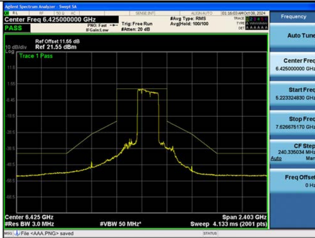
Bandwidth 320M, Ch. 95(6425 MHz) 3x996T+484T RU105
