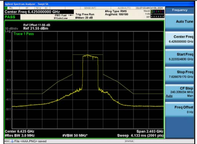
Bandwidth 320M, Ch. 95(6425 MHz) 3x996T RU104
