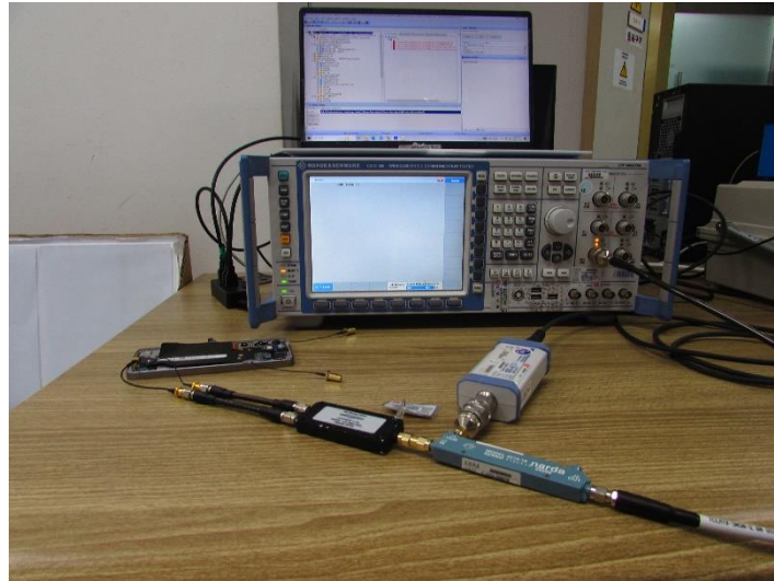
Test setup photo-2 (8-1(b) (Legacy))
