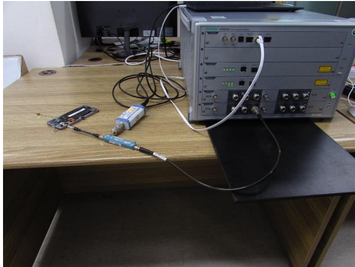
Test setup photo-3 (8-1(c) 5G Sub 6 SA)
