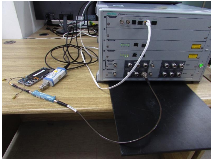
Test setup photo-1 (8-1(a) 5G Sub 6)
