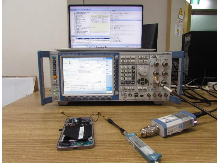
Test setup photo-1 (8-1(a) Legacy)
