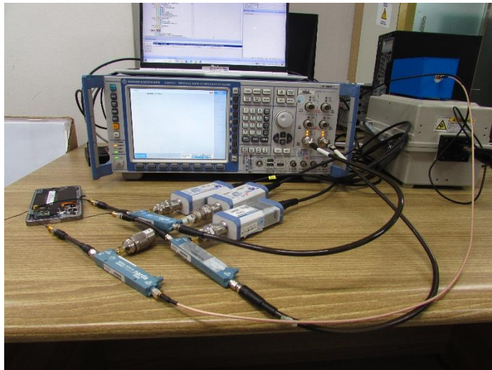
Test setup photo-2 (8-1(f) (System level compliance))
