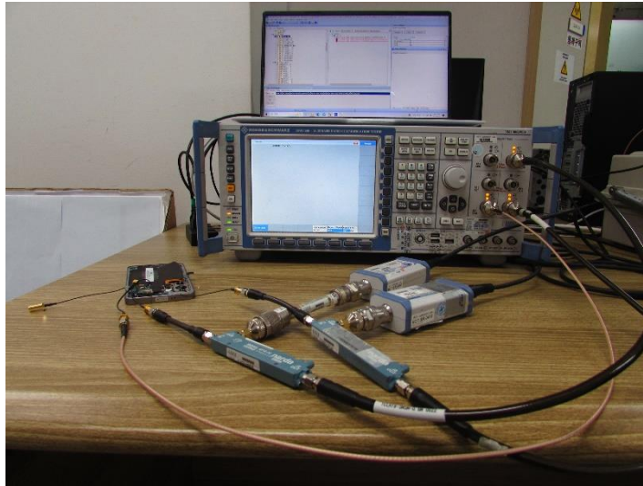
Test setup photo-2 (8-1(e) (WLAN DBS))
