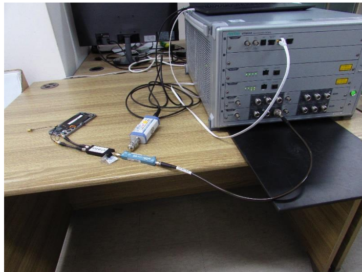
Test setup photo-2 (8-1(b) 5G Sub 6 NSA)
