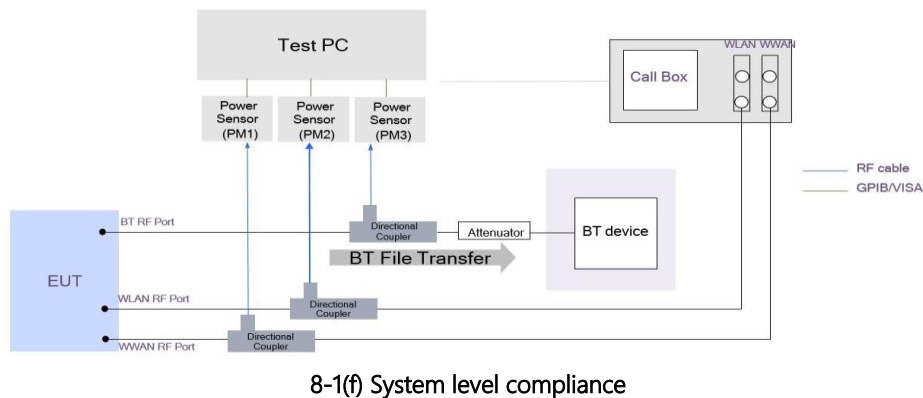
Figure 8-1 Conducted power measurement setup
