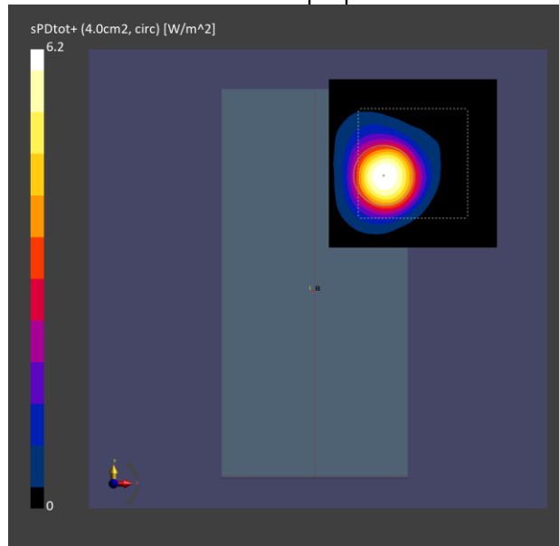
Figure 9-2: 4cm2 psPD distribution measured at input.power.limit of 12.3 dBm for n261 Beam 257
