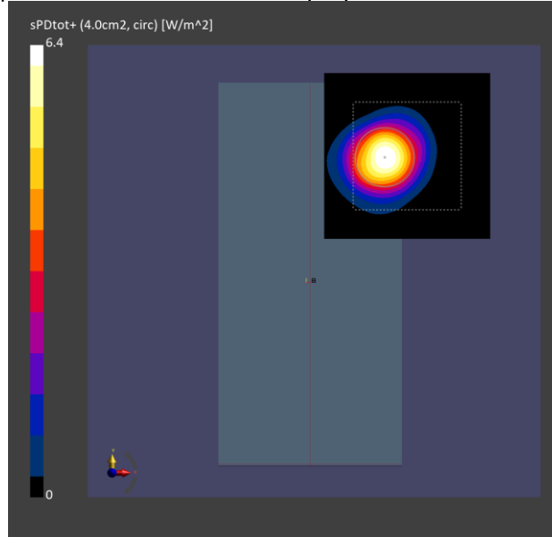
Figure 9-1: 4cm2 psPD distribution measured at input.power.limit of 5.3 dBm for n261 Beam 271
