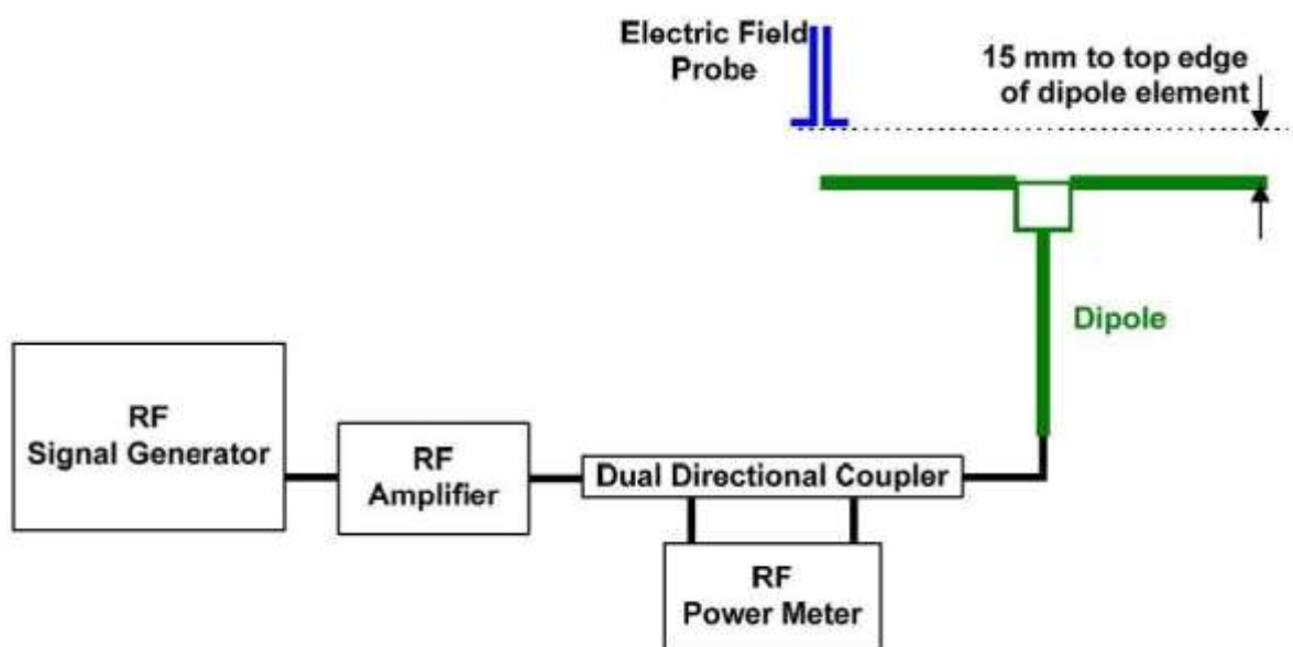
Setup diagram
