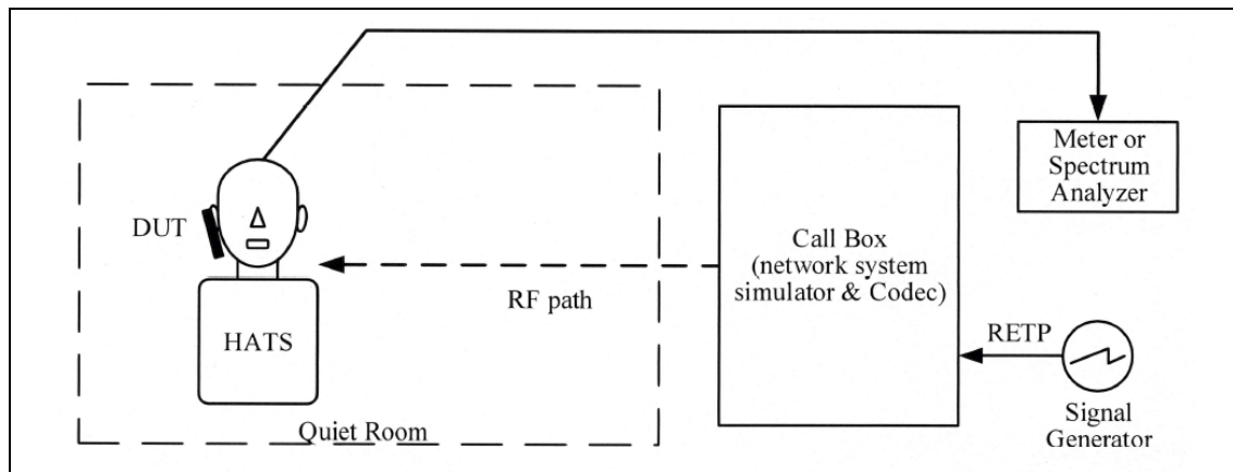
Figure 1. Volume Control Test Set-up
