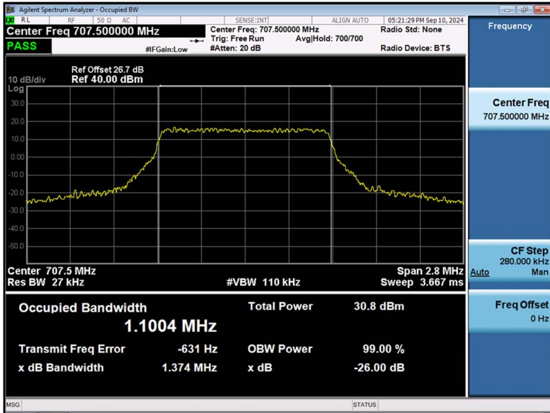
LTE B12_1.4M_OBW_Mid_16QAM_FullRB
