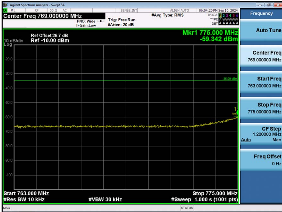
LTE B13_5 M_Extended Band Edge_Low_QPSK_FullIRB
