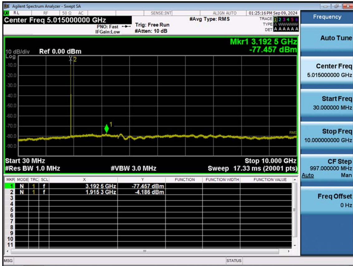
LTE B25_5 M_Conducted Spurious(30 M-10 G)_High_QPSK_1RB
