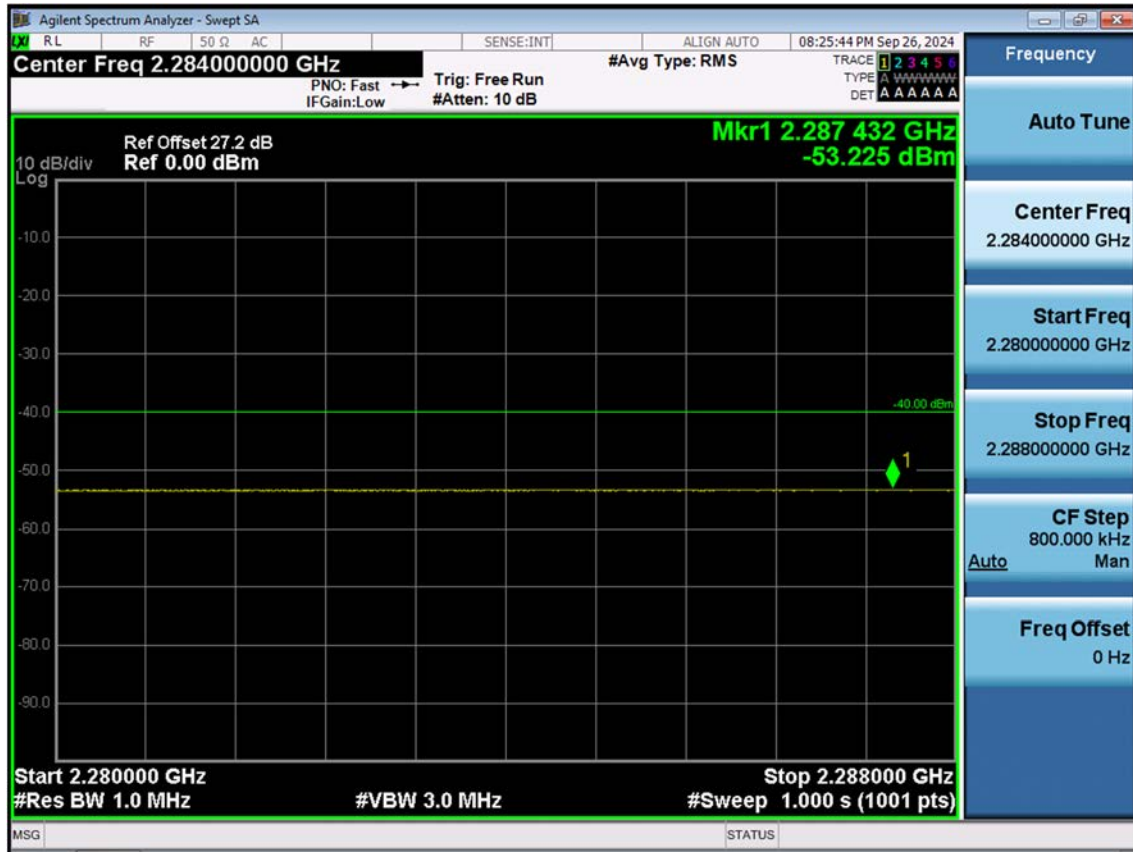
LTE B30_5 M_Band Edge(2280MHz-2288MHz)_Mid_QPSK_FullRB
