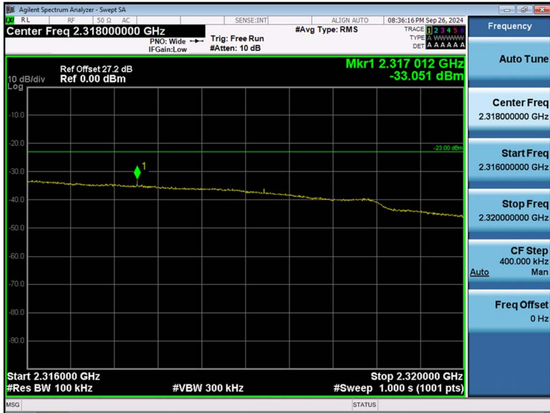
LTE B30_5 M_Band Edge(2316MHz-2320MHz)_High_QPSK_FullRB
