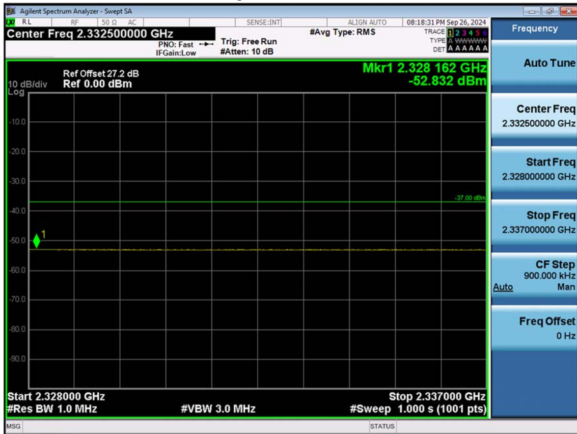
LTE B30_5 M_Band Edge(2328MHz-2337MHz)_Low_QPSK_FullIRB
