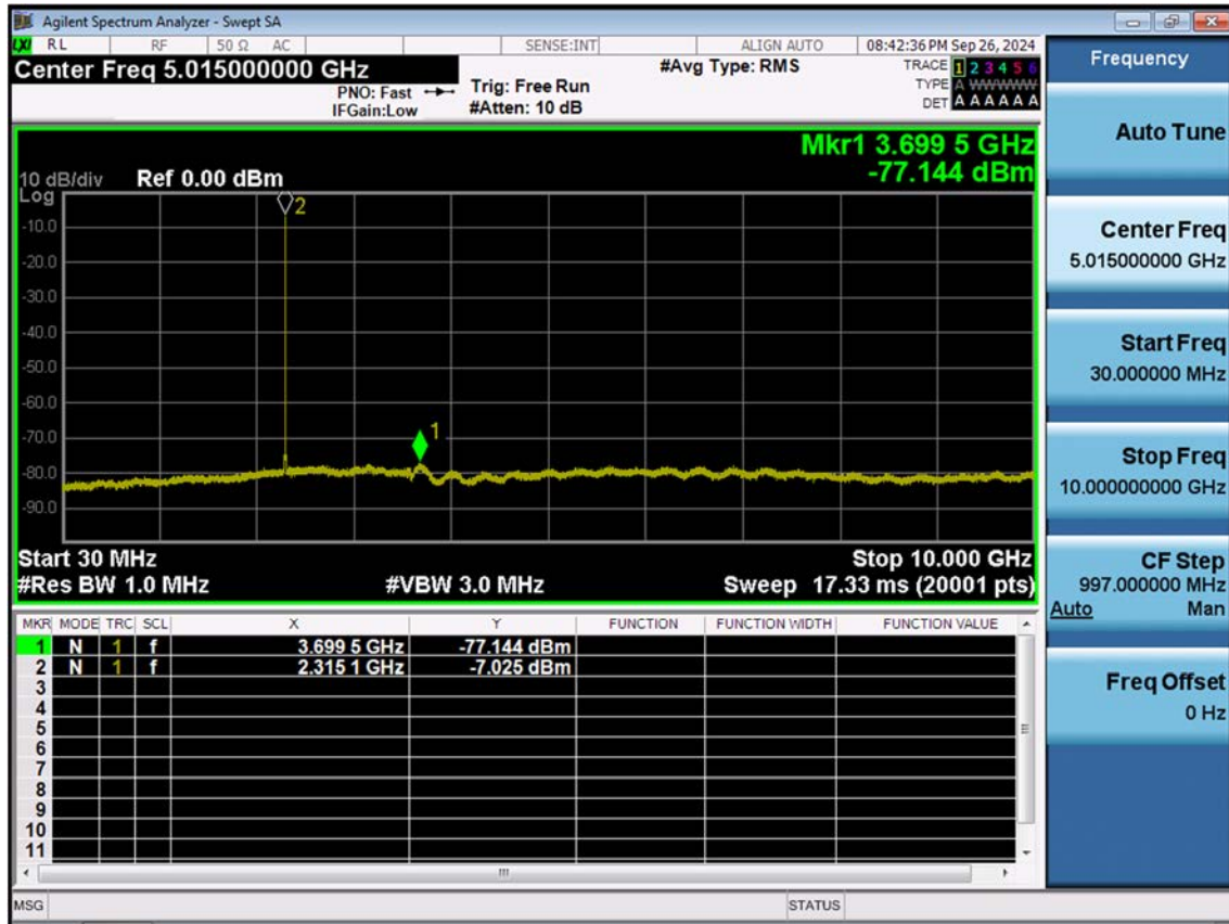
LTE B30_5 M_Conducted Spurious(30 M-10 G)_High_QPSK_1RB
