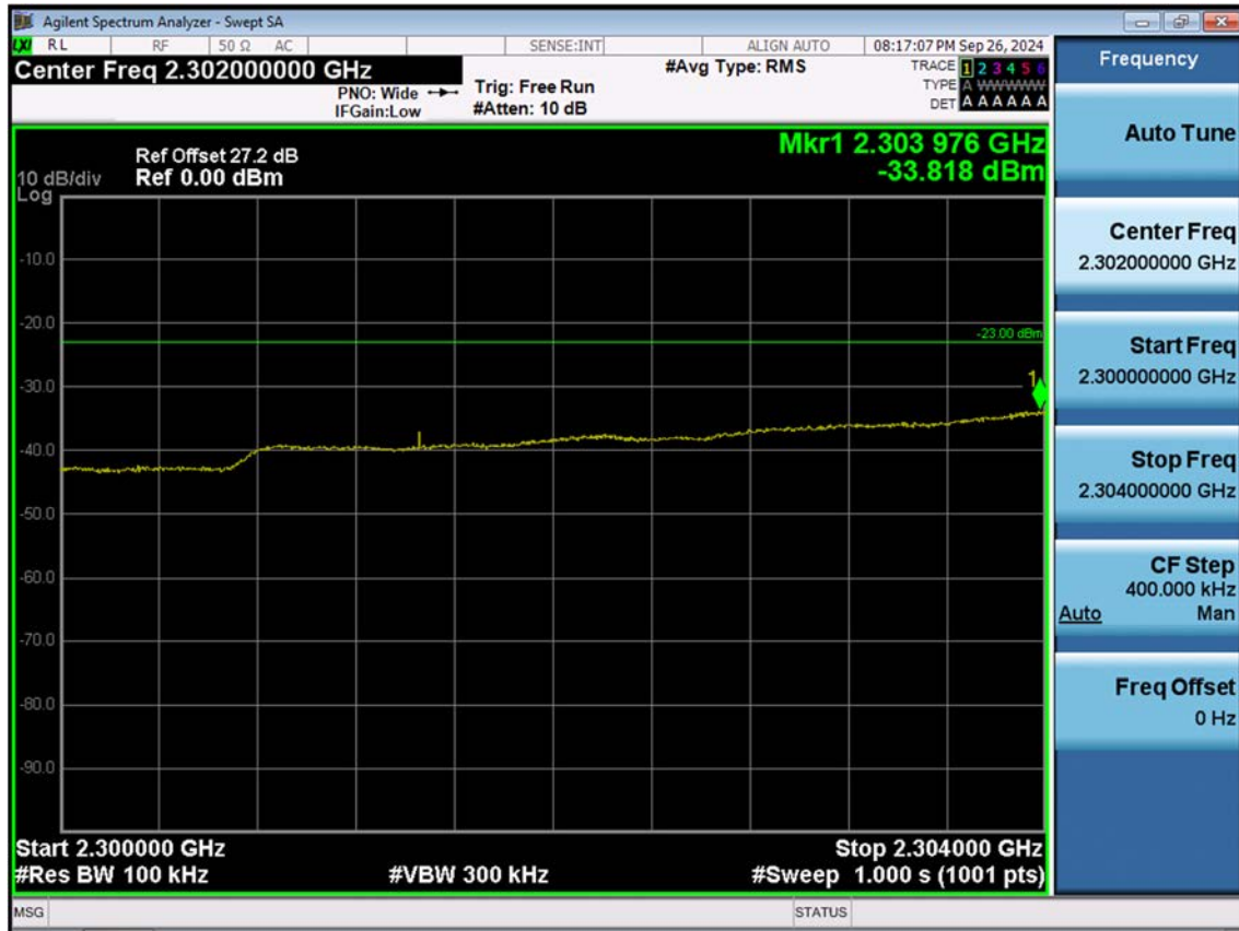
LTE B30_5 M_Band Edge(2300MHz-2304MHz)_Low_QPSK_FullIRB
