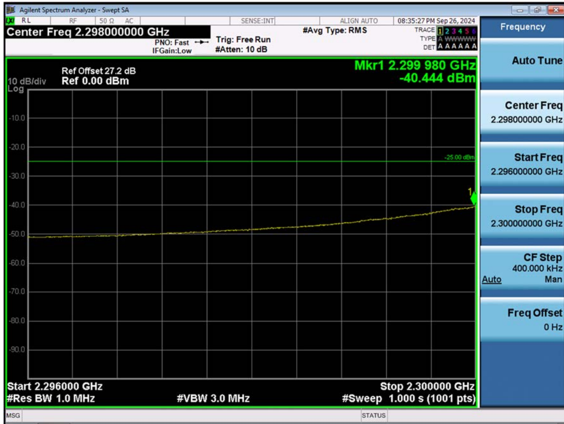
LTE B30_5 M_Band Edge(2296MHz-2300MHz)_High_QPSK_FullRB
