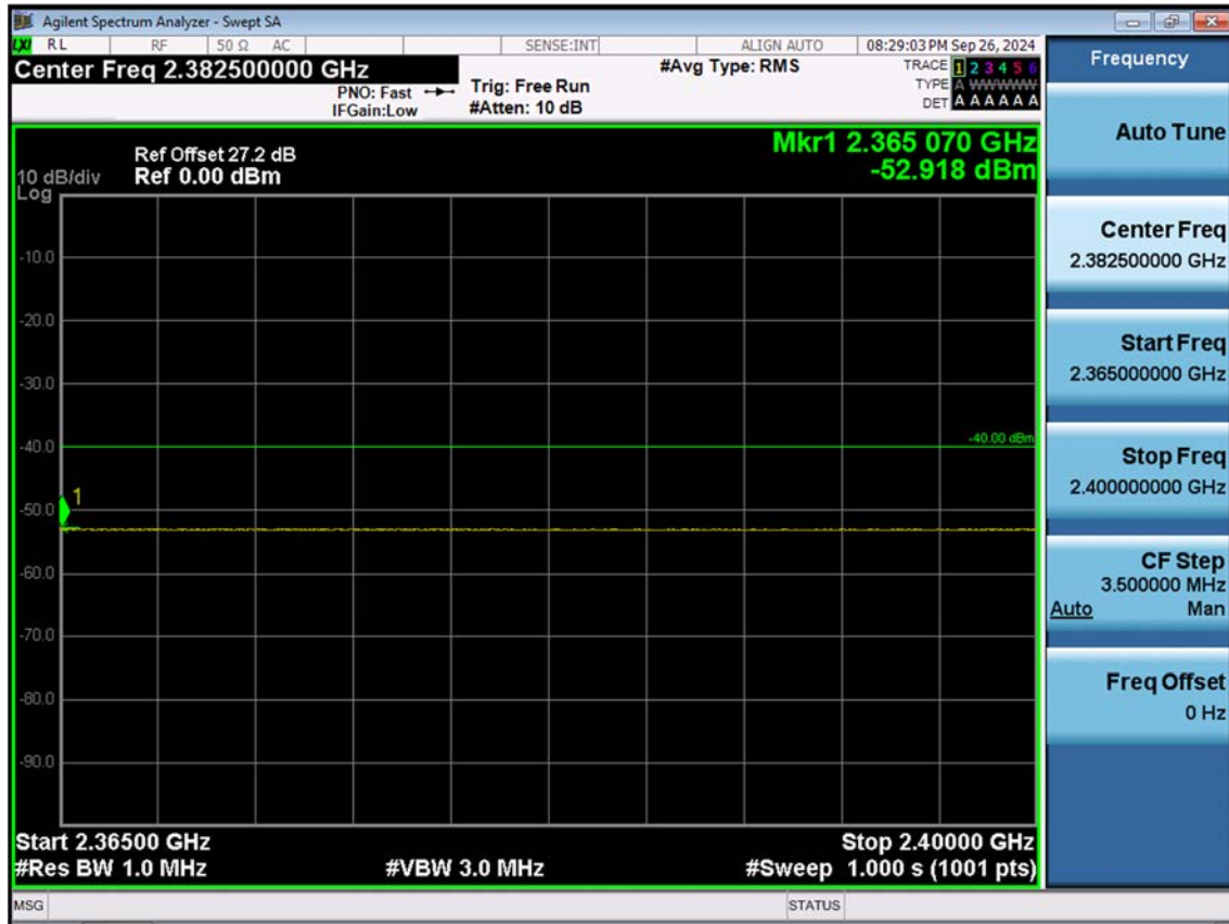
LTE B30_5 M_Band Edge(2365MHz-2400MHz)_Mid_QPSK_FullIRB
