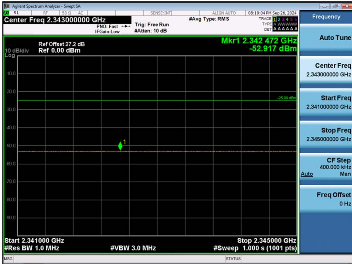
LTE B30_5 M_Band Edge(2341MHz-2345MHz)_Low_QPSK_FullIRB
