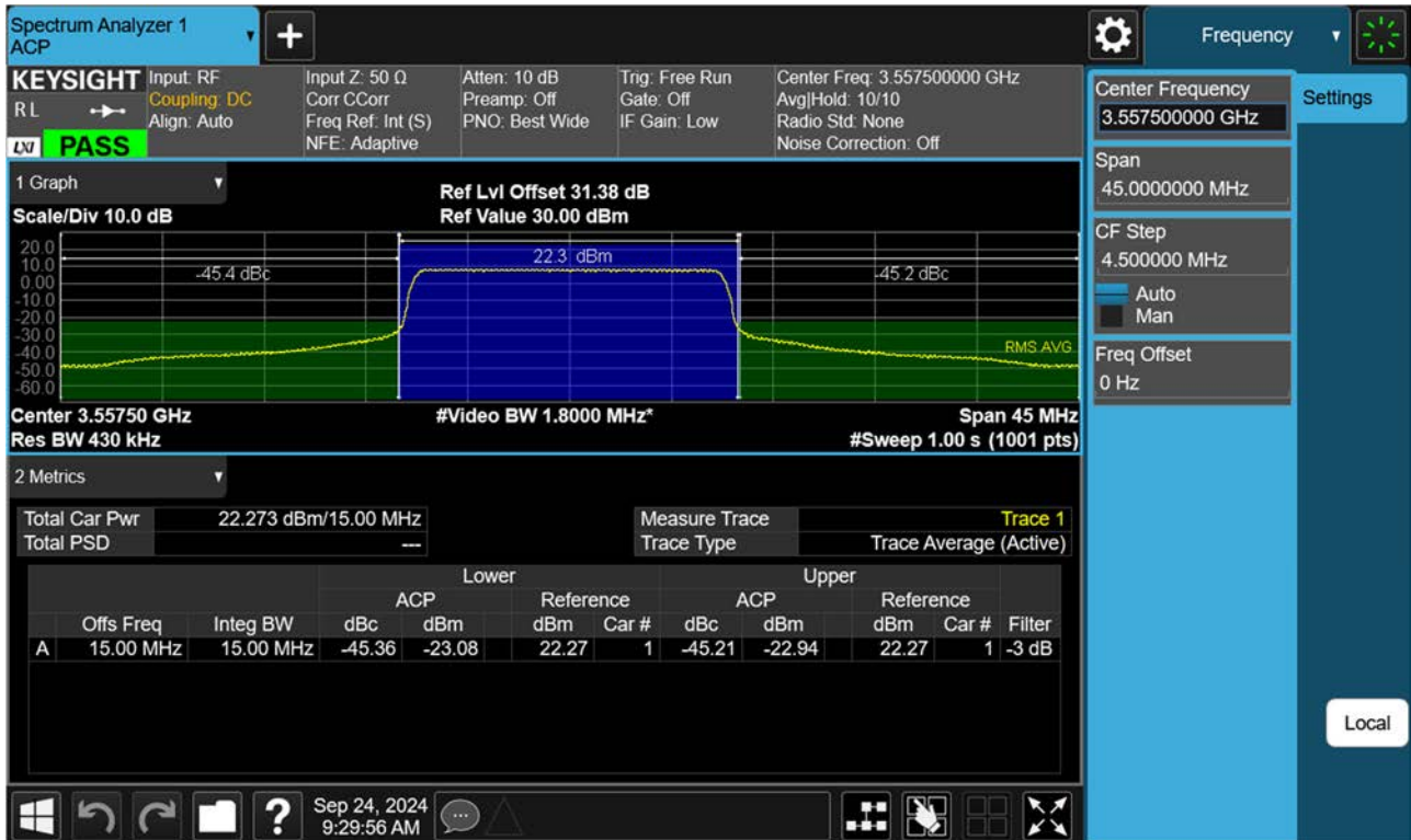
BAND 48. Adjacent Channel Leakage Ratio(ACLR) Plot (15 MHz Ch.55315 QPSK RB 75, Offset 0)
