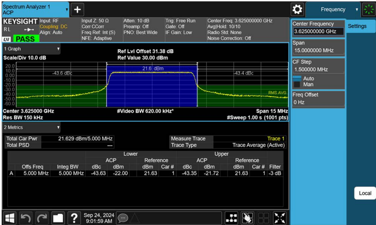
BAND 48. Adjacent Channel Leakage Ratio(ACLR) Plot (5 MHz Ch.55990 QPSK RB 25, Offset 0)
