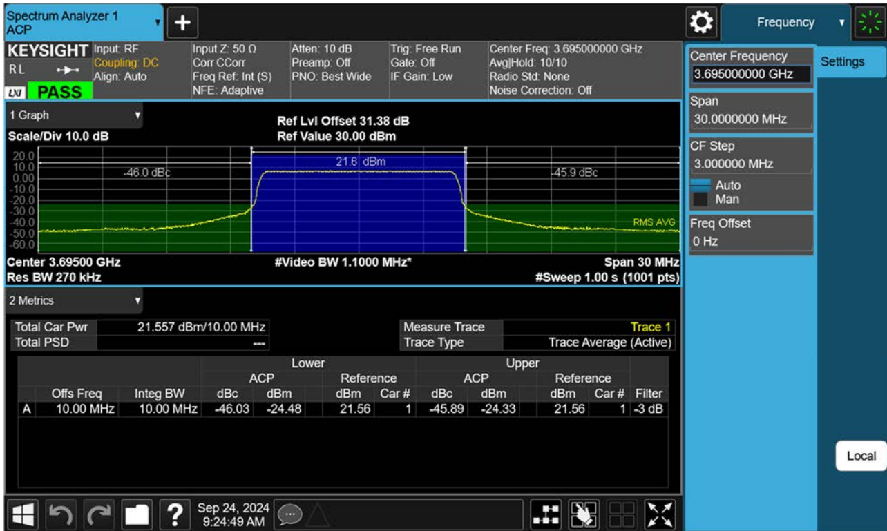
BAND 48. Adjacent Channel Leakage Ratio(ACLR) Plot (10 MHz Ch. 56690 QPSK RB 50, Offset 0)
