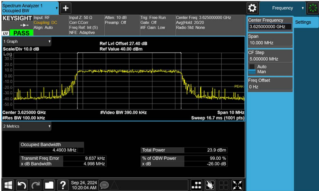
BAND 48. Occupied Bandwidth Plot (5 MHz Ch.55990 256-QAM RB 25)
