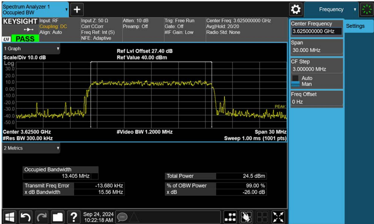
BAND 48. Occupied Bandwidth Plot (15 MHz Ch.55990 64-QAM RB 75)
