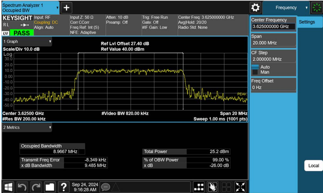
BAND 48. Occupied Bandwidth Plot (10 MHz Ch.55990 16-QAM RB 50)
