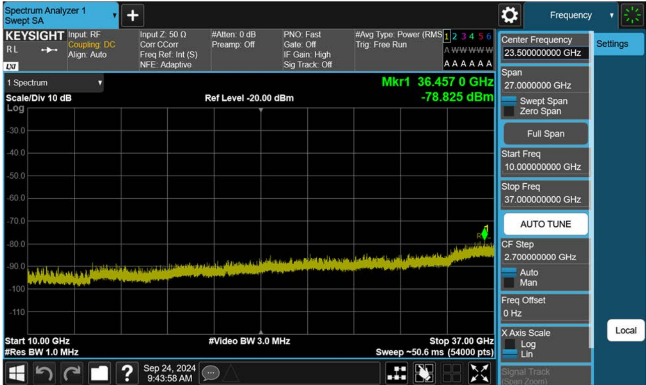
BAND 48. Conducted Spurious Plot 2 (15 MHz Ch. 56665 QPSK RB 1, Offset 0)
