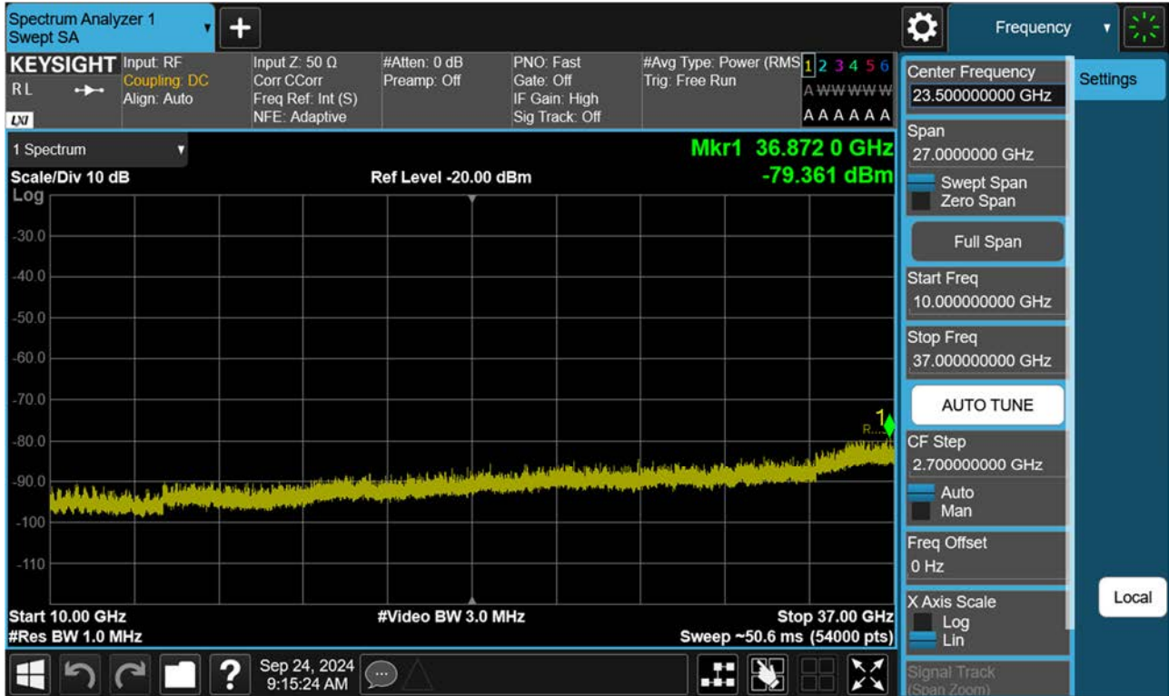
BAND 48. Conducted Spurious Plot 2 (10 MHz Ch. 55290 QPSK RB 1, Offset 0)
