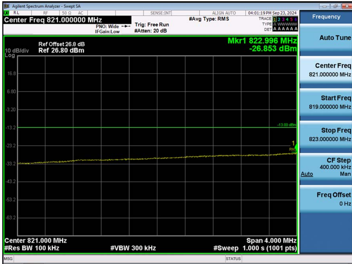
LTE B5_10 M_Extended Band Edge_Low_QPSK_FullIRB
