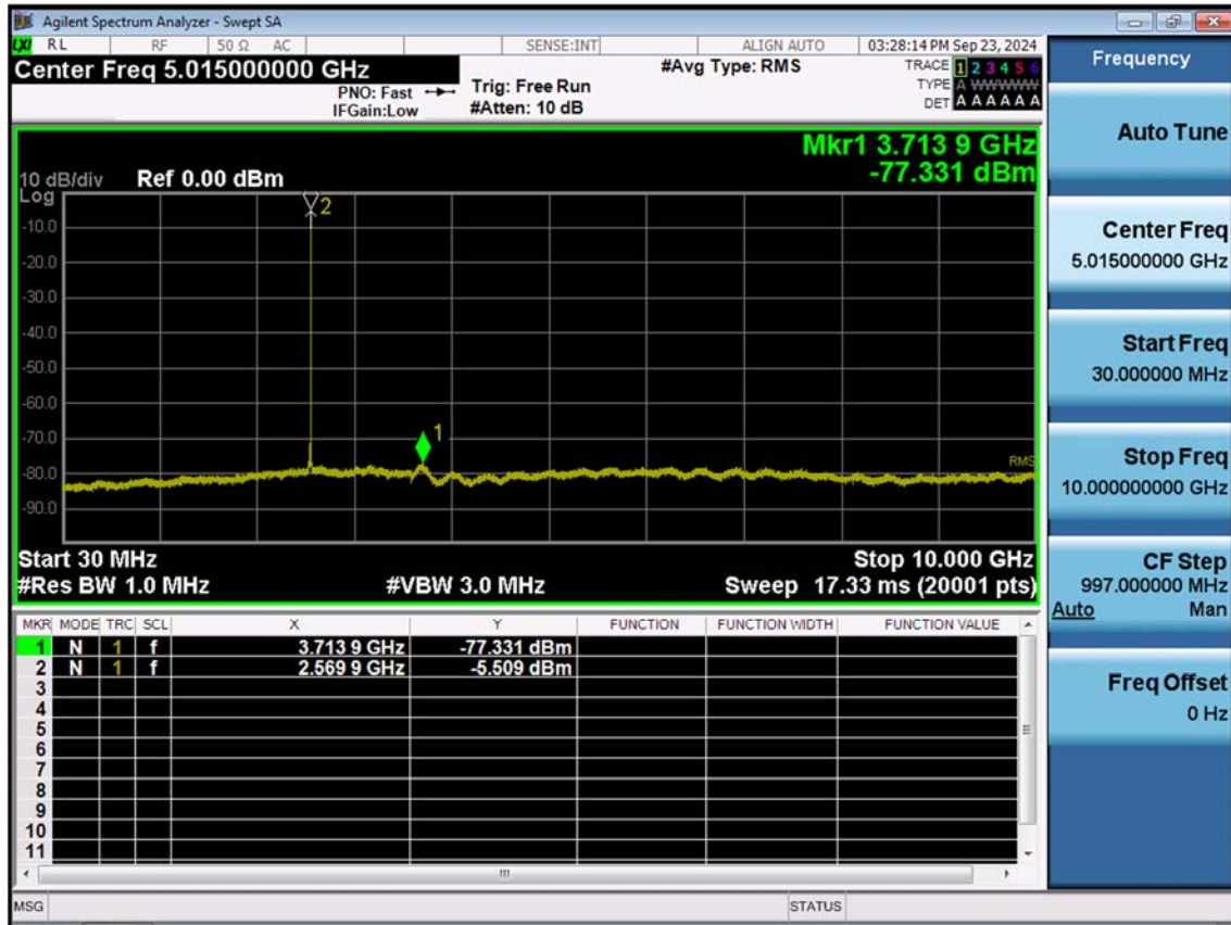
LTE B7_15 M_Conducted Spurious(30 M-10 G)_High_QPSK_1RB
