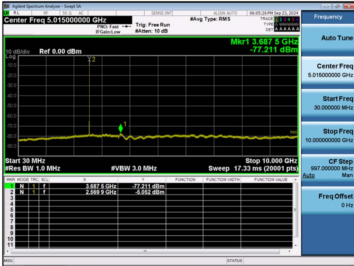
LTE B7_10 M_Conducted Spurious(30 M-10 G)_High_QPSK_1RB
