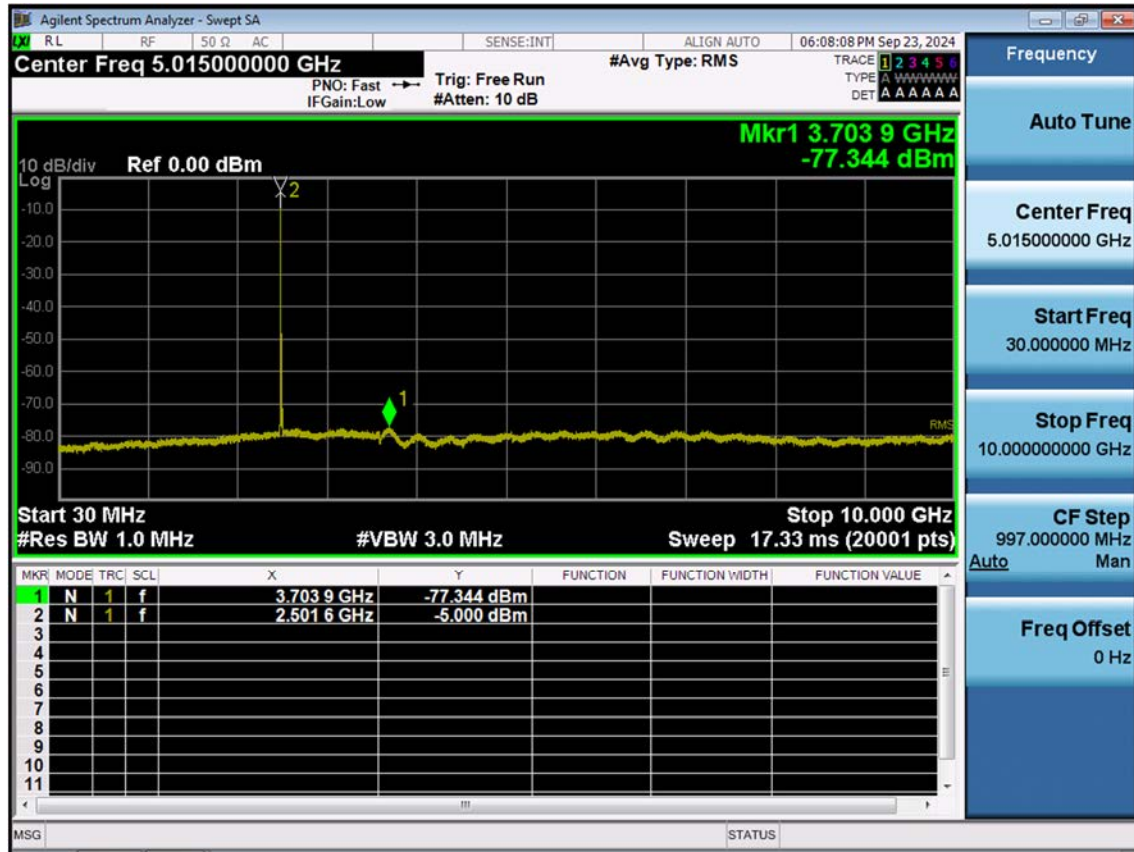
LTE B7_15 M_Conducted Spurious(30 M-10 G)_Low_QPSK_1RB
