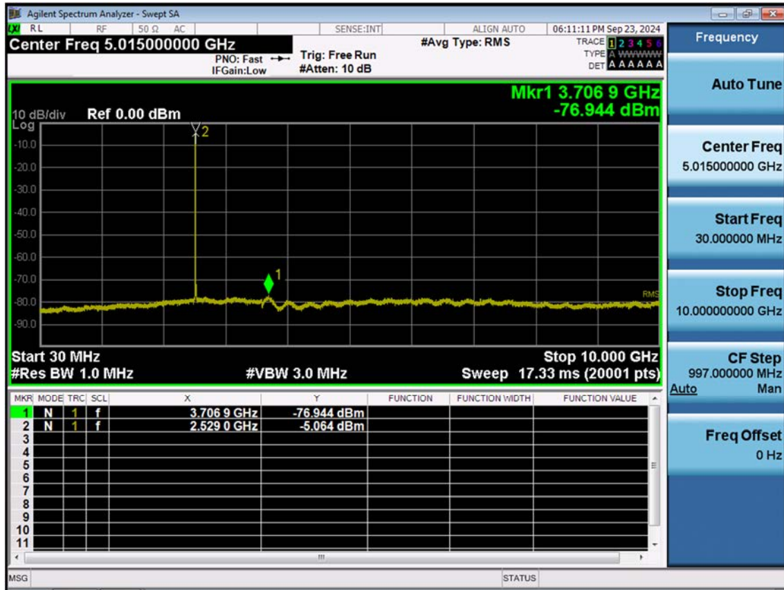
LTE B7_15 M_Conducted Spurious(30 M-10 G)_Mid_QPSK_1RB
